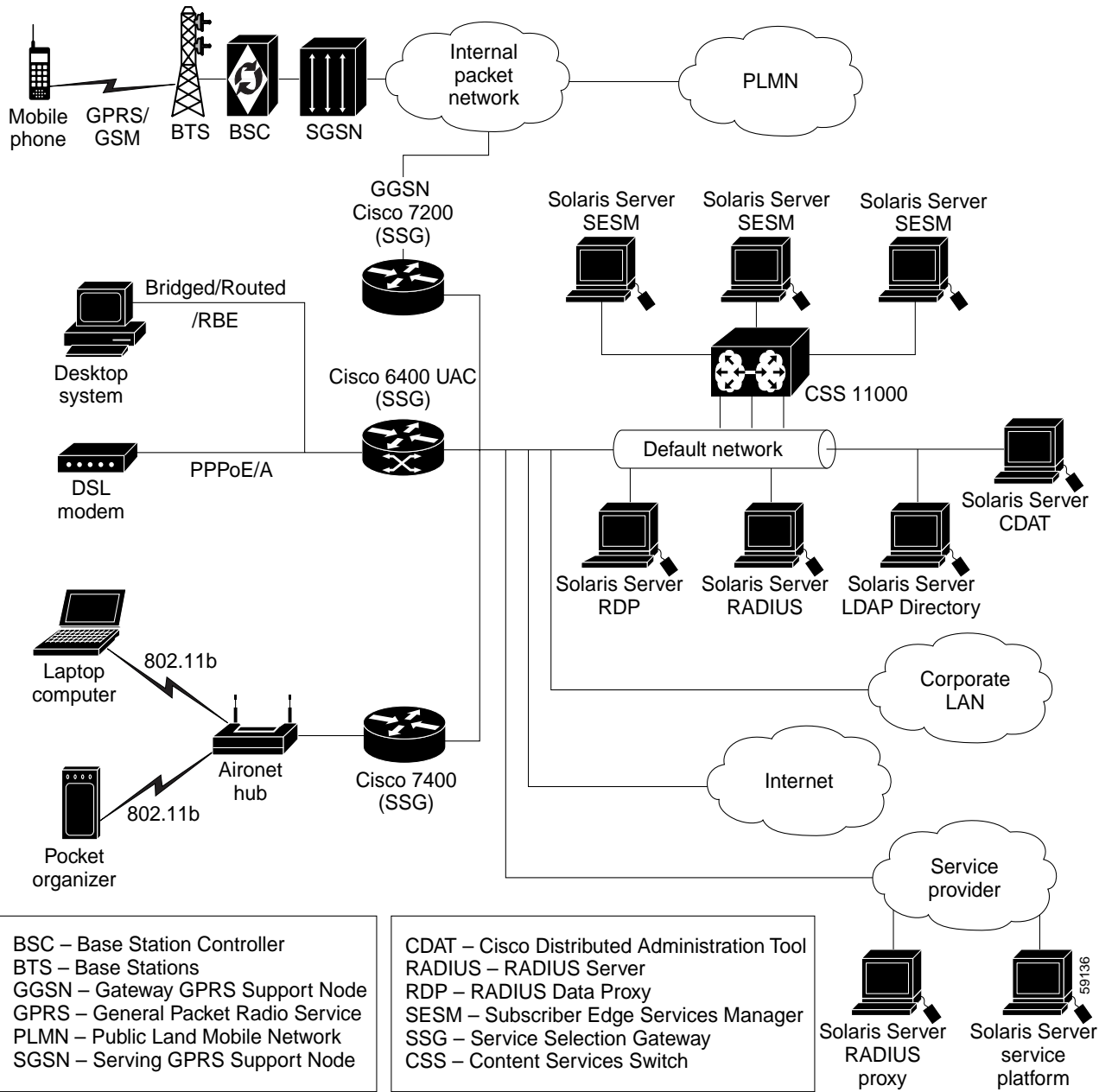
Figure 3-1 Network Diagram
