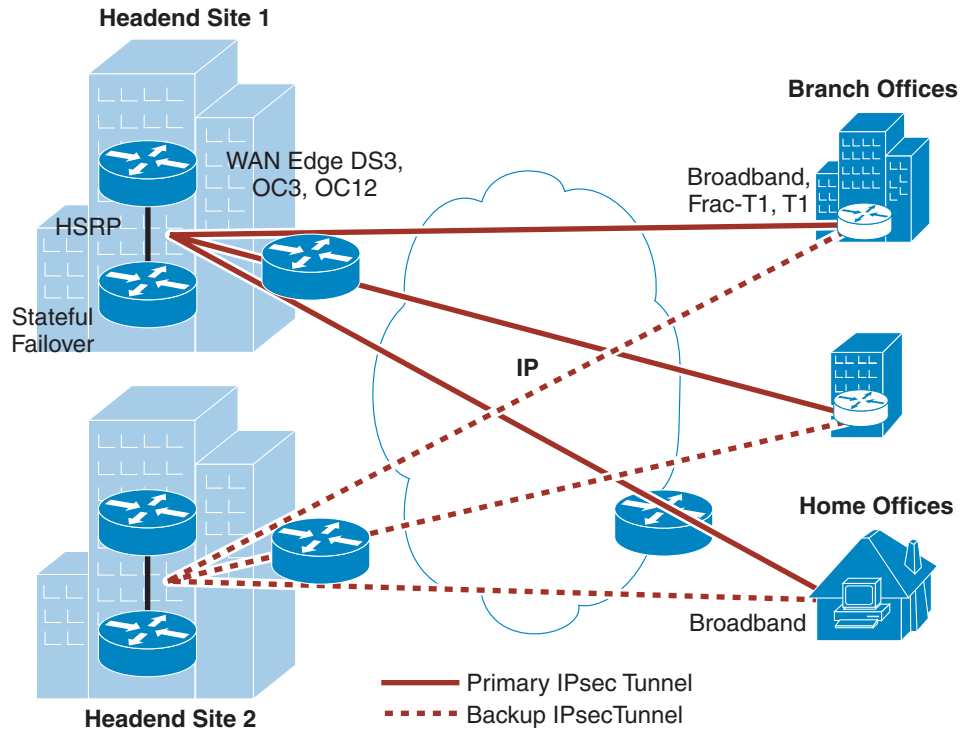
Figure 4 IPsec Direct Encapsulation Deployment
