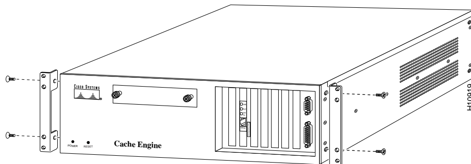
Figure 1 Attaching the Mounting Brackets
