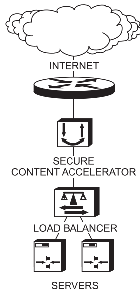
Figure 2-4 Secure Content Accelerator Installation with a Load Balancer
