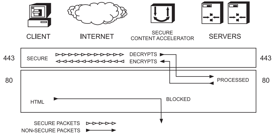
Figure 3-2 Port Blocking with Dropped Traffic
