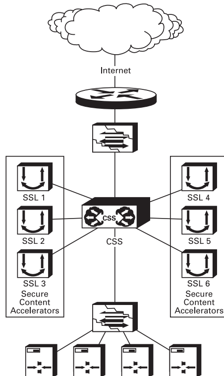
Figure 2-8 Secure Content Accelerator One-Armed Transparent Proxy Installation
