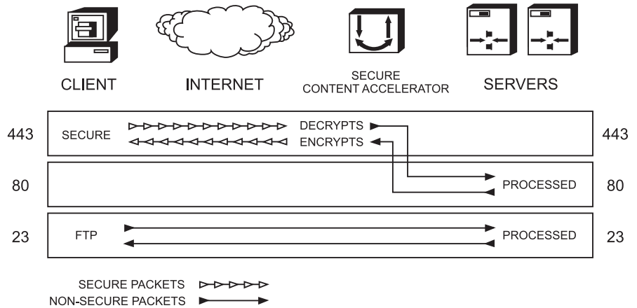
Figure 3-1 Port Blocking
