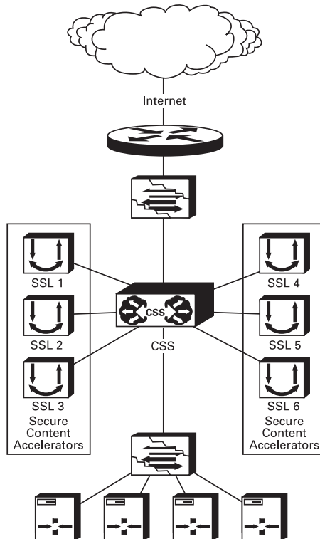
Figure 2-7 Secure Content Accelerator One-Armed Non-Transparent Proxy Installation
