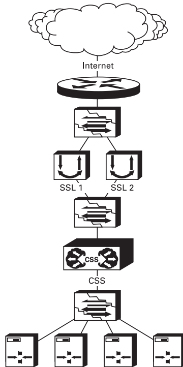
Figure 2-5 Secure Content Accelerator In-Line Installation
