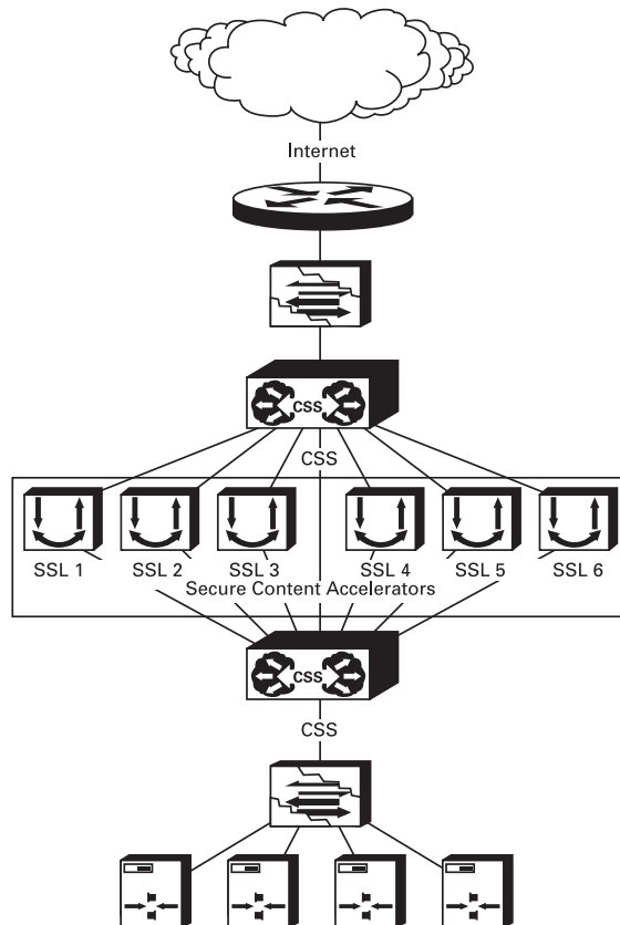
Figure 2-6 Secure Content Accelerator Transparent Sandwich Installation
