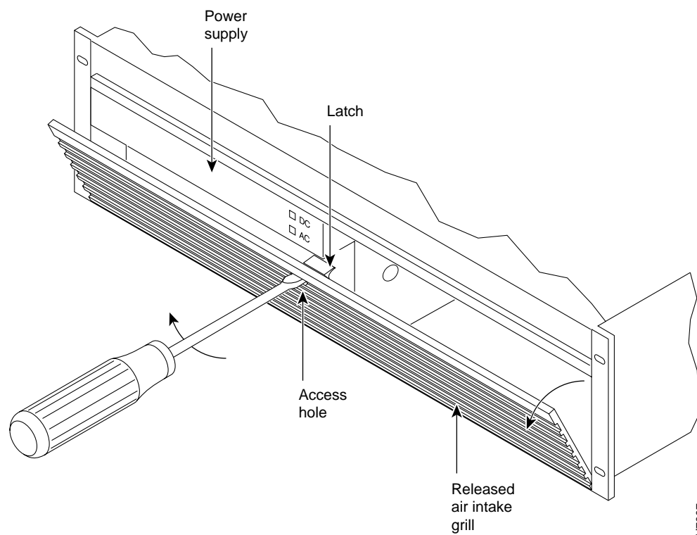
Figure 5-1 Unlatching the Air Intake Grille
