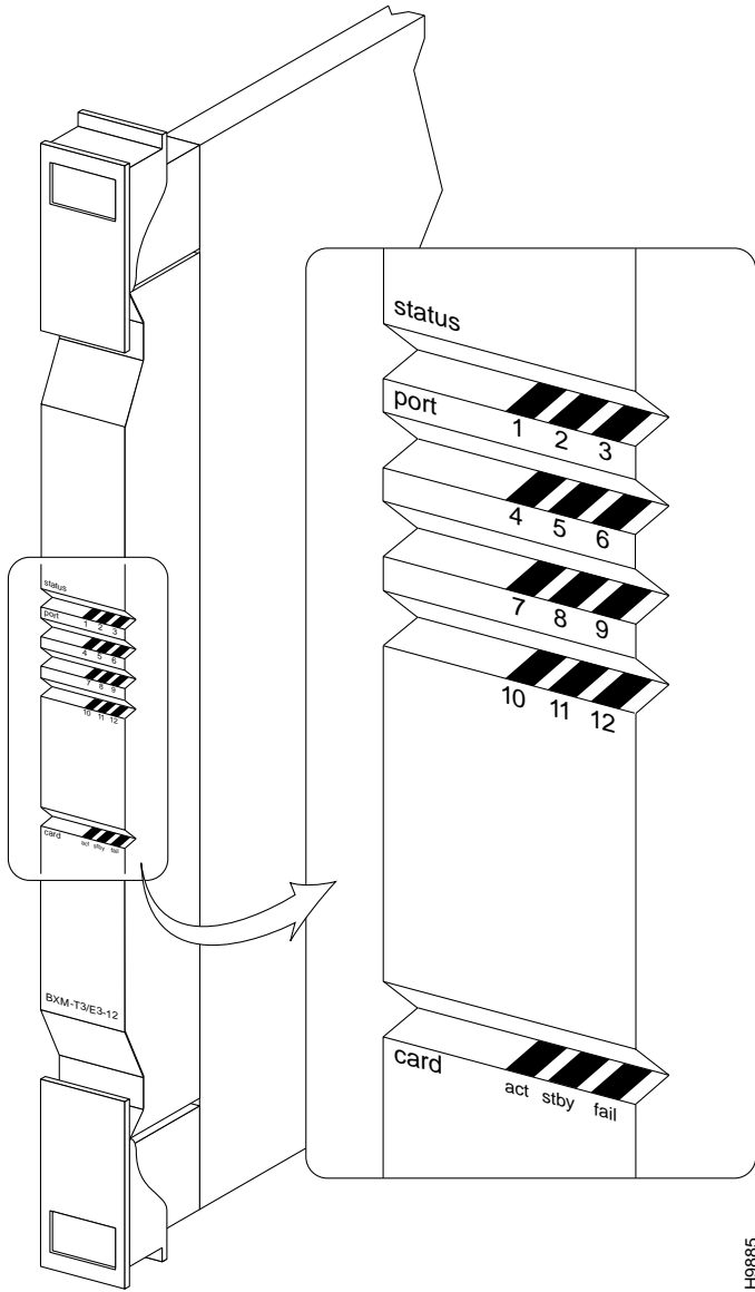
Figure 2-4 BXM-T3/E3 Front Panel, 12-Port Card Shown
