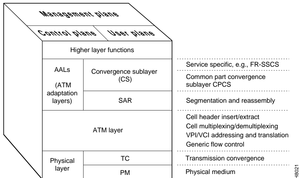
Figure 6-7 ATM Layers
