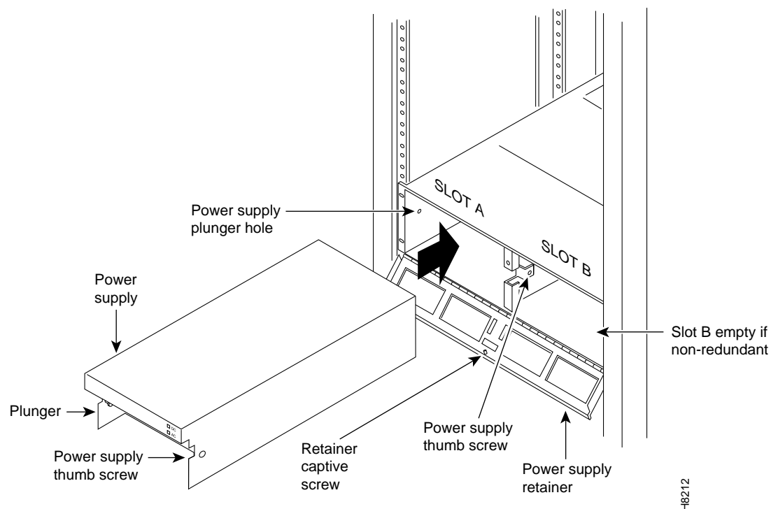
Figure 5-4 AC Power Supply Assembly
