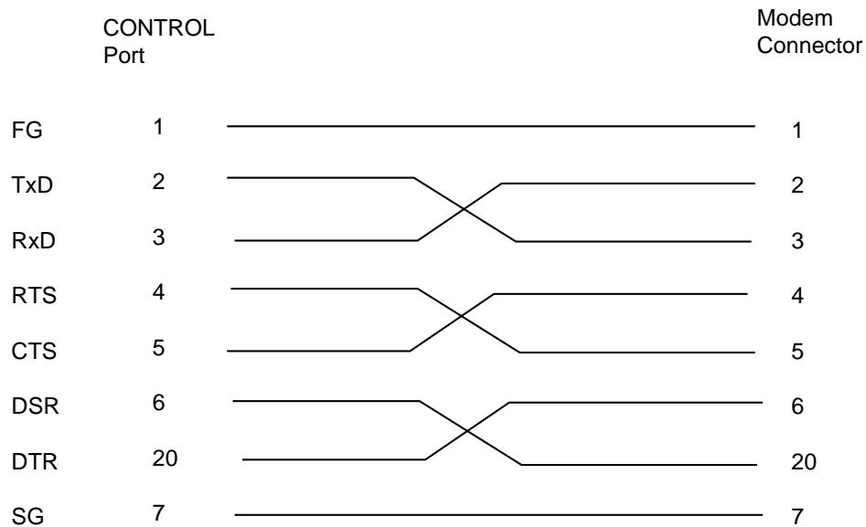
Figure C-1 Dial-Modem Cabling for Auto Answer (Dial-In to BPX)
