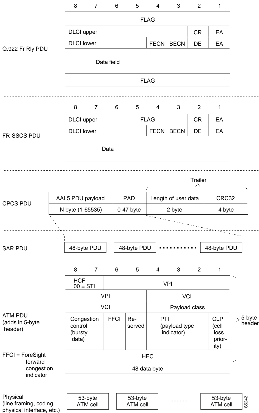
Figure 6-8 Protocol Stack Operation
