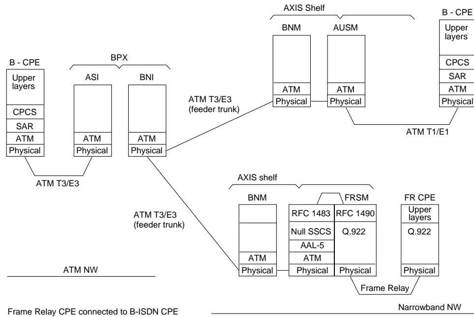
Figure 6-4 Frame Relay to ATM Service Interworking Detail
