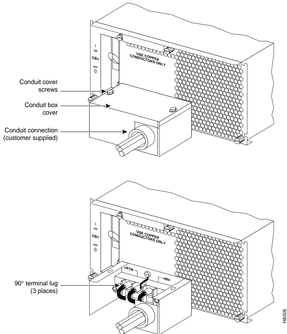
Figure 5-3 DC Power Entry Module with Conduit Box
