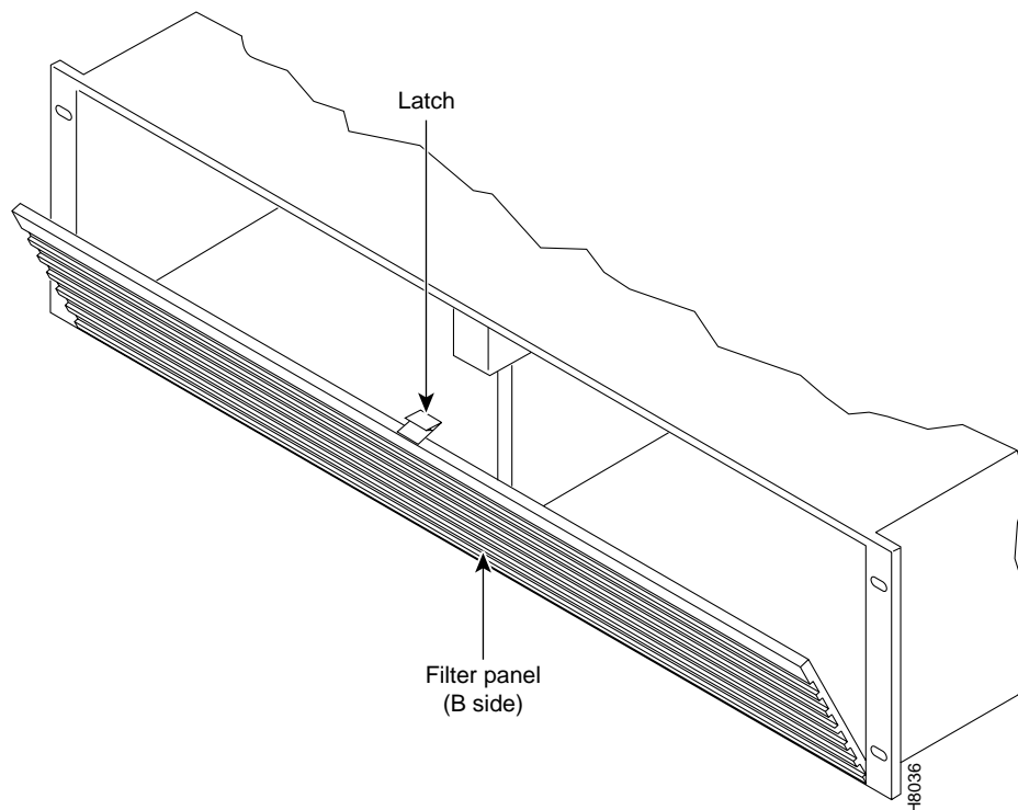
Figure 5-5 Removing Blank Filler Panel (B side shown)
