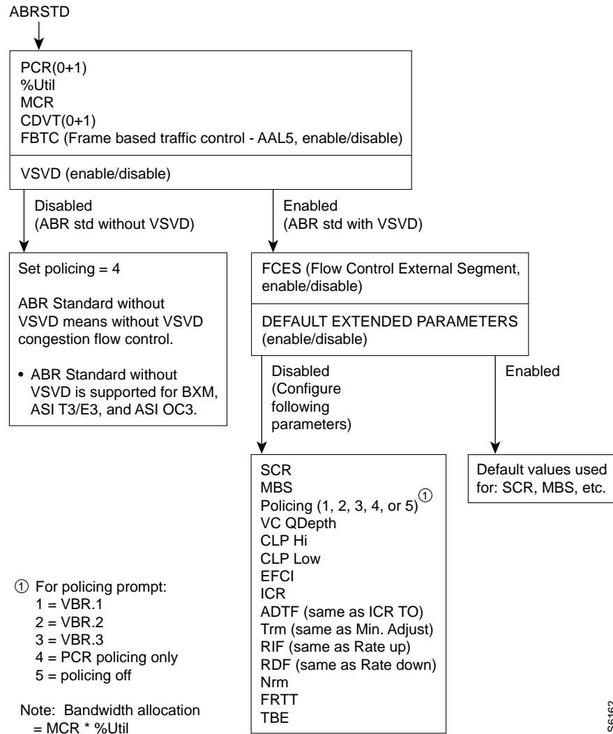
Figure 3-6 ABR Standard Connection Prompt Sequence
