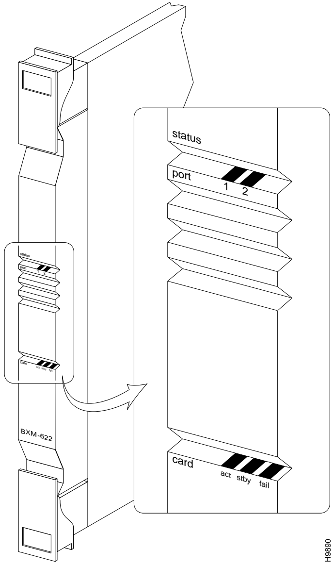
Figure 2-2 BXM-622 Front Panel, Two-Port Card Shown
