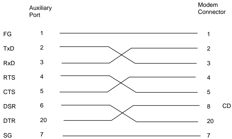
Figure C-2 Dial Modem Cabling for Auto Dial (dial-out to customer service)
