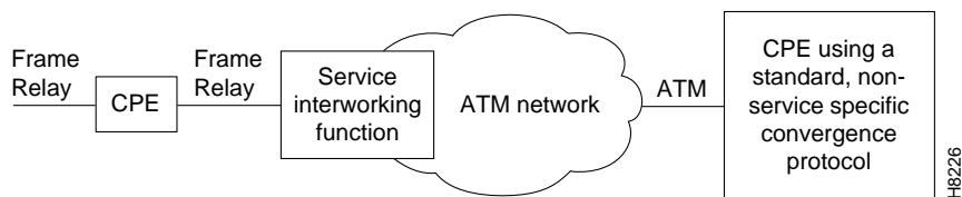
Figure 6-2 Frame Relay to ATM Service Interworking
