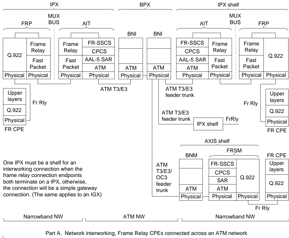
Figure 6-5 Frame Relay to ATM NW Interworking Detail
