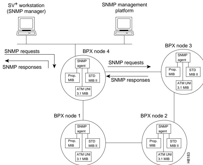
Figure 8-1 SNMP Manager and Agents in a BPX Domain
