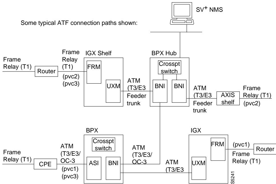
Figure 6-6 ATF Connections, Simplified Example
