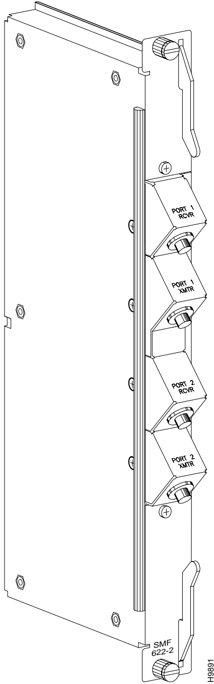
Figure 2-5 SMF-622-2, SMFLR-622-2, and SMFXLR-622-2 Back Card
