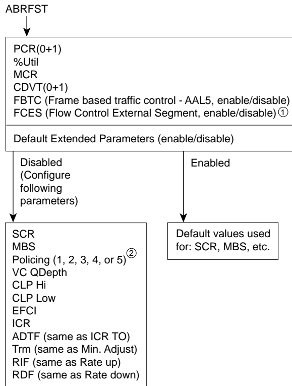
Figure 3-8 ABR ForeSight Connection Prompt Sequence
