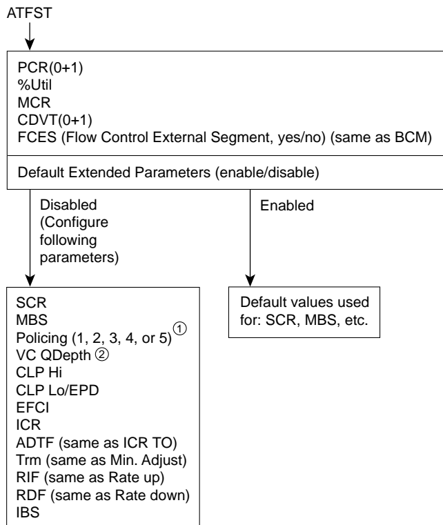
Figure 3-9 ATFST Connection Prompt Sequence
