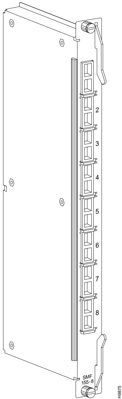
Figure 2-6 BXM-155-8 Port Backcard, MMF, SMF, or SMFLR
