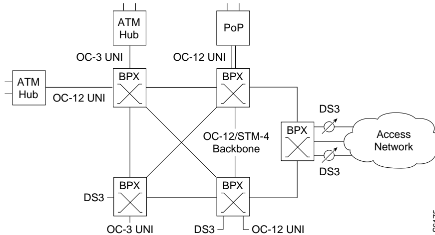
Figure 2-1 A BPX Network with BXM Cards
