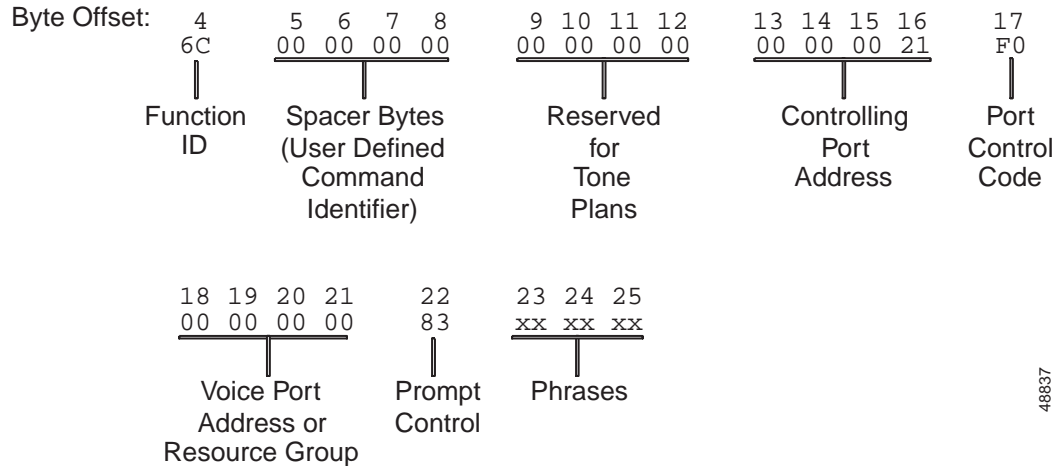
Figure 4-17 $6C (Standard) Command Format
