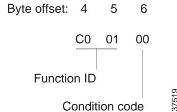
Figure 4-31 $C0 01 Command Format
