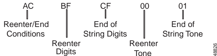
Figure 4-10 Reenter/End of String Segment of the $67 (Enhanced) Command
