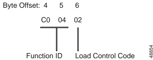
Figure 4-34 $C0 04 Command Format
