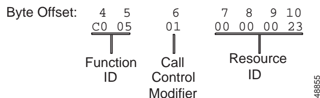
Figure 4-35 $C0 05 Command Format
