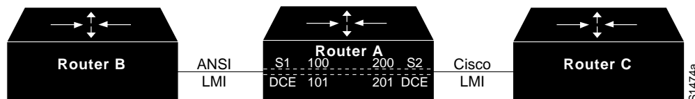
Figure 1-3 PVC Switching Configuration
