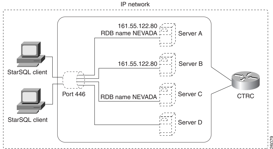
Figure 244 CTRC Server Configurations with IP Addresses, RDB Names, and Default Port
