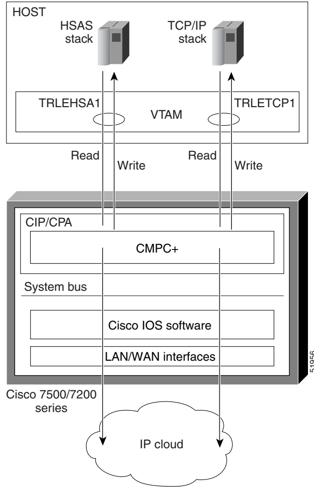
Figure 266 CMPC+ IP Structure
