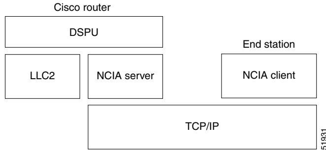
Figure 209 Logical View of NCIA Server with DSPU
