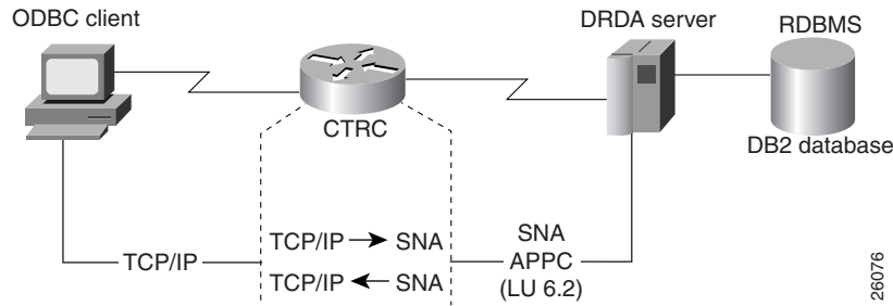
Figure 240 Cisco Router Configured with the CTRC Feature for DB2 Communications (SNA Host Network)
