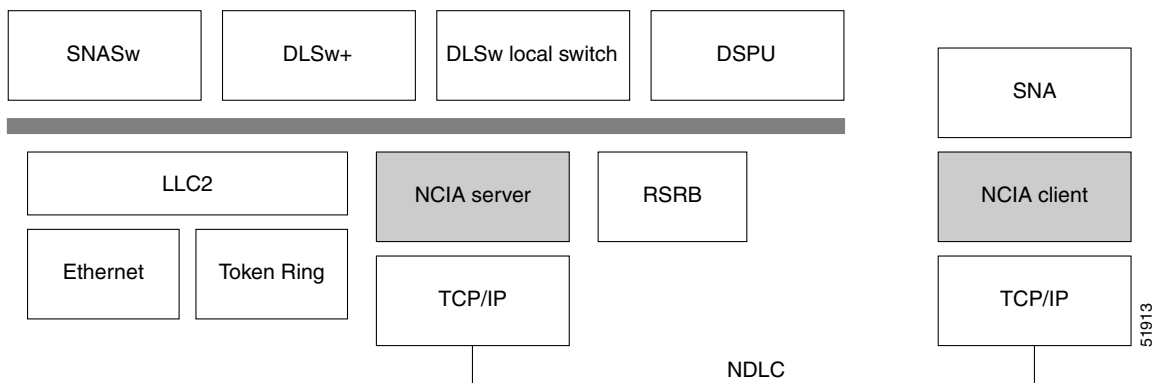
Figure 201 NCIA Server Client/Server Model
