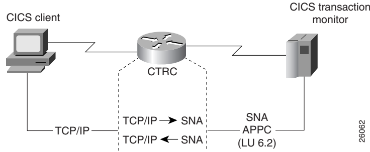
Figure 239 Cisco Router Configured with the CTRC Feature for CICS Communications
