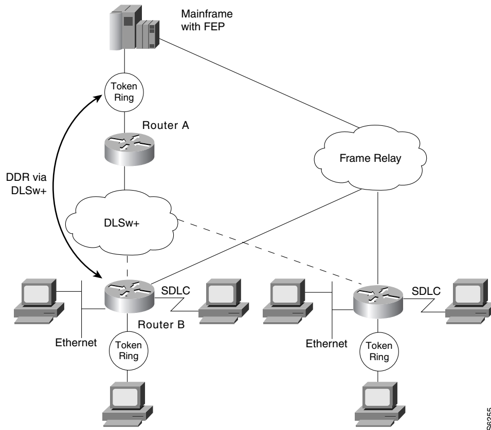
Figure 189 FRAS Dial Backup over DLSw+
