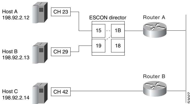
Figure 249 System with an ESCON Director Switch and a Directly Attached Channel
