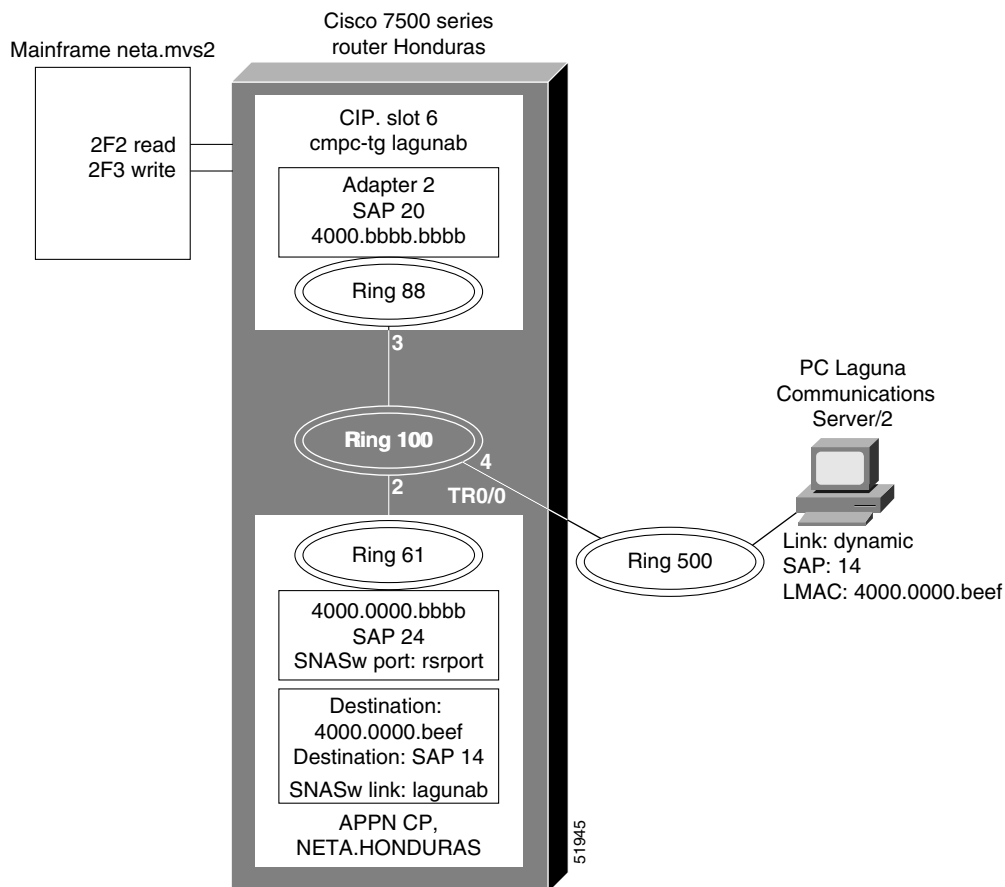
Figure 235 Topology for VTAM-to-SNASw Connection on the CIP
