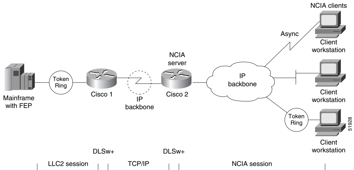
Figure 213 NCIA Server Session with DLSw+
