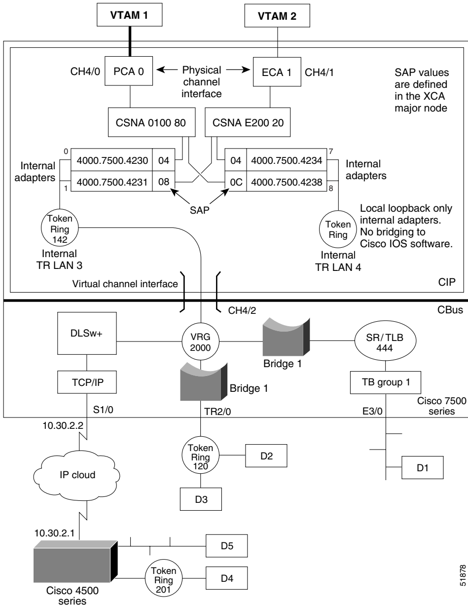
Figure 255 CIP CSNA Source-Route Translational Bridging Configuration
