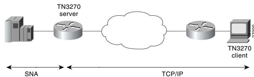
Figure 275 TN3270 Implementation
