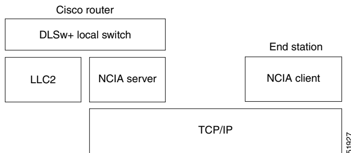
Figure 205 Logical View of NCIA Server Session to a Local Token Ring Using DLSw+ Local Switch
