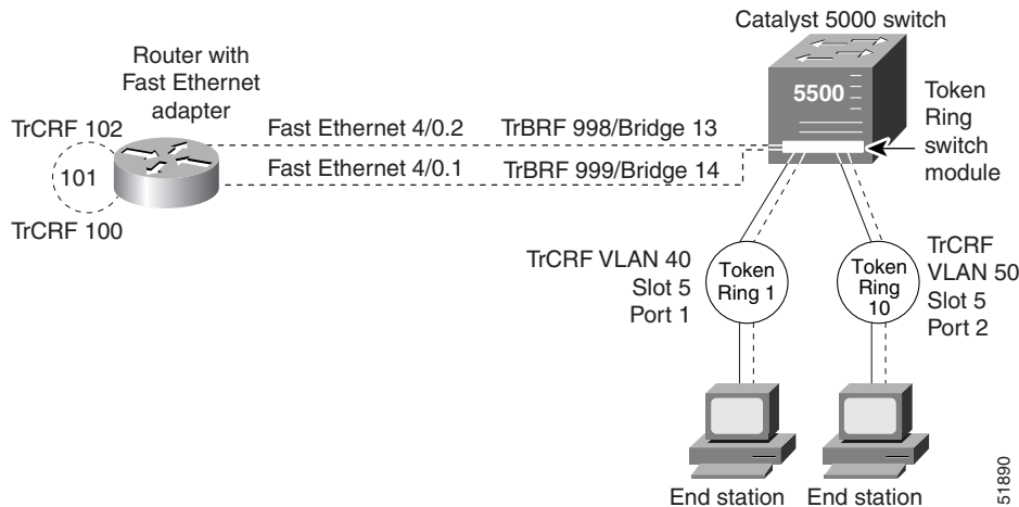
Figure 64 SRB Between TRISL VLANs
