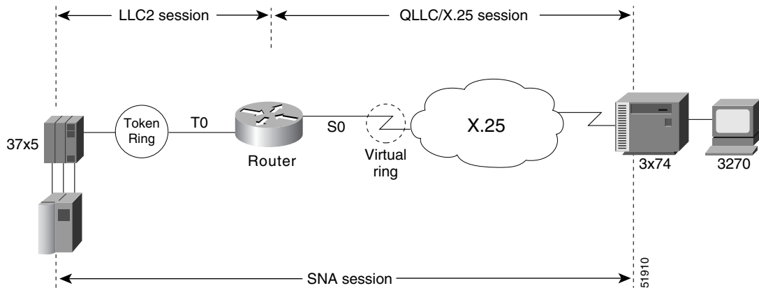
Figure 168 QLLC Conversion Between a Single 37x5 and a Single 3x74
