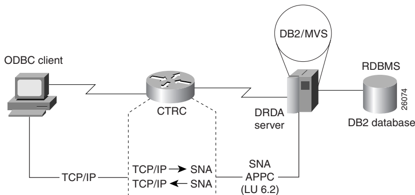
Figure 245 Cisco Router with CIP and Connection to DB2 on VTAM
