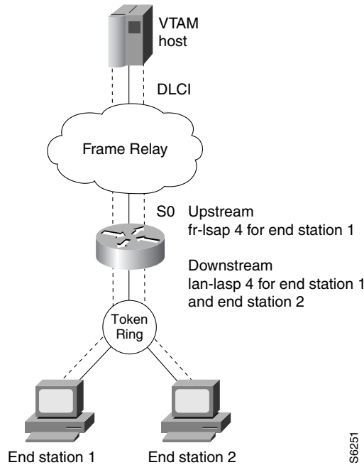
Figure 196 Frame Relay BNN Support
