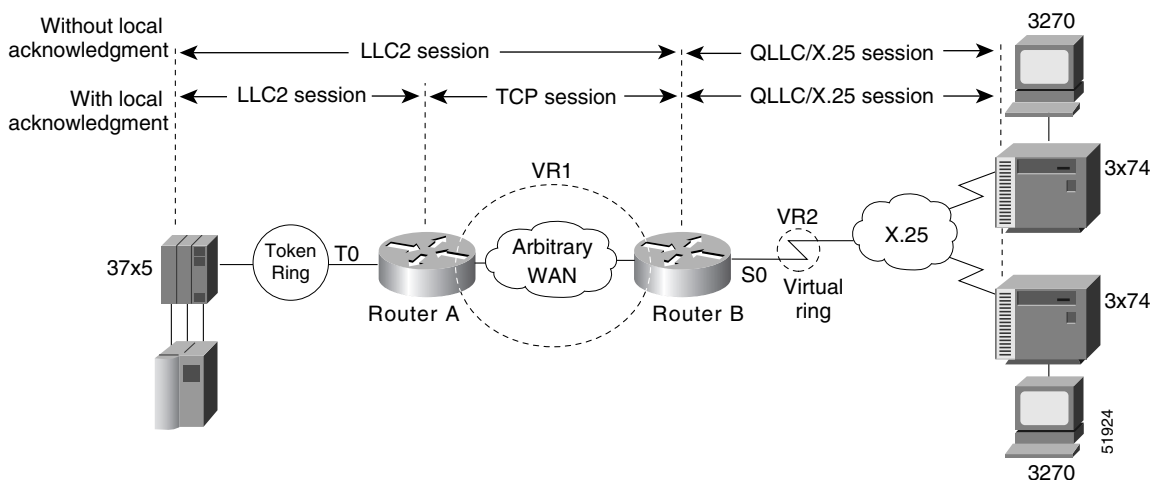
Figure 177 QLLC Conversion Between a Single 37x5 and Multiple 3x74s Across an Arbitrary WAN
