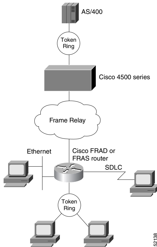
Figure 192 Cisco FRAD Access to a LAN-Attached AS/400 through a Cisco 4500
