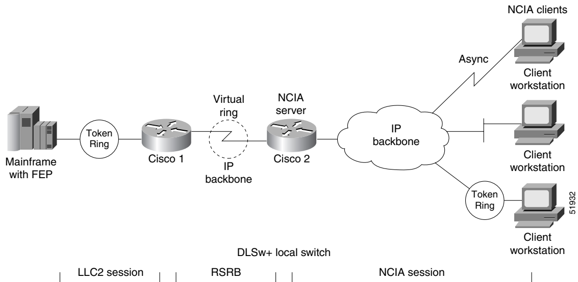
Figure 210 NCIA Server Session with RSRB
