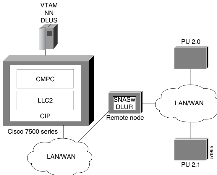
Figure 263 Topology for VTAM-to-SNASw on a Remote Router with DLUR Connection
