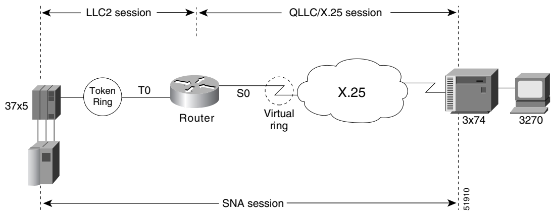
Figure 176 QLLC Conversion Between a Single 37x5 and a Single 3x74
