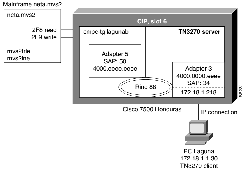
Figure 285 Parameters for VTAM-to-TN3270 DLUR Using CMPC
