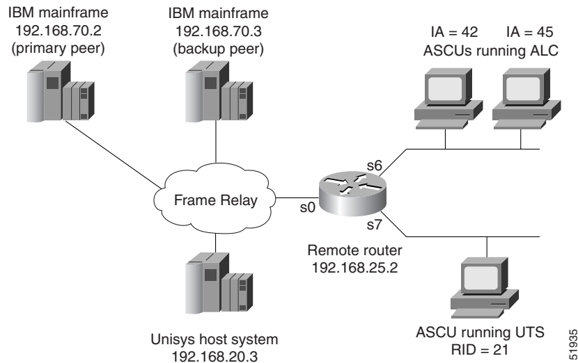
Figure 218 Router Topology for the ALPS with MATIP Configuration Example
