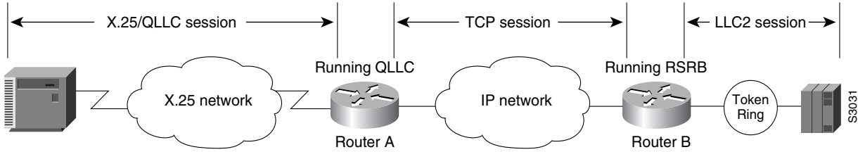
Figure 167 QLLC Conversion Running on a Router with an Intermediate IP Network
