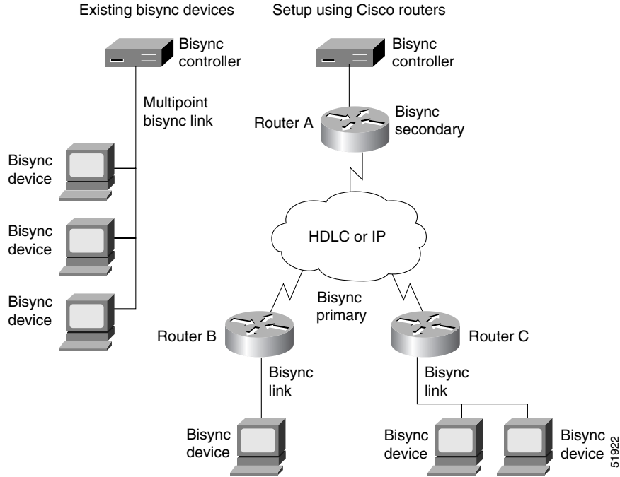
Figure 155 Multipoint Bisync Link Reconfigured Using Routers
