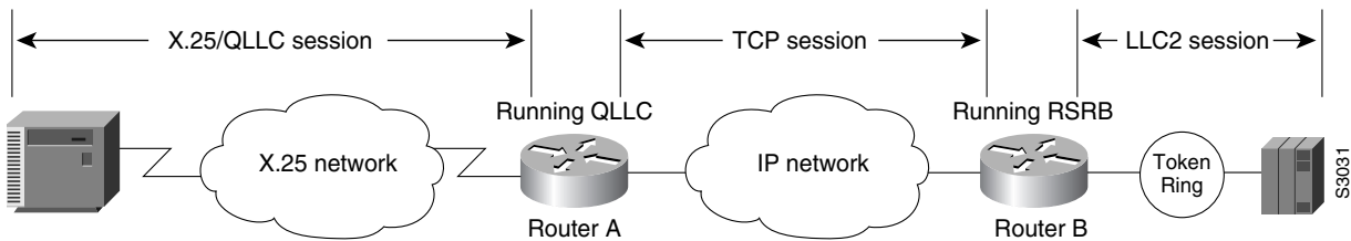
Figure 175 QLLC Conversion Running on a Router with an Intermediate IP Network
