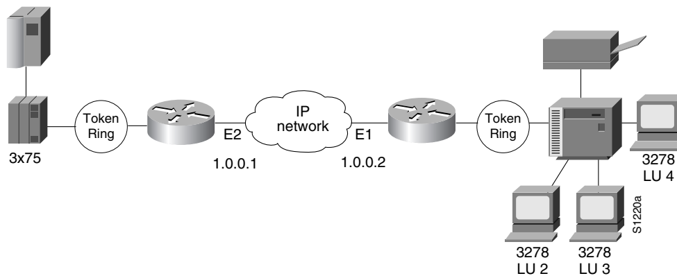
Figure 126 RSRB Configuration Example
