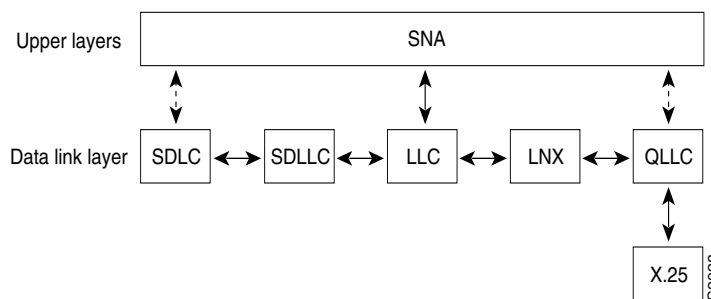
Figure 172 SNA Data Link Layer Support
