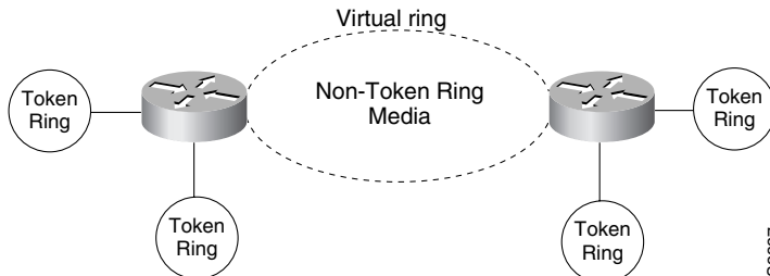
Figure 114 RSRB Topology
