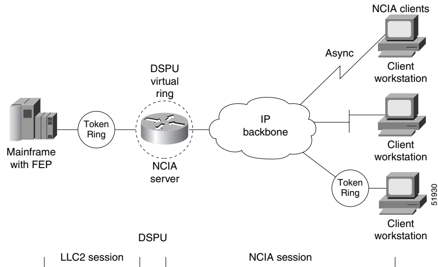
Figure 214 NCIA Server Session with RSRB/DLSw+ and DSPU
