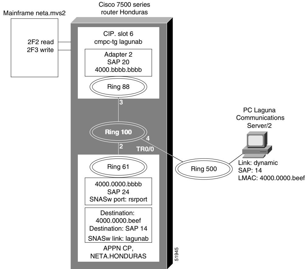
Figure 260 Parameters for VTAM-to-SNASw Connection on the CIP
