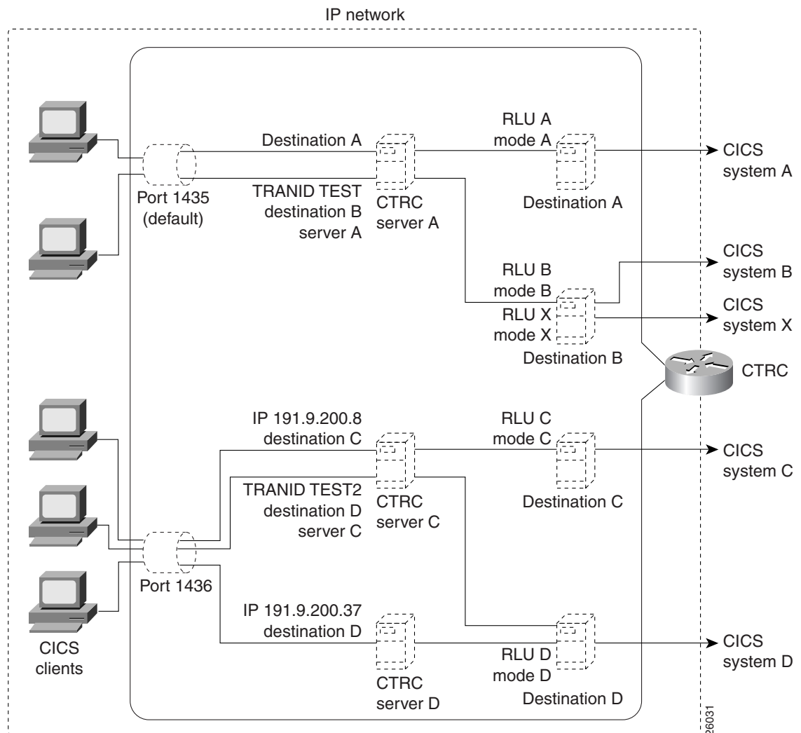
Figure 247 CTRC Configuration with IP Addresses, Routes, and Multiple CICS Destinations
