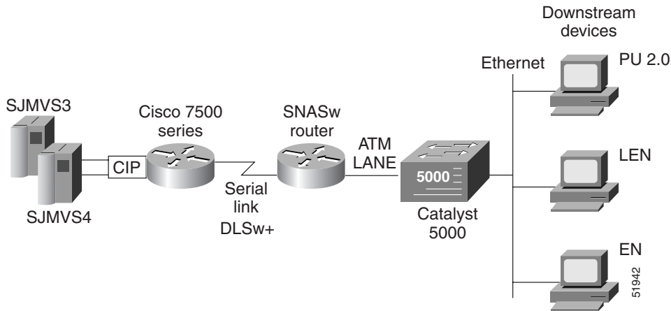
Figure 232 SNASw with Ethernet LANE over ATM
