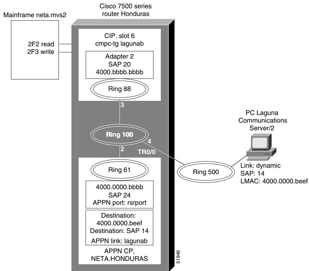
Figure 236 Topology for VTAM-to-APPN NN Configuration on the CIP
