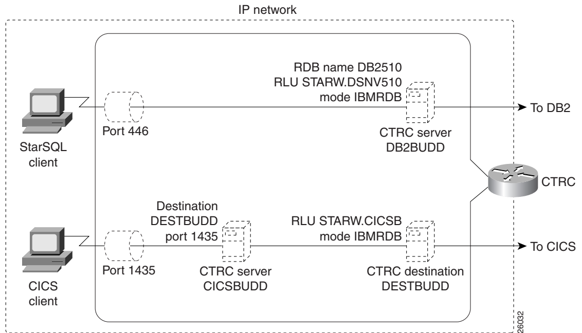
Figure 246 CTRC Configuration for Communication with DB2 and CICS
