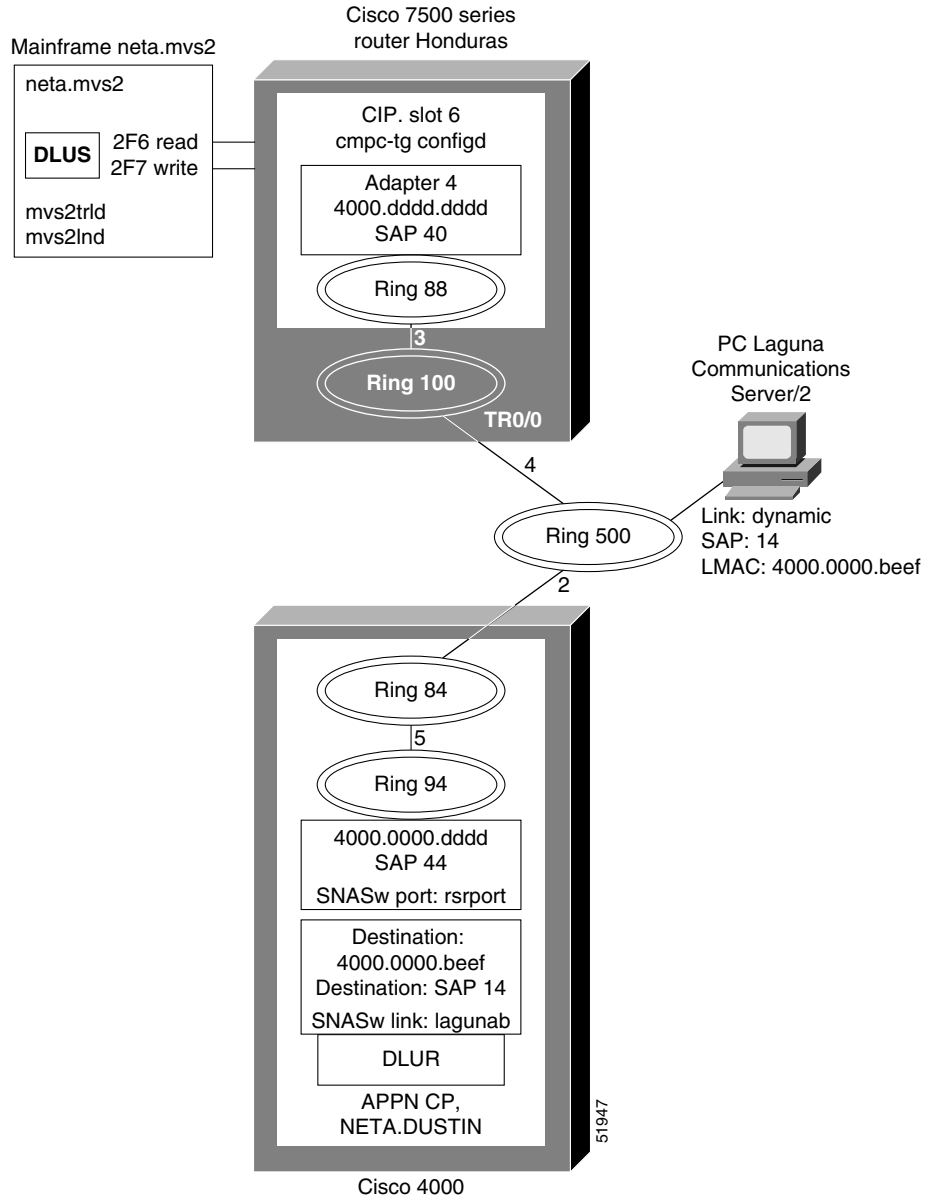
Figure 264 Parameters for VTAM-to-SNASw on a Remote Router with DLUR Connection
