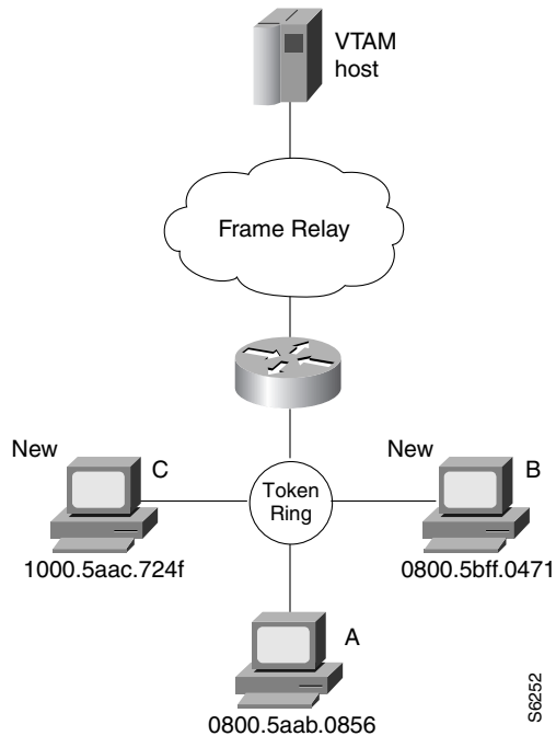
Figure 197 FRAS BNN Configuration
