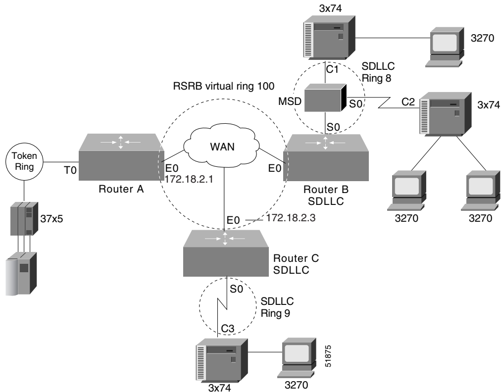
Figure 182 SDLLC with RSRB with Multiple 3x74s
