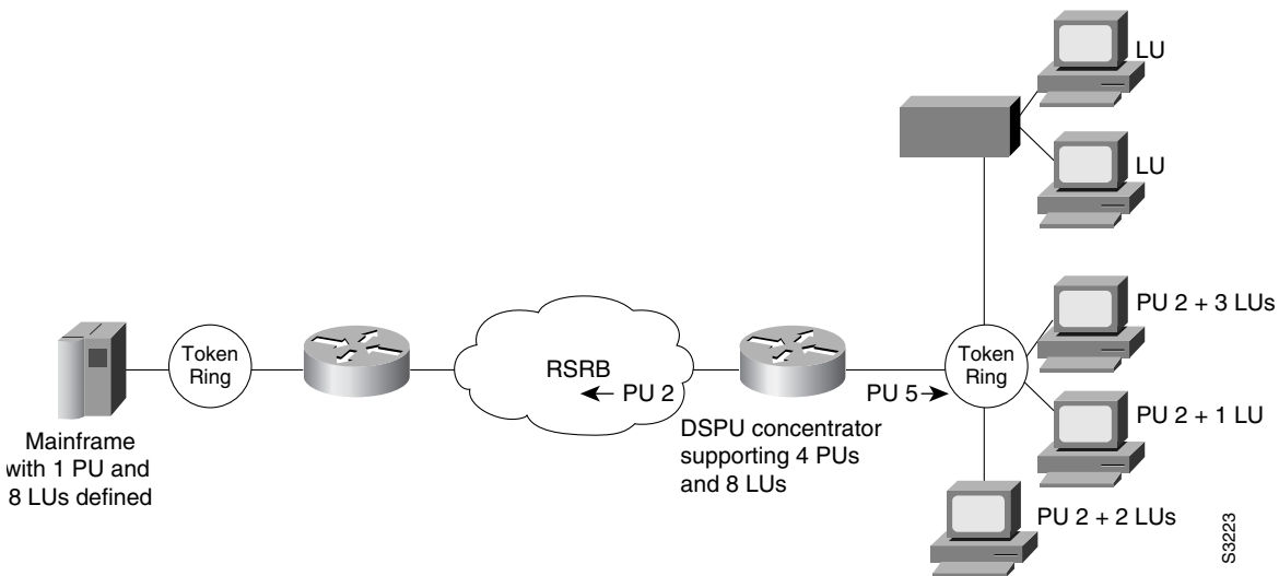
Figure 220 Router Acting as a DSPU Concentrator
