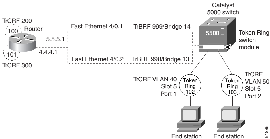
Figure 58 IP Routing Source-Routed Frames Between TrBRF VLANs
