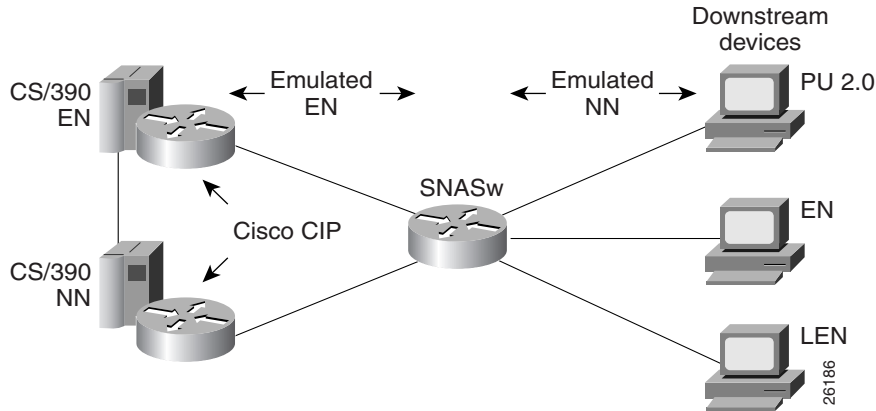
Figure 107 BEX Functionality
