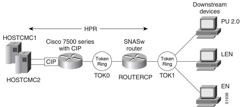
Figure 227 SNASw over Token Ring with HPR
