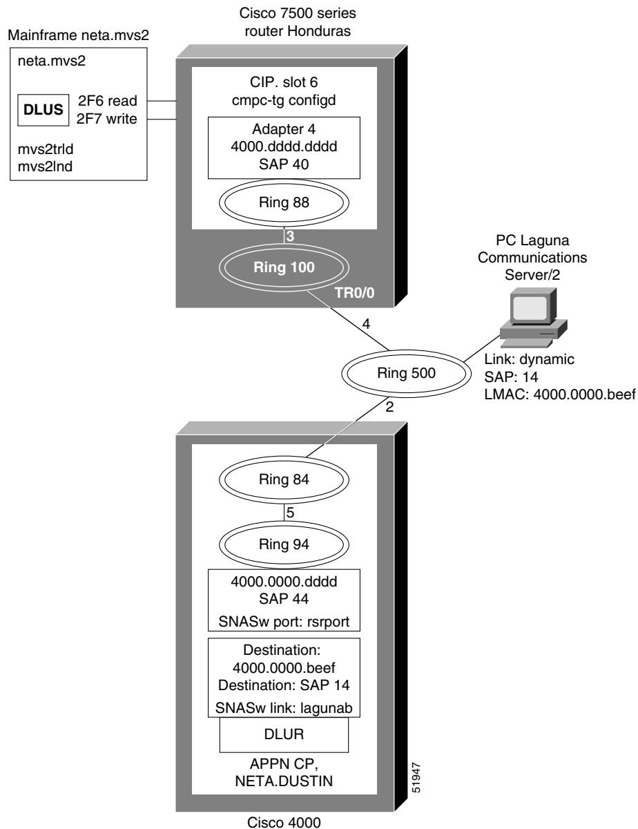
Figure 238 Topology for VTAM-to-APPN NN on a Remote Router with DLUR Connection
