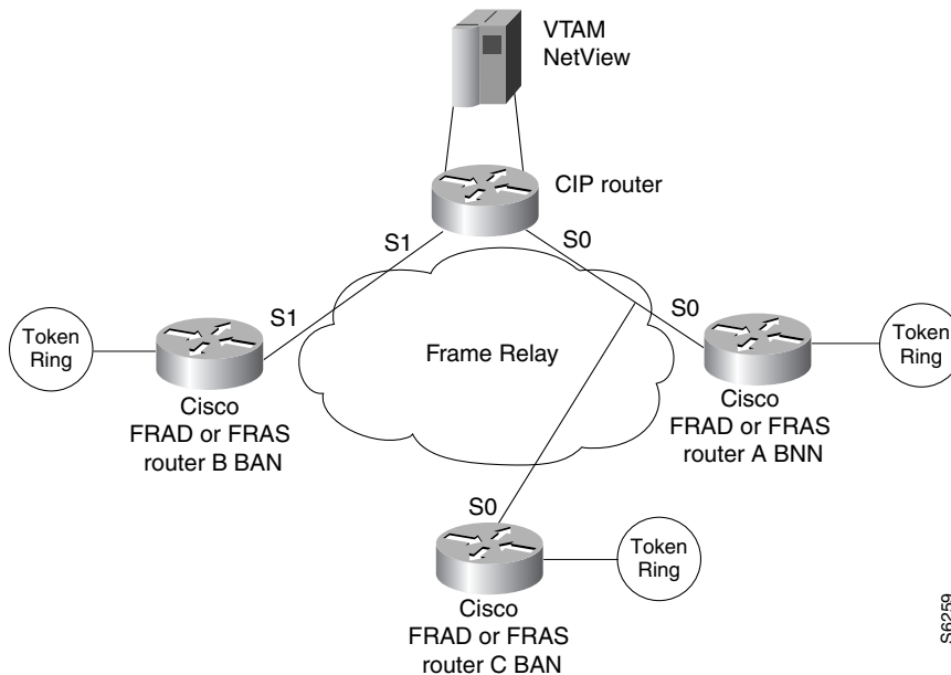
Figure 199 FRAS Host CIP Connection to VTAM
