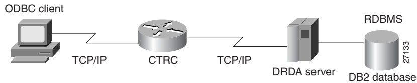
Figure 241 Cisco Router Configured with the CTRC Feature for DB2 Communications (TCP/IP Host Network)
