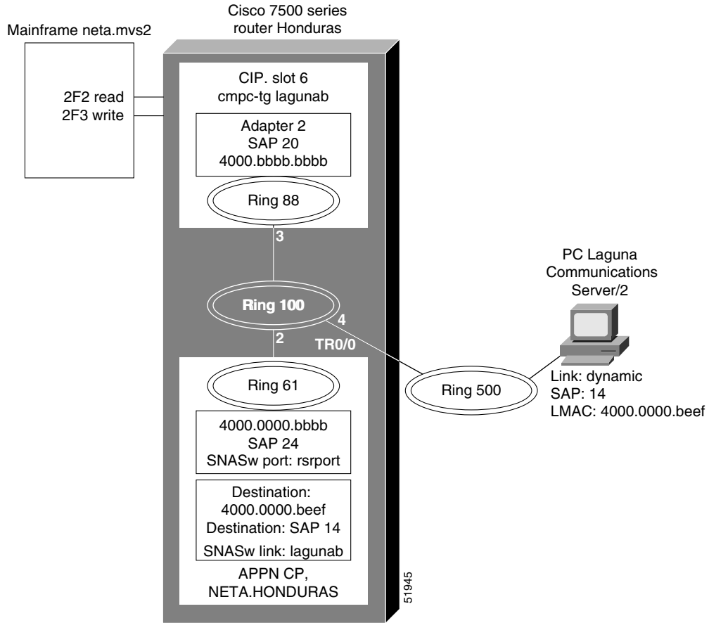
Figure 237 Topology for VTAM-to-SNASw on a Remote Router with DLUR Connection
