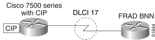
Figure 234 SNASw with FRAS Host (Downstream Frame Relay BNN Support)
