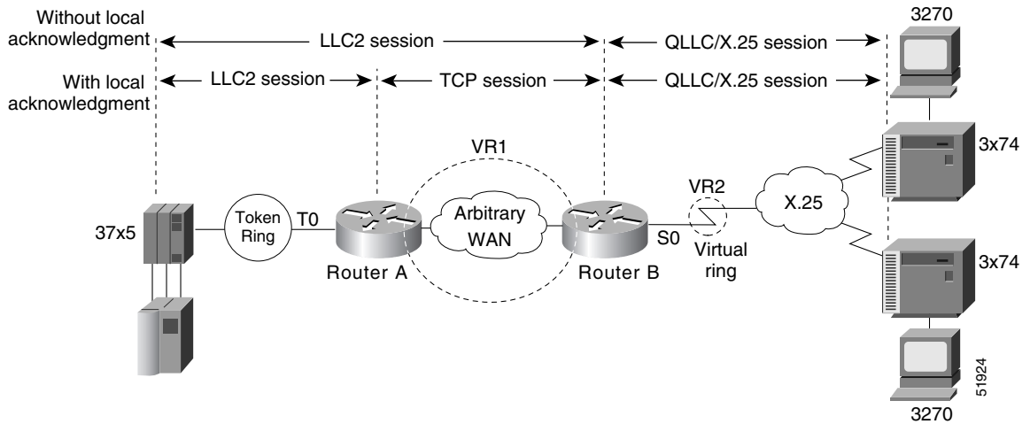
Figure 169 QLLC Conversion Between a Single 37x5 and Multiple 3x74s Across an Arbitrary WAN
