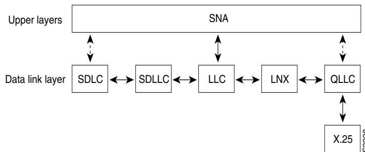
Figure 164 SNA Data Link Layer Support
