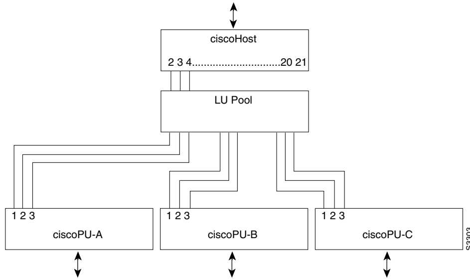
Figure 223 Pooled LU Routing
