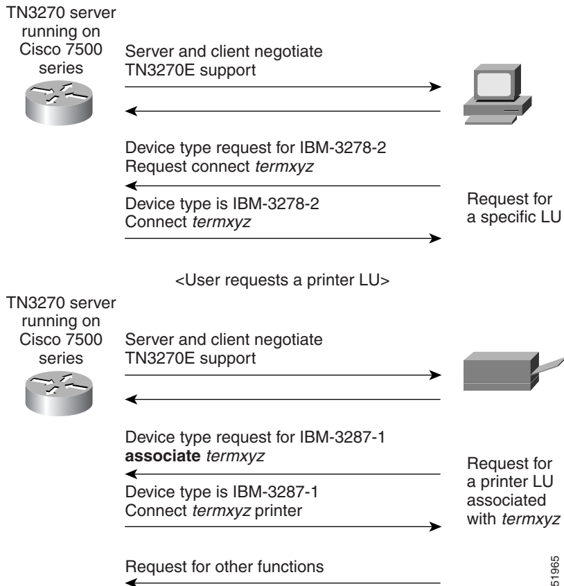
Figure 278 Client Request for a Specific LU and Printer LU Association
