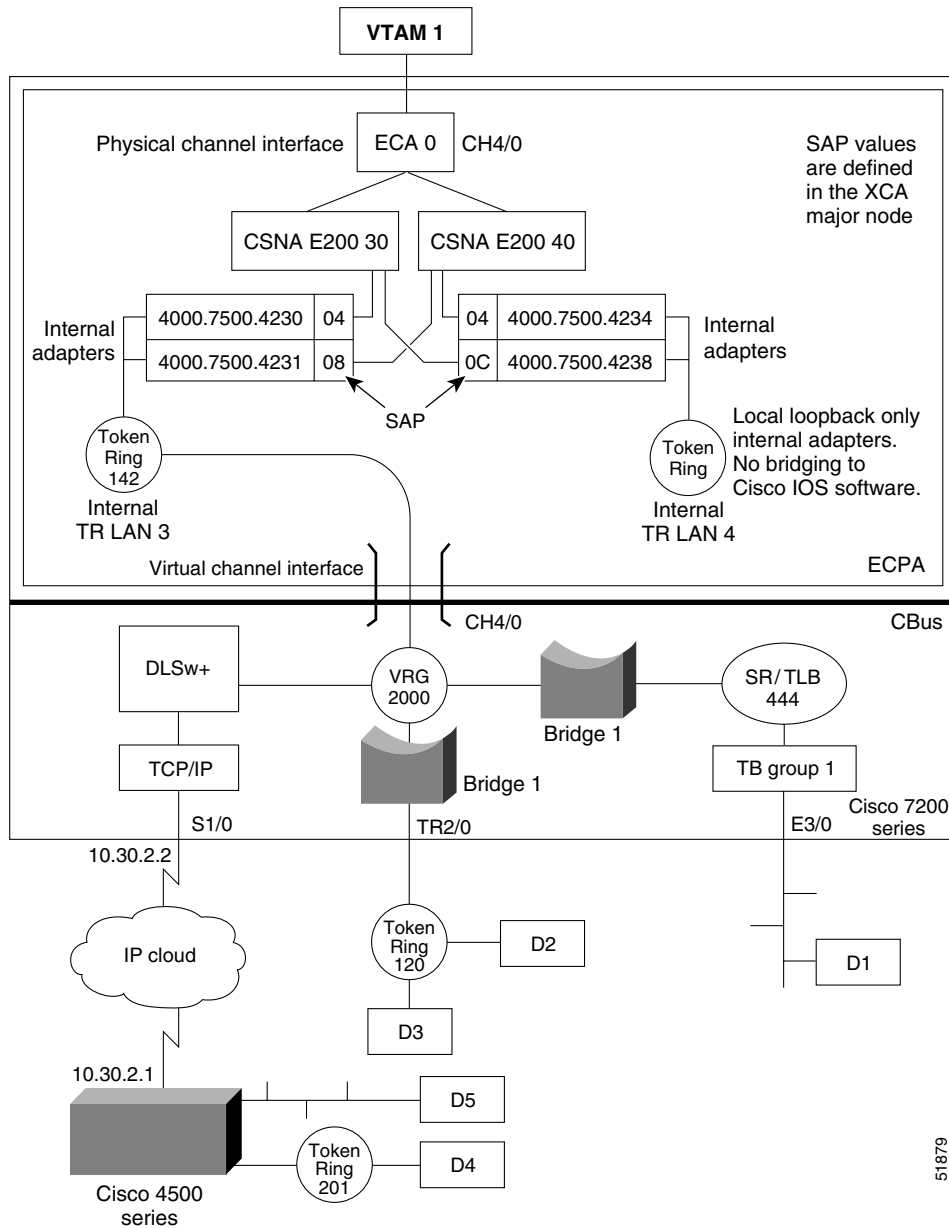
Figure 256 ECPA CSNA Source-Route Translational Bridging Configuration
