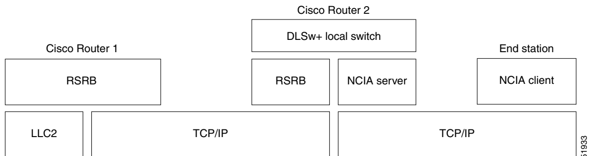
Figure 211 Logical View of NCIA Server Session with RSRB (Remote Token Ring)
