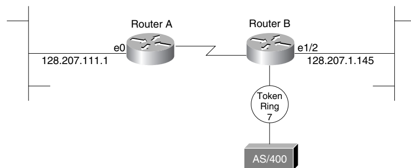
Figure 135 DLSw+ Translation Between Ethernet and Token Ring
