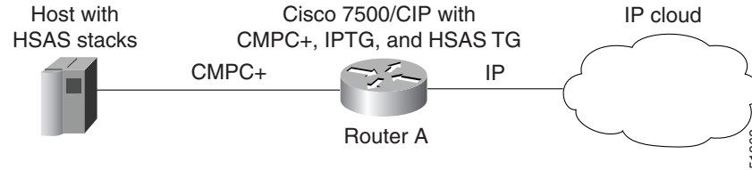
Figure 273 CMPC+ with TCP/IP and HSAS Stacks
