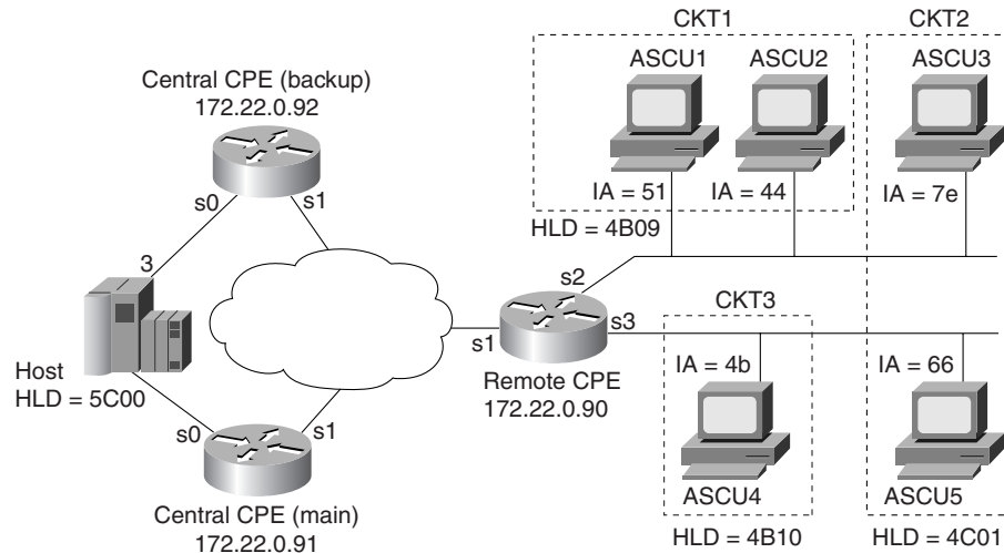
Figure 219 Router Topology for the ALPS Configuration for ALC Encapsulation Example
