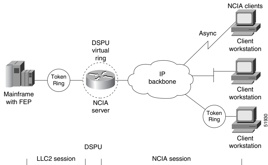
Figure 208 NCIA Server Session with DSPU
