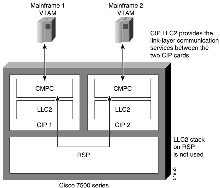
Figure 261 Topology for VTAM-to-VTAM Connection
