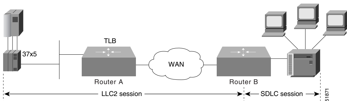
Figure 178 SDLLC with Ethernet and Translational Bridging
