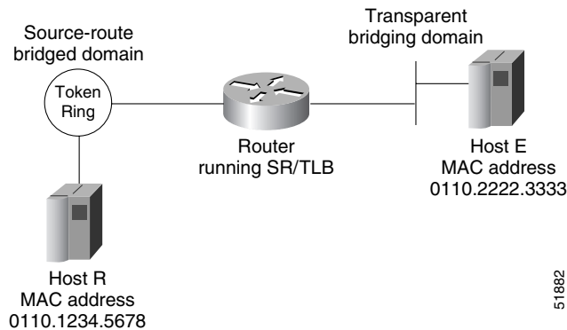
Figure 41 Example of a Bit-Swapped Address
