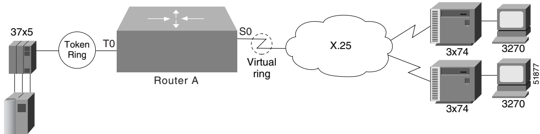
Figure 184 QLLC Conversion Between a Single 37x5 and Multiple 3x74s
