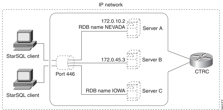
Figure 242 CTRC Servers' Configuration with IP Addresses (for DB2 Communications)
