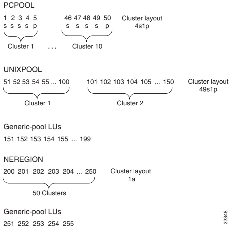
Figure 282 Cluster Layouts for PU1 in the TN3270 Server
