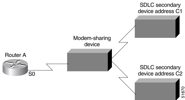
Figure 170 Two SDLC Secondary Stations Attached to a Single Serial Interface Through a Modem-Sharing Device
