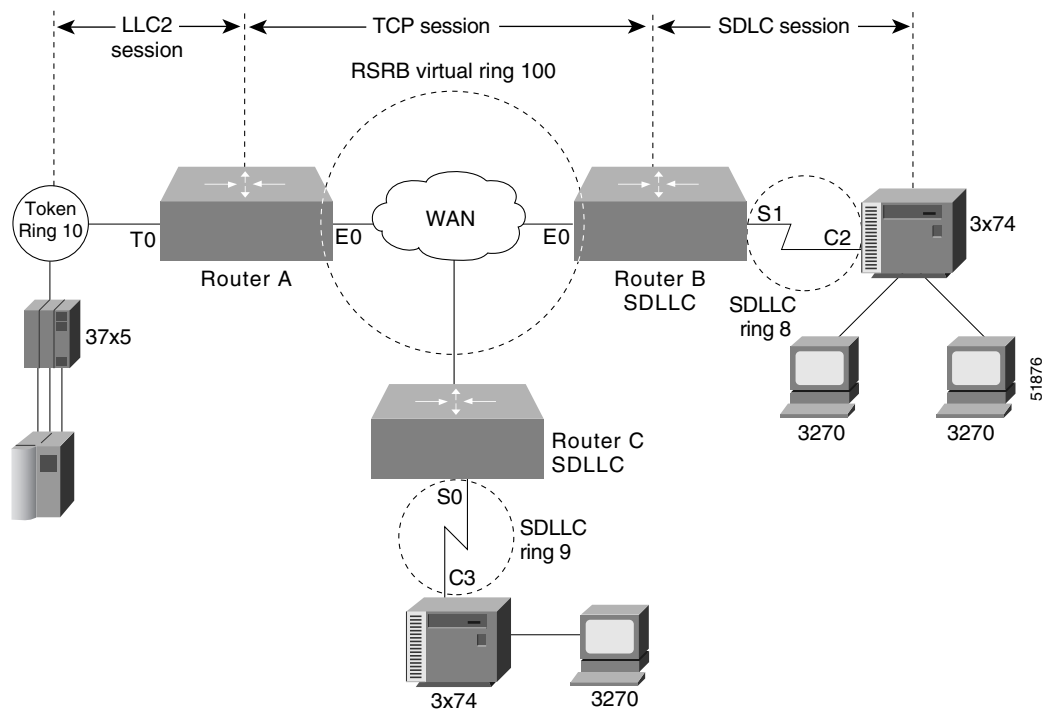
Figure 183 SDLLC with RSRB and Local Acknowledgment
