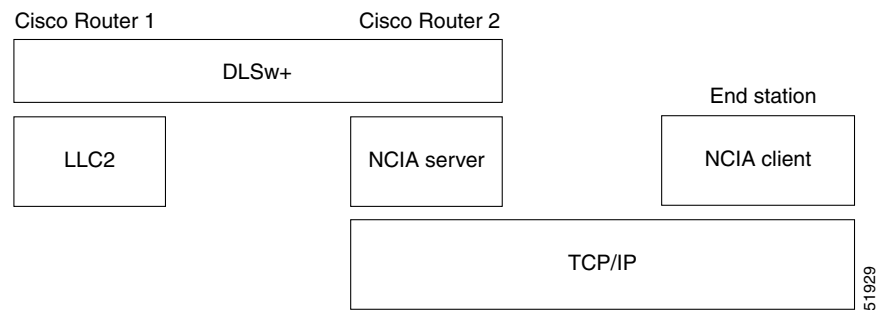
Figure 207 Logical View of NCIA Server with DLSw+
