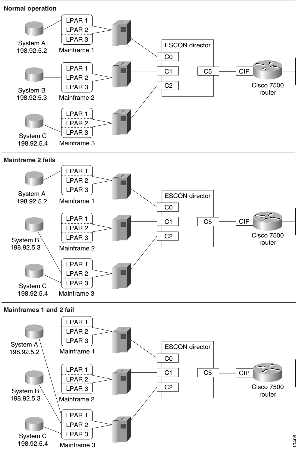
Figure 253 IP Host Backup Configuration
