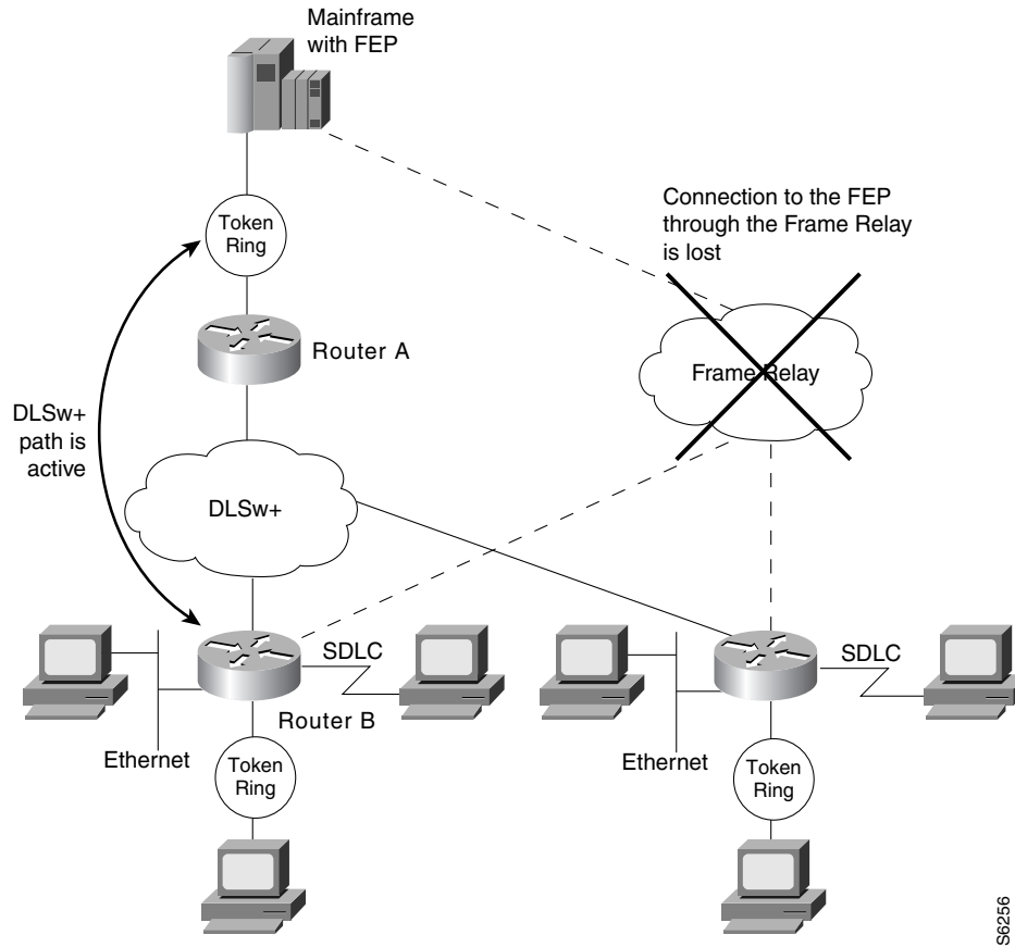
Figure 190 FRAS Dial Backup over DLSw+ when Frame Relay is Unavailable
