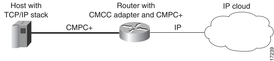
Figure 265 MVS Host with TCP/IP Stack and Cisco Router with CMPC+
