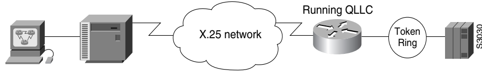
Figure 174 Router Running QLLC Conversion Feature
