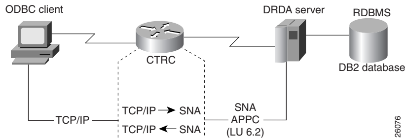
Figure 110 Cisco Router Configured with the CTRC Feature for DB2 Communications (SNA Host Network)
