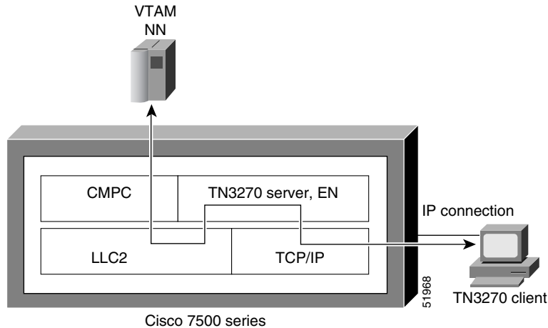
Figure 284 Topology for VTAM-to-TN3270 Server DLUR Using CMPC
