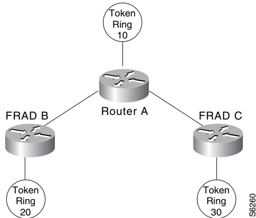
Figure 198 FRAD Using SRB over Frame Relay to Connect to a Cisco Router
