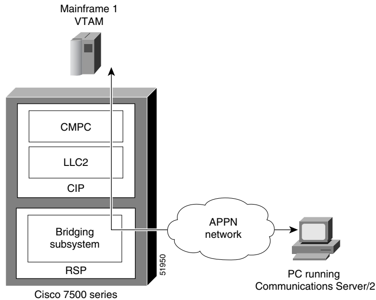
Figure 257 Topology for VTAM-to-Remote PC with Communications Server/2
