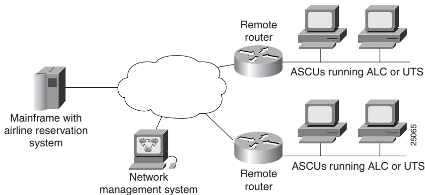
Figure 104 ALPS Architecture
