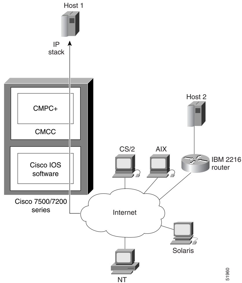
Figure 270 IP Communication from a Host to IP Nodes
