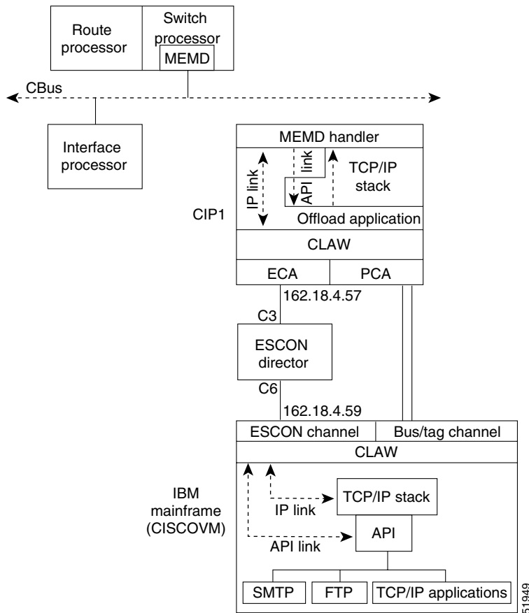
Figure 251 Offload Network Configuration Block Diagram
