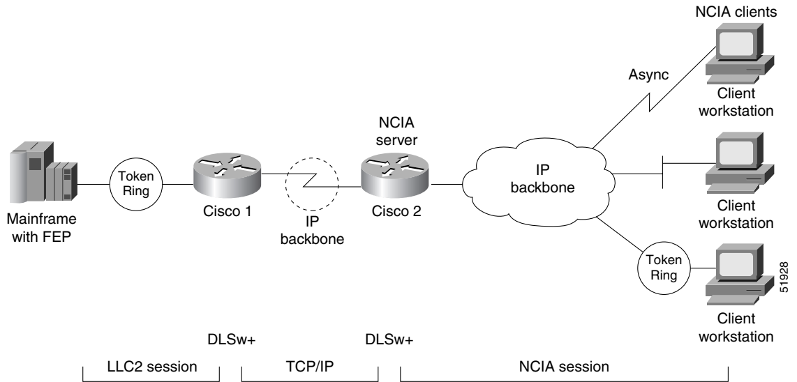
Figure 206 NCIA Server Session with DLSw+
