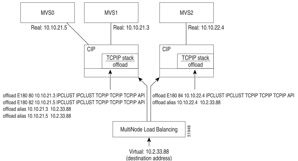
Figure 252 Offload Alias Support on Multiple CMCC Adapters to Multiple Hosts
