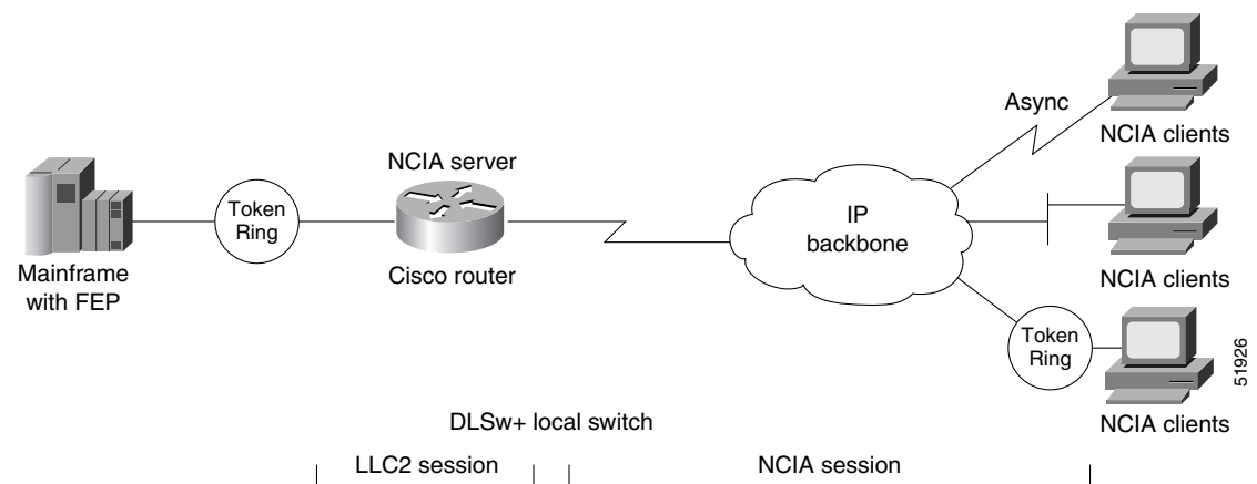
Figure 212 NCIA Server Session to Local Token Ring Using DLSw+ Local Switch
