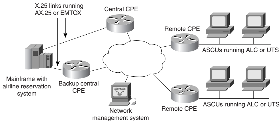
Figure 216 ALPS with ALC and UTS Architecture
