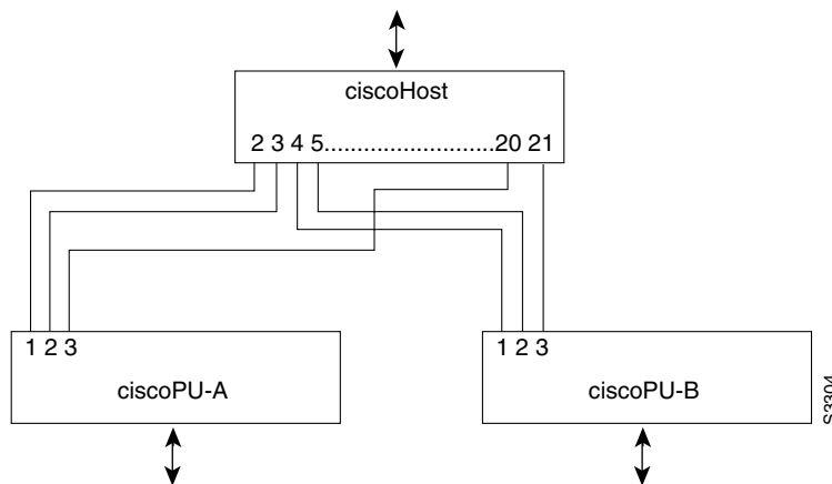
Figure 222 Dedicated LU Routing
