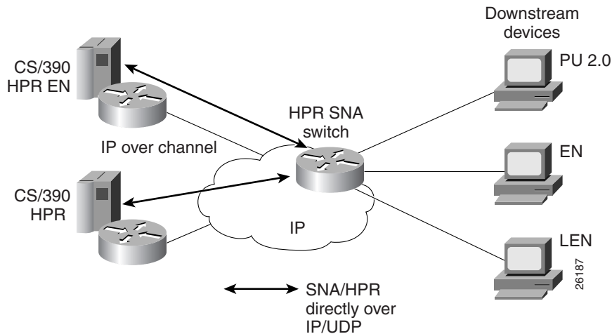
Figure 225 EE Functionality
