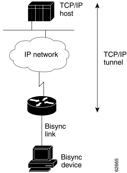
Figure 161 Cisco Router Support of Bisync Devices with BIP
