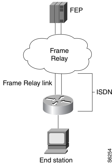
Figure 188 FRAS DLCI Backup over ISDN
