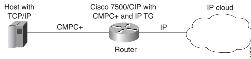
Figure 271 CMPC+ IP with TCP/IP
