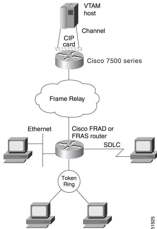
Figure 191 Cisco FRAD Access to a Mainframe through a Cisco 7500
