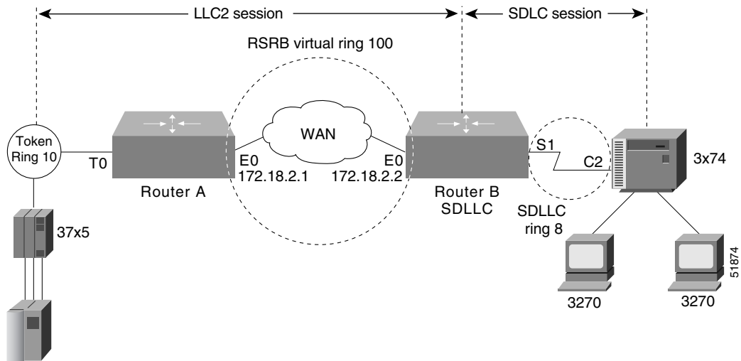
Figure 181 SDLLC with RSRB with a Single 3x74
