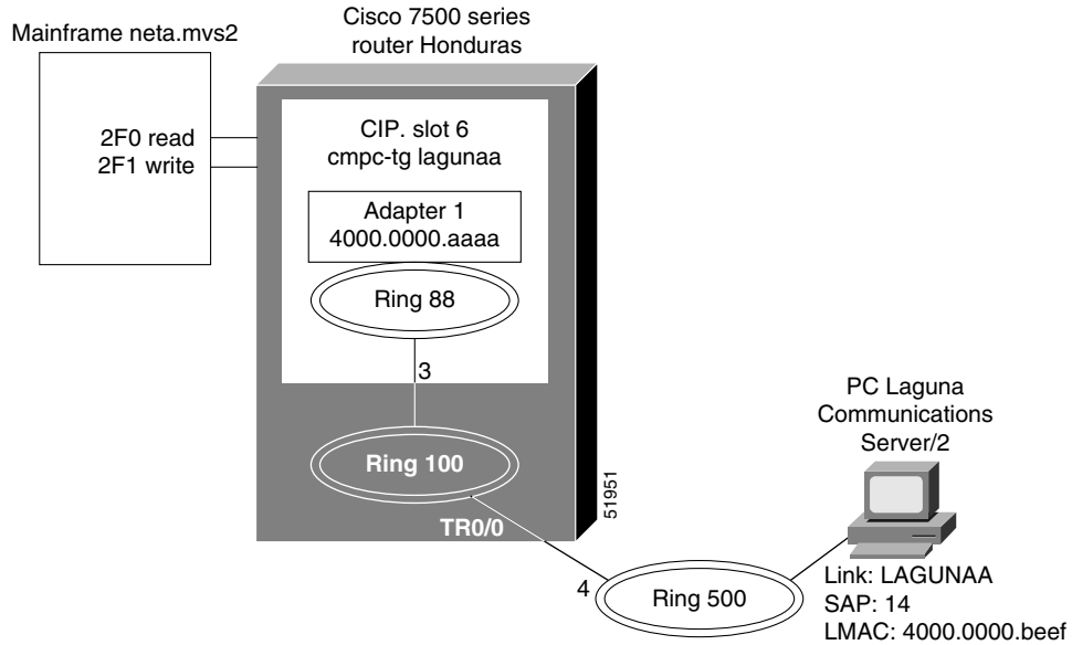
Figure 258 Parameters for VTAM-to-Remote PC with Communications Server/2
