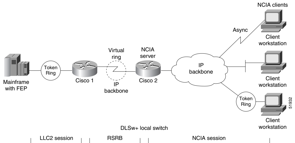
Figure 215 NCIA Server Session with RSRB
