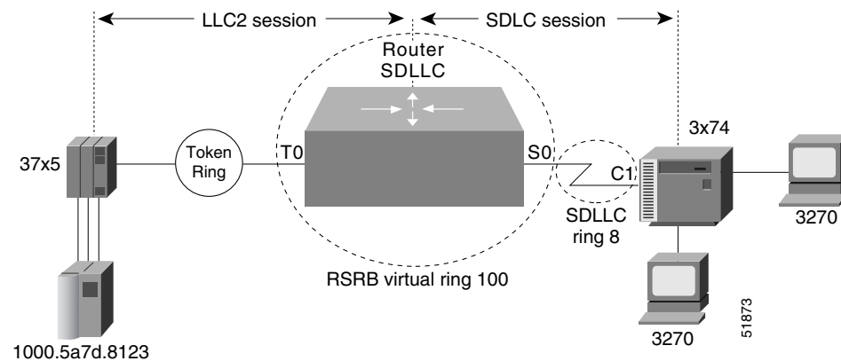
Figure 180 SDLLC with Single Router Using RSRB
