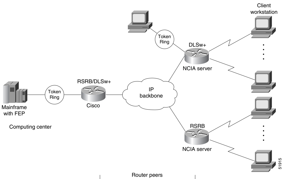
Figure 203 NCIA Server Provides Independence from the Upstream Network Implementation
