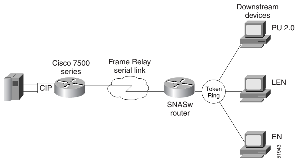
Figure 233 SNASw with SRB Frame Relay (Frame Relay BAN Support)
