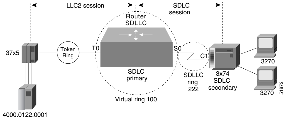
Figure 179 SDLLC Communication Between a 37x5 and a 3x74 Connected to the Same Router (Direct Connection)
