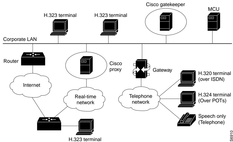
Figure 1-1 H.323 Network
