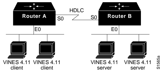
Figure 15-3 VINES Serverless Configuration
