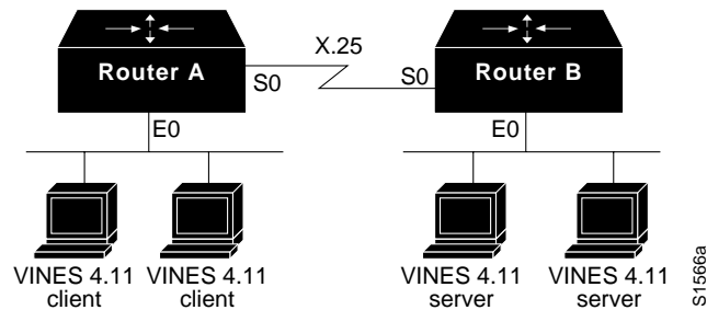
Figure 15-4 VINES Serverless X.25 Configuration
