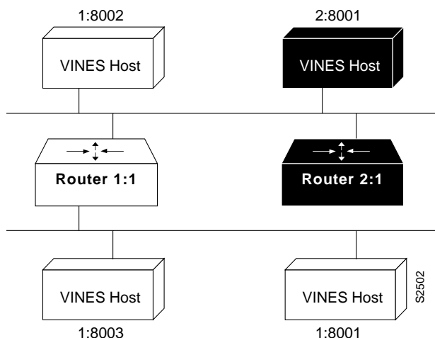
Figure 15-1 VINES Logical Network
