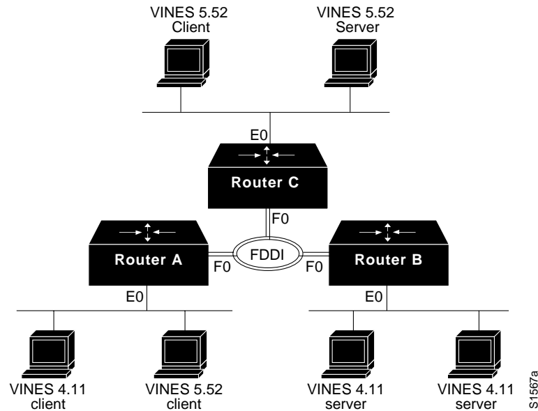
Figure 15-5 VINES Complex Serverless Configuration
