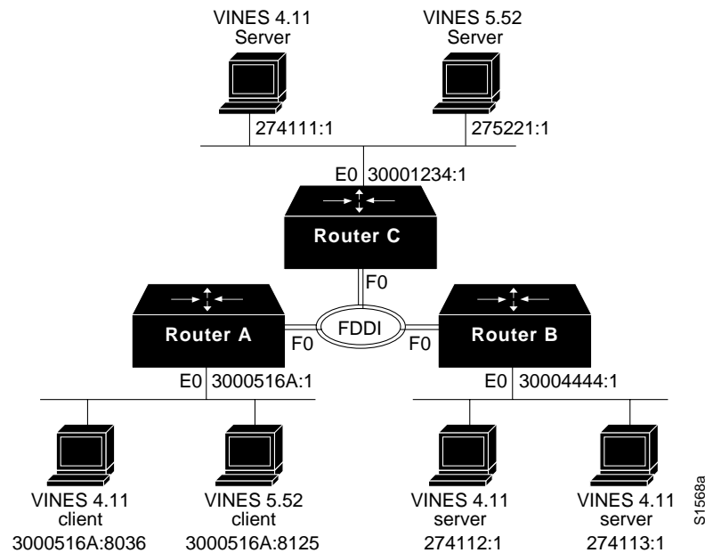
Figure 15-6 VINES Access-List Configuration
