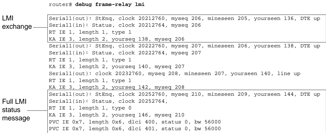
Figure 2-42 Sample Debug Frame-Relay LMI Output
