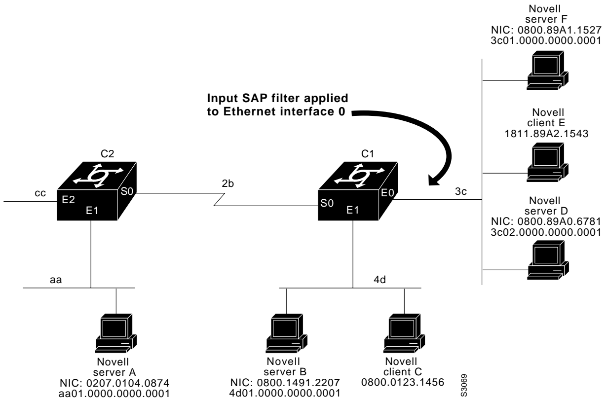
Figure 19-4 SAP Input Filter
