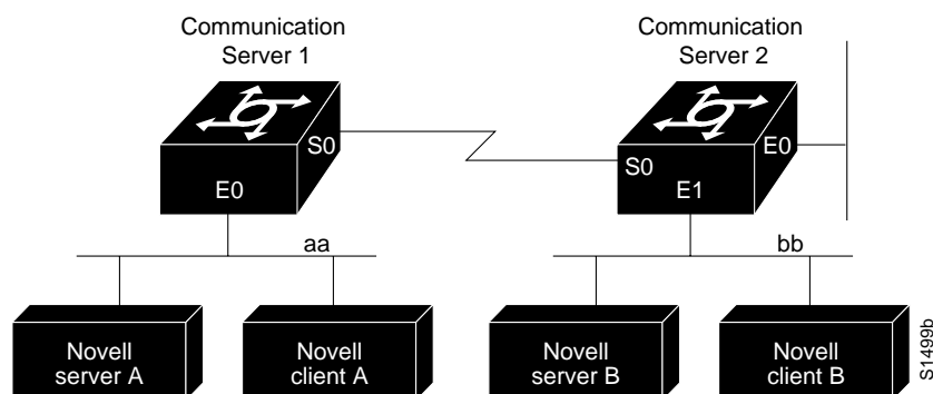
Figure 19-3 Novell IPX Servers Requiring Access Control
