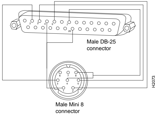
Figure 14-5 Wiring Diagram of a Mini 8-to-DB-25 Cable
