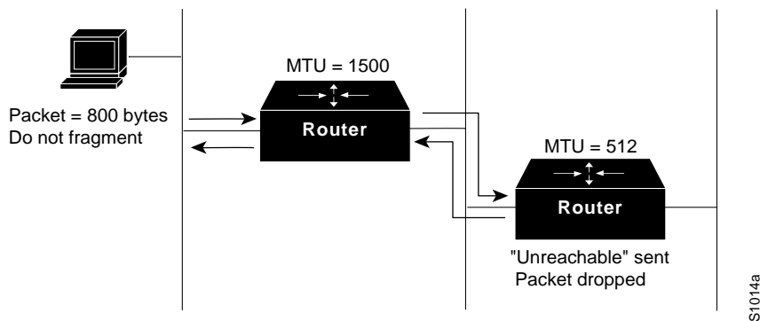
Figure 16-1 IP Path MTU Discovery
