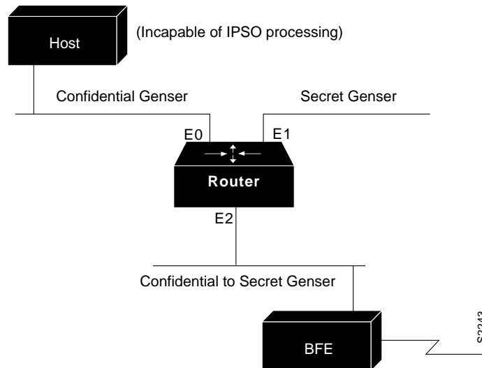
Figure 16-7 IPSO Security Levels
