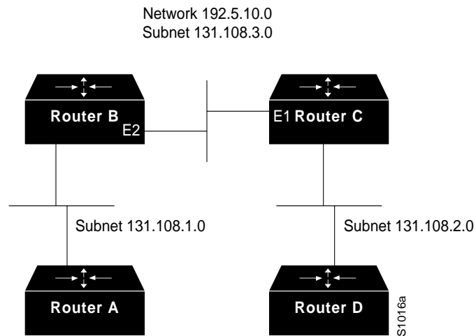
Figure 16-3 Creating a Network from Separated Subnets
