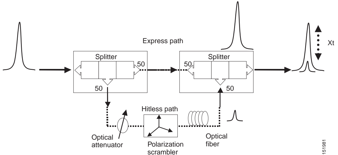
Figure D-4 Generation Block for Single-Interfering Cross-Talk Measurement
