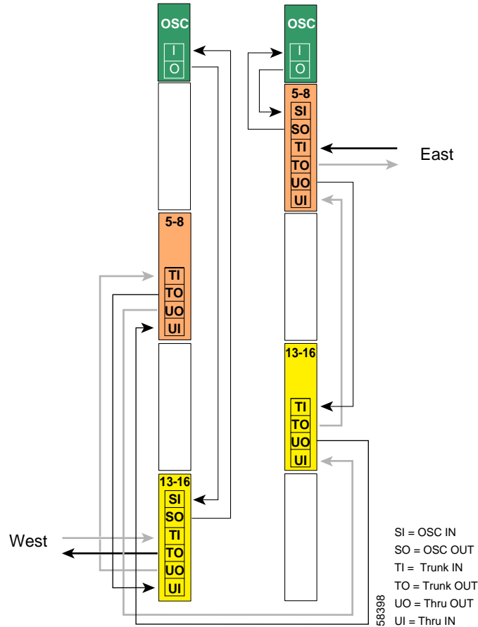
Figure 10-43 Add/Drop Mux/Demux Module Cabling with OSC for Node 3 in Line Card Protected Meshed Ring
