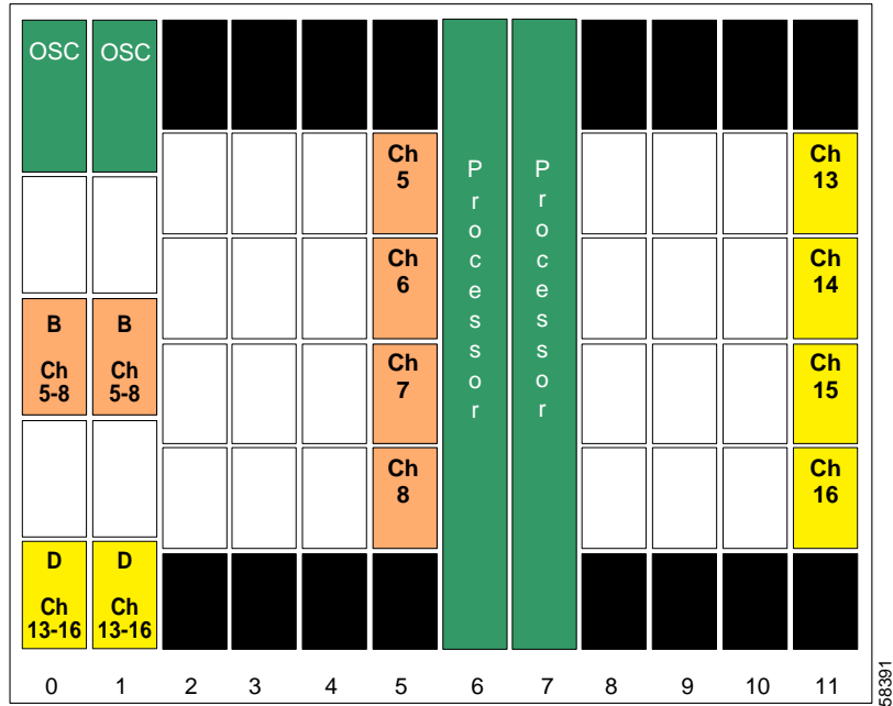
Figure 10-29 Shelf Configuration for Node 3 in Splitter Protected Meshed Ring
