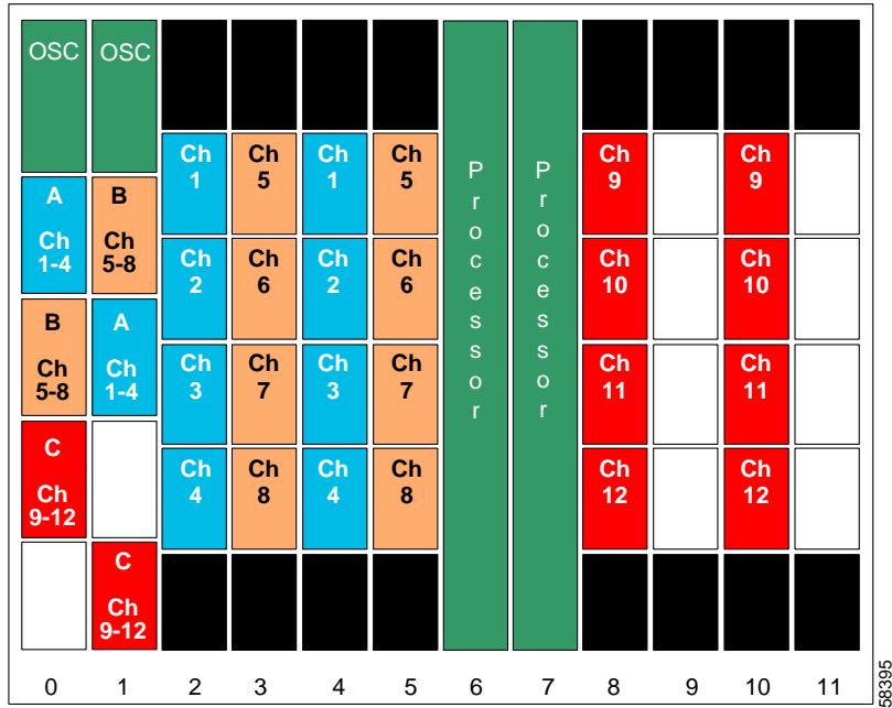
Figure 10-38 Shelf Configuration for Node 1 in Line Card Protected Meshed Ring
