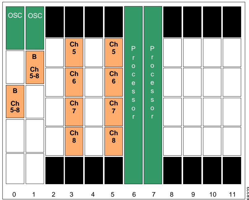
Figure 10-18 Shelf Configuration for Node 3 in Line Card Protected Hubbed Ring
