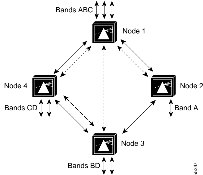
Figure 10-2 Meshed Ring Topology Example
