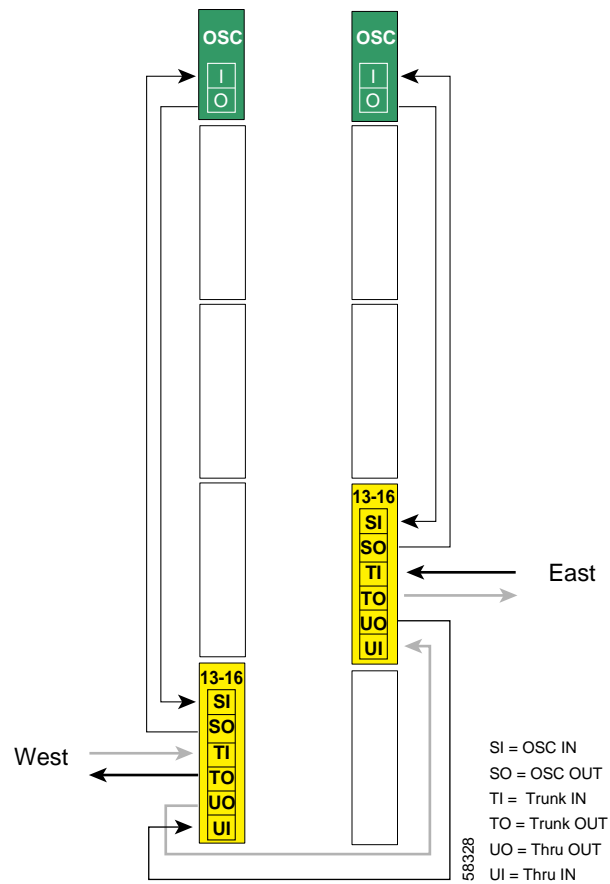
Figure 10-23 Add/Drop Mux/Demux Module Cabling with OSC for Node 5 in Line Card Protected Hubbed Ring
