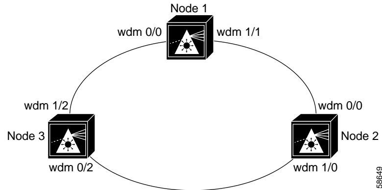
Figure 11-2 Ring Topology Example
