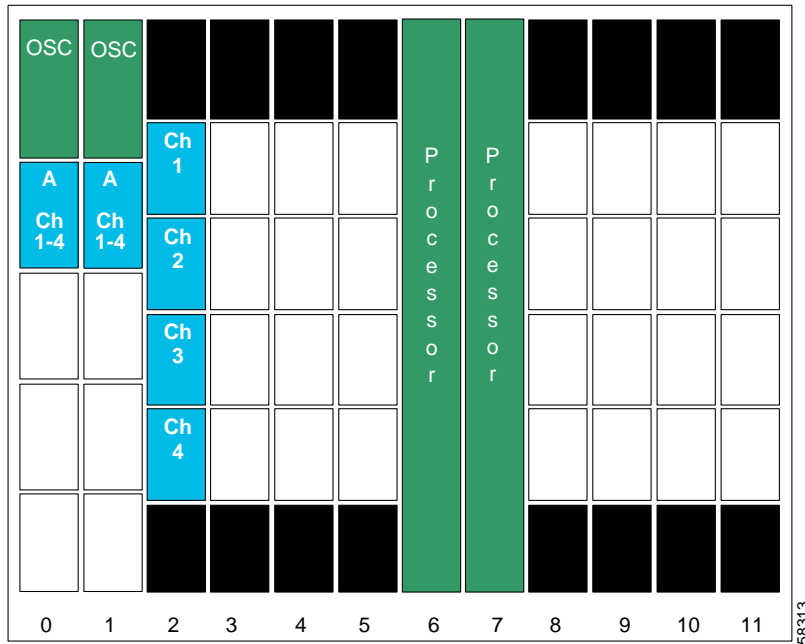
Figure 10-6 Shelf Configuration for Node 2 in Splitter Protected Hubbed Ring
