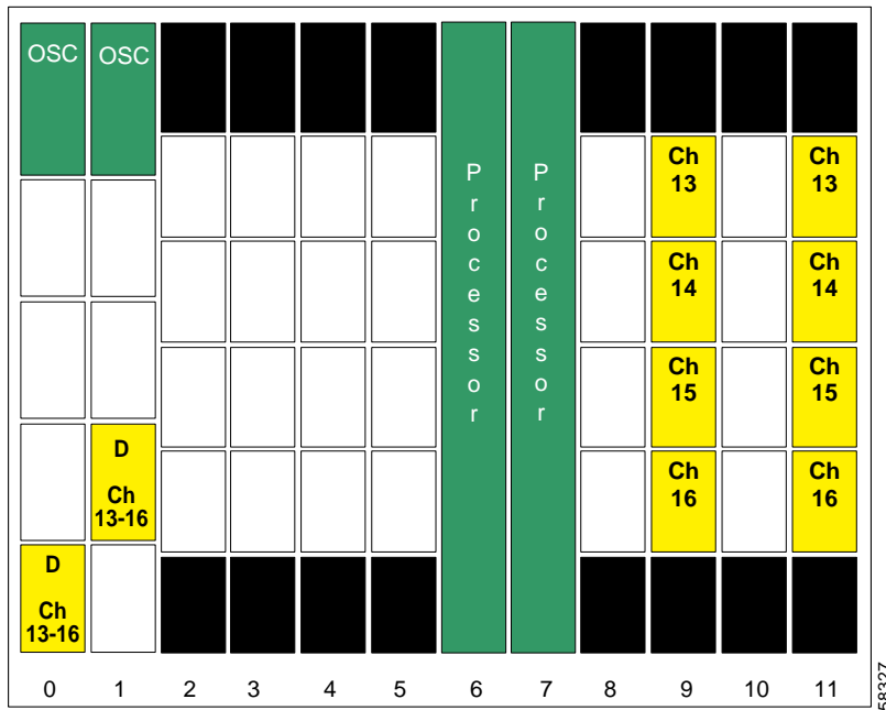
Figure 10-22 Shelf Configuration for Node 5 in Line Card Protected Hubbed Ring
