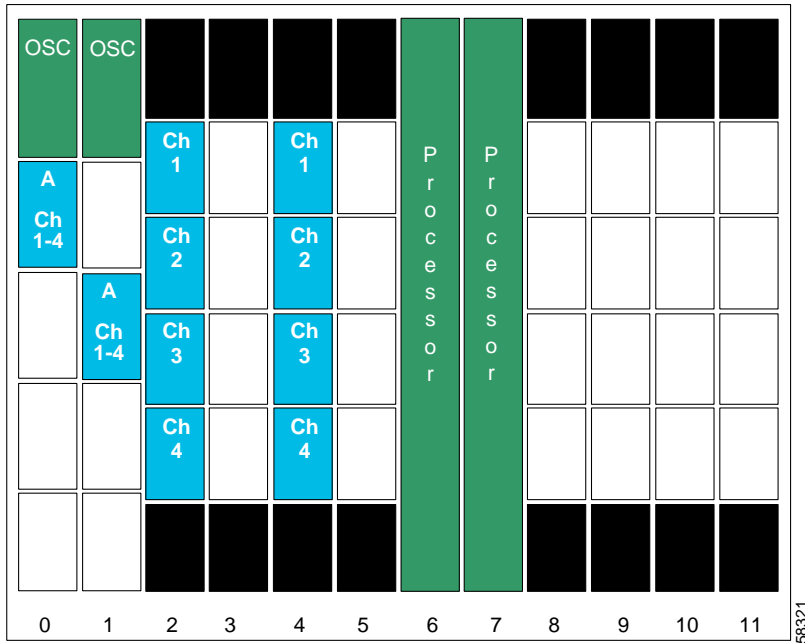
Figure 10-40 Shelf Configuration for Node 2 in Line Card Protected Meshed Ring
