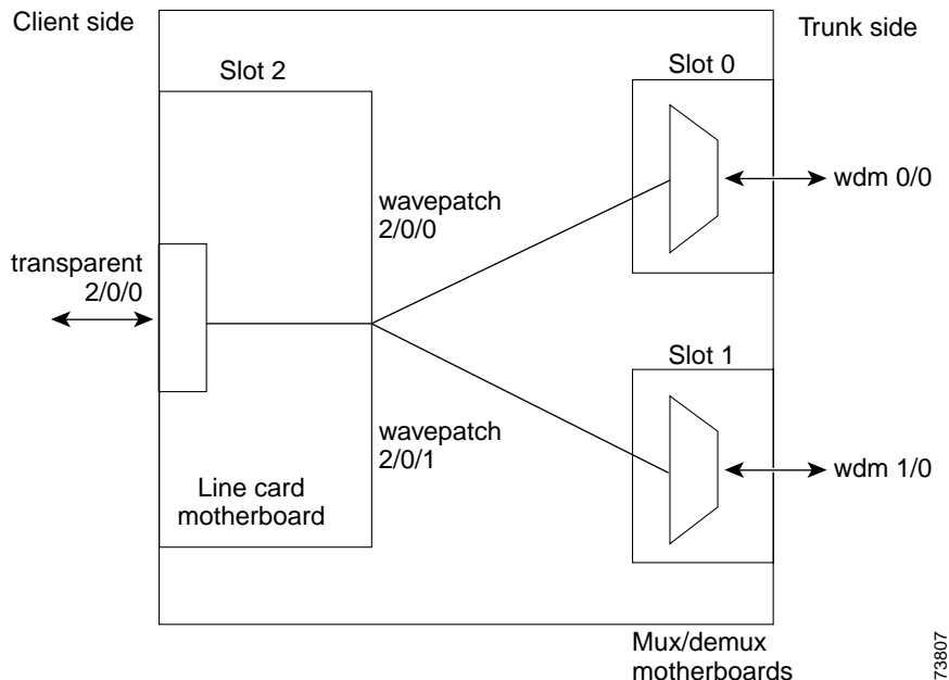
Figure 7-1 Splitter Protection Scheme with 2.5-Gbps Transponder Module
