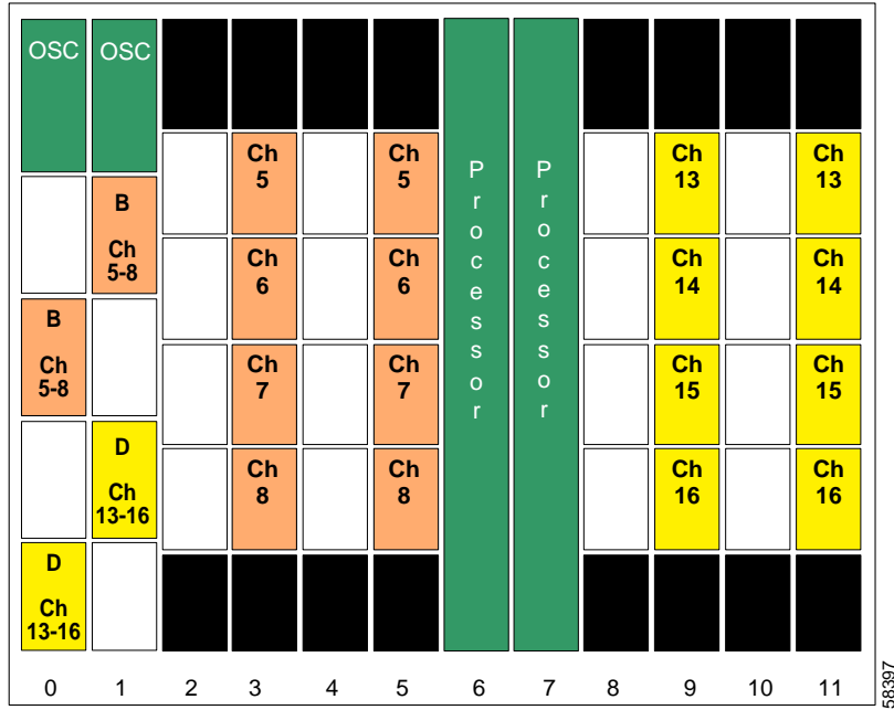
Figure 10-42 Shelf Configuration for Node 3 in Line Card Protected Meshed Ring
