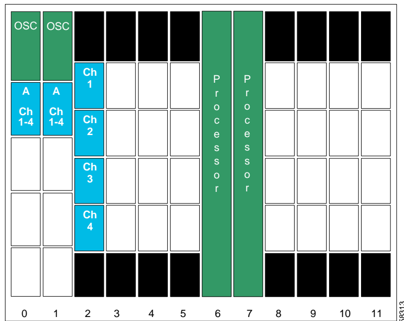
Figure 10-27 Shelf Configuration for Node 2 in Splitter Protected Meshed Ring
