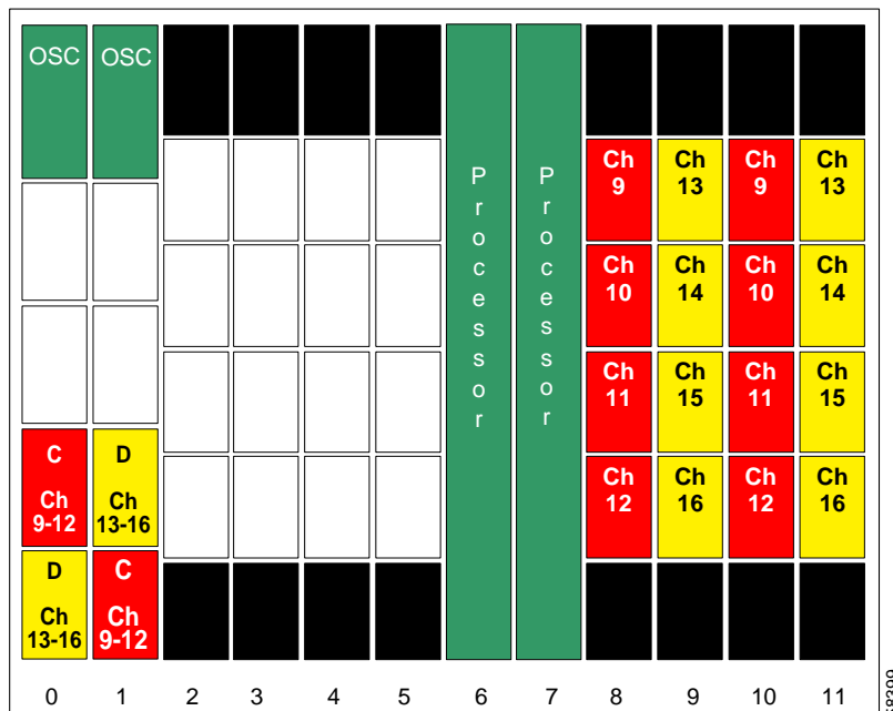
Figure 10-44 Shelf Configuration for Node 4 in Line Card Protected Meshed Ring
