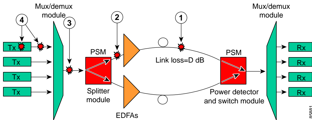
Figure 6-2 Point-to-Point Topology with Post-Amplification
