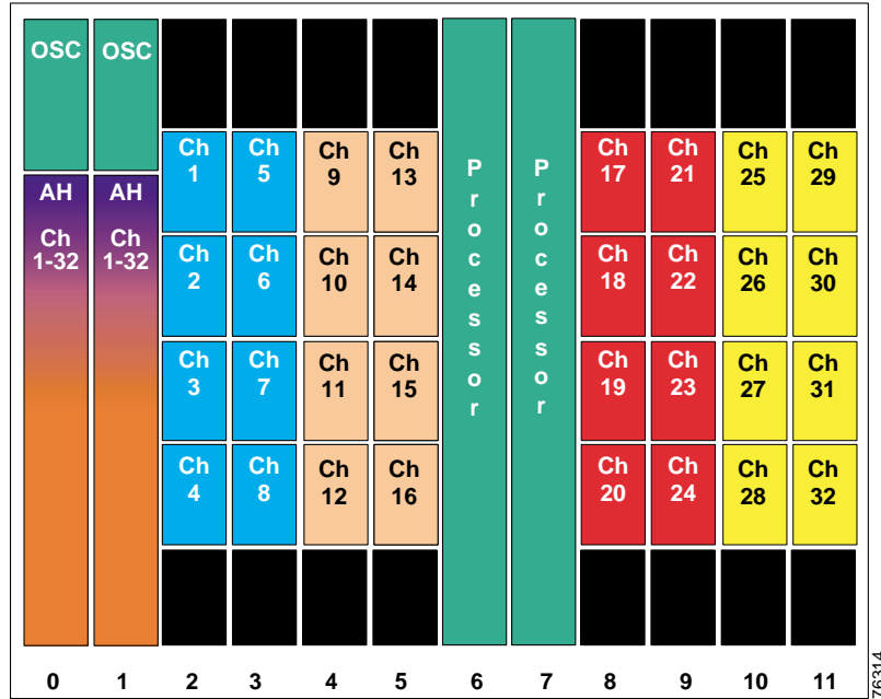
Figure 9-3 Shelf Configuration for Splitter Protected 32-Channel Point-to-Point Topology
