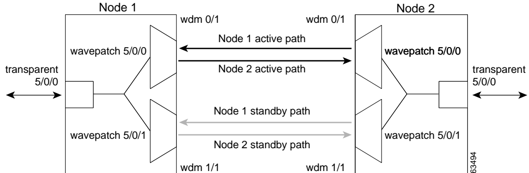
Figure 7-7 Bidirectional Path Switching Example with Splitter Protection
