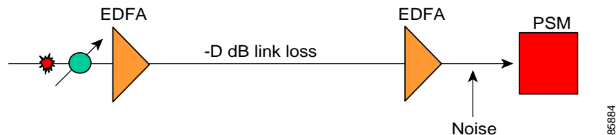
Figure 6-4 Failure Scenario with Noise from Two EDFAs
