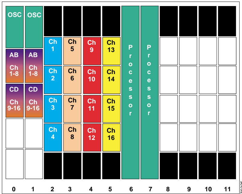
Figure 10-4 Shelf Configuration for 16-Channel Hub Node in Splitter Protected Hubbed Ring
