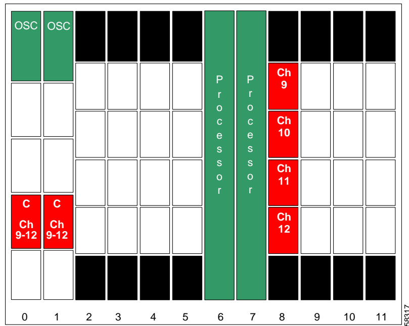
Figure 10-10 Shelf Configuration for Node 4 in Splitter Protected Hubbed Ring
