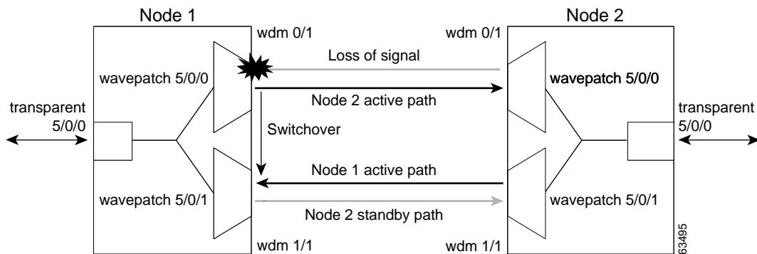
Figure 7-5 Unidirectional Path Switching Example
