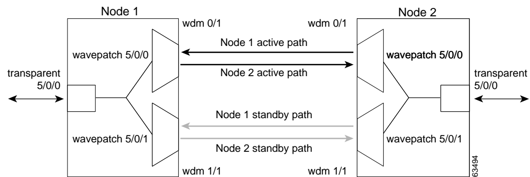
Figure 7-4 Active and Standby Path Configuration Example
