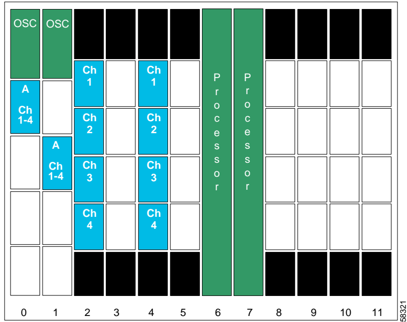
Figure 10-16 Shelf Configuration for Node 2 in Line Card Protected Hubbed Ring
