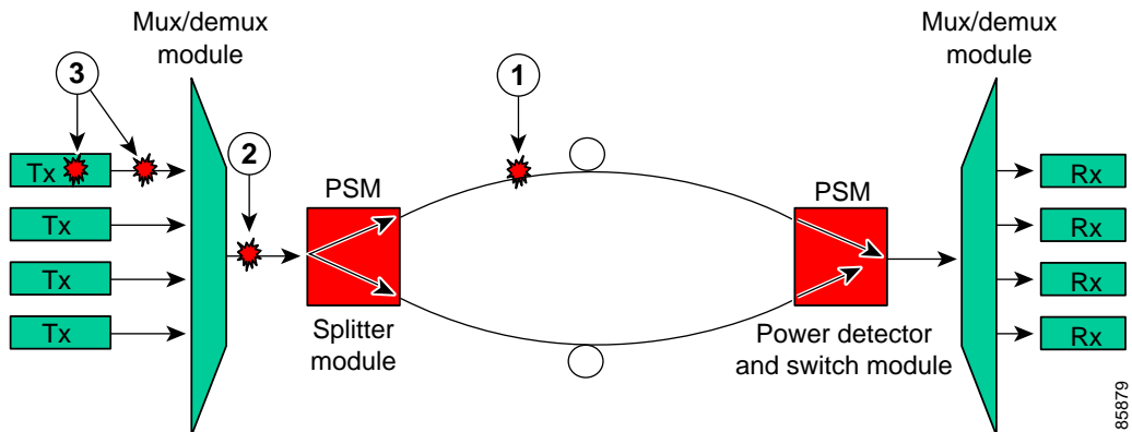
Figure 6-1 Point-to-Point Topology Without Amplification
