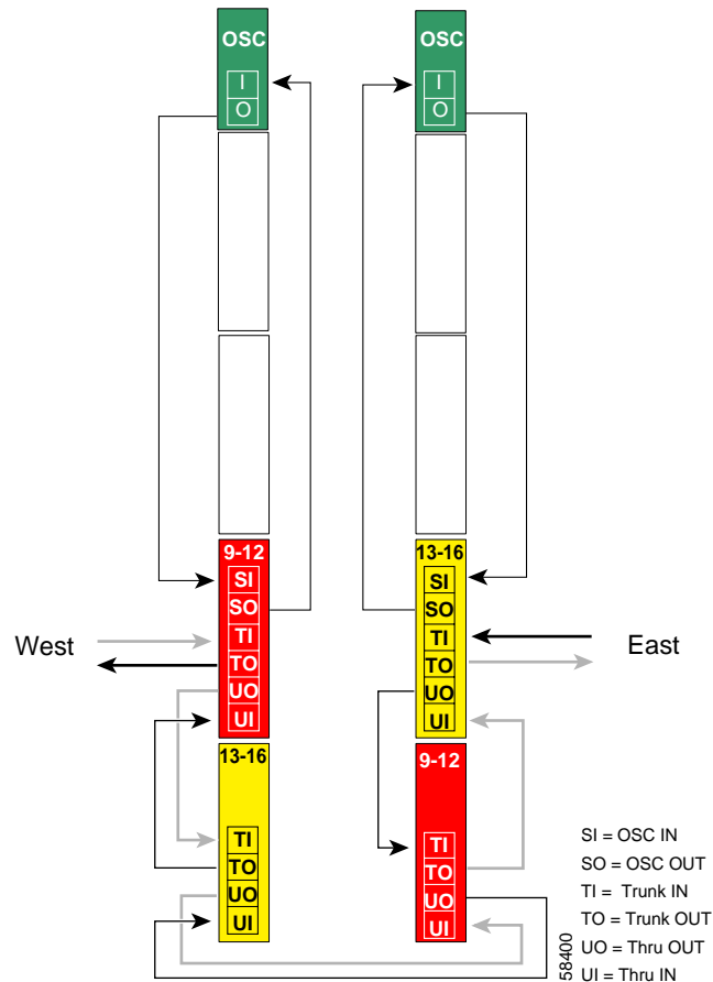
Figure 10-45 Add/Drop Mux/Demux Module Cabling with OSC for Node 4 in Line Card Protected Meshed Ring
