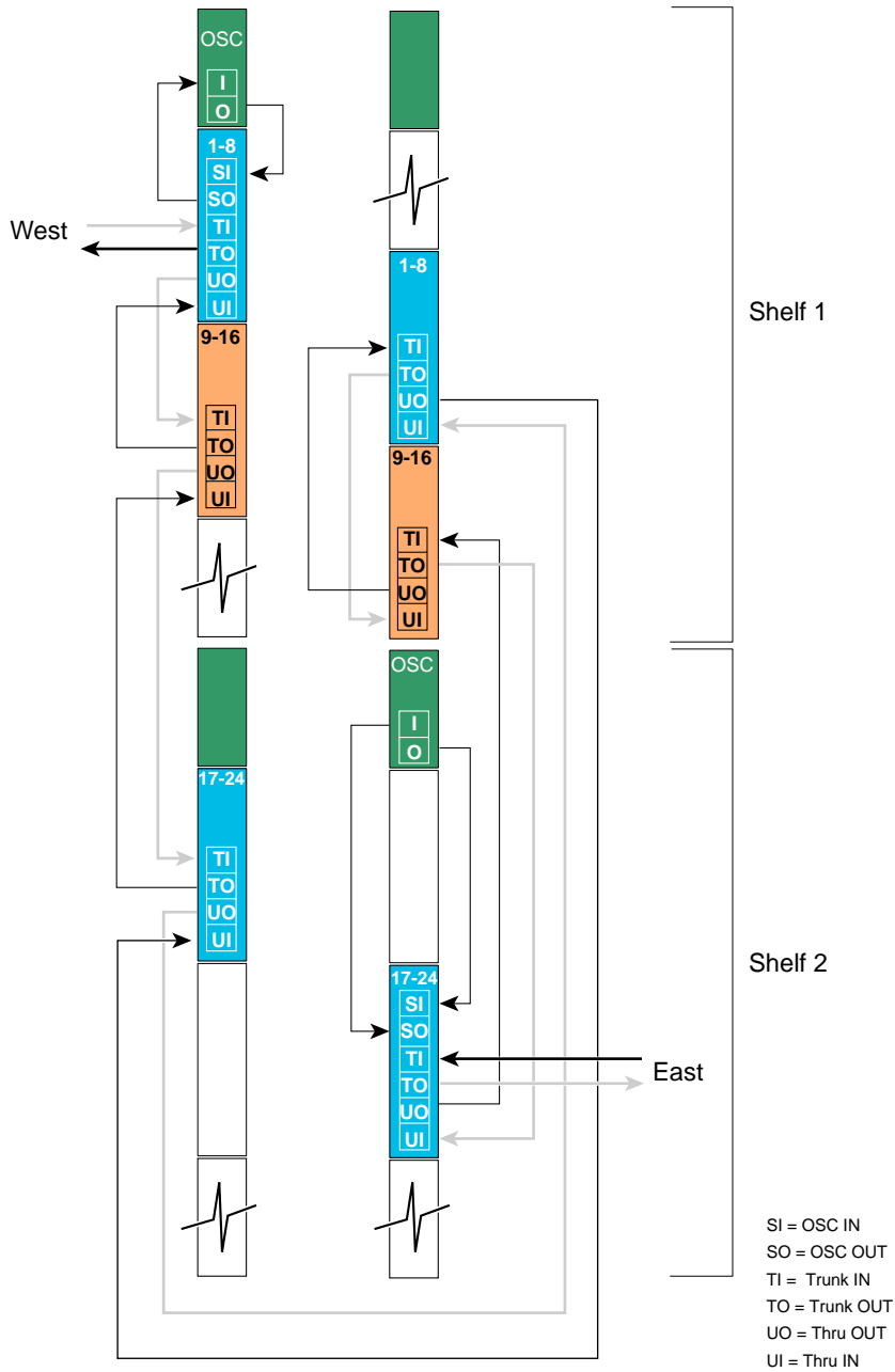
Figure 8-3 Add/Drop Mux/Demux Module Cabling with Two Shelves with 24 Channels and Line Card Protection
