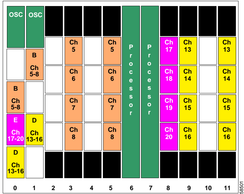
Figure 10-48 Shelf Configuration for Node 3 in Line Card Protected Meshed Ring with Unprotected Channels
