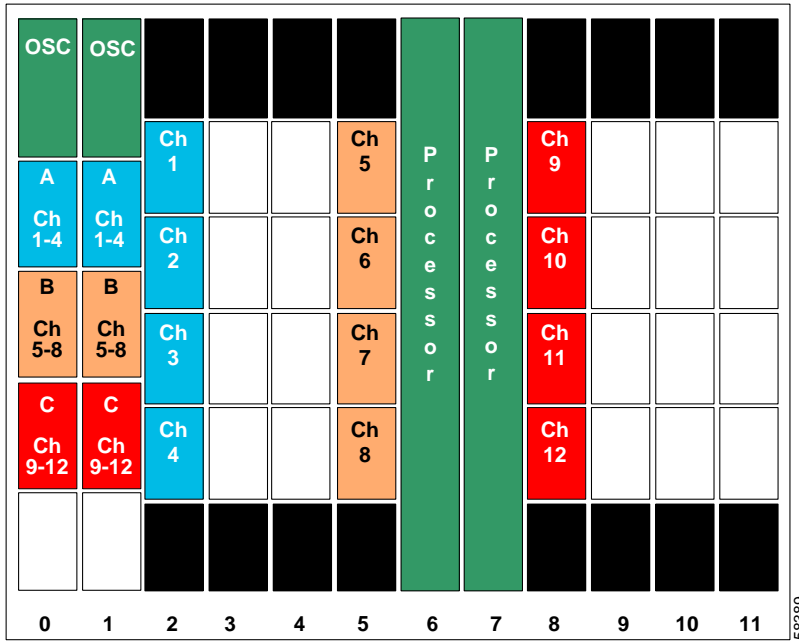
Figure 10-25 Shelf Configuration for Node 1 in Splitter Protected Meshed Ring
