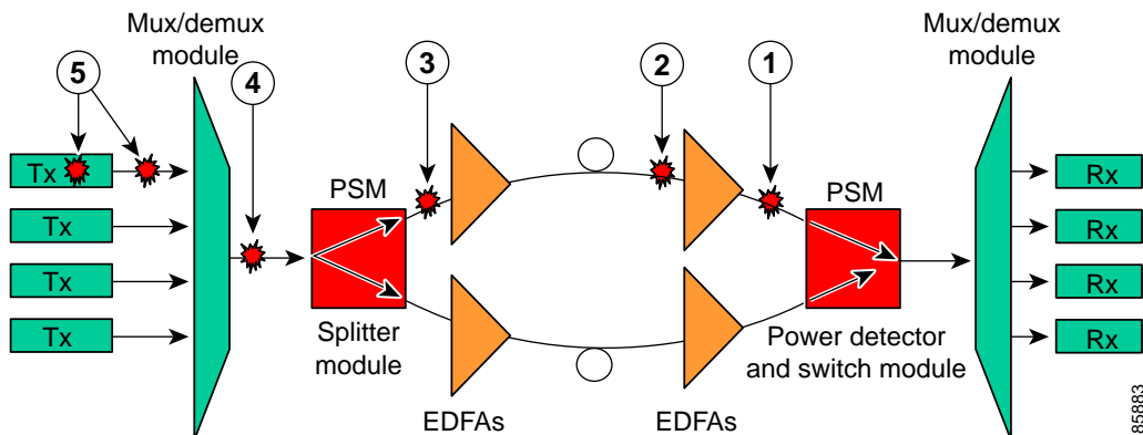
Figure 6-3 Point-to-point Topology with Post-Amplification and Pre-Amplification
