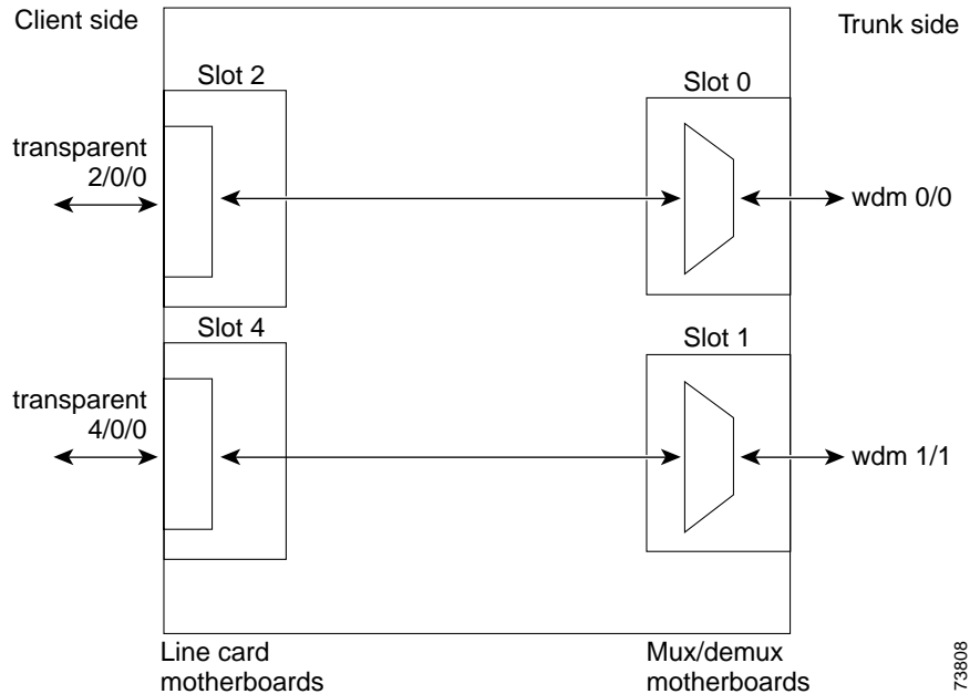
Figure 7-2 Line Card Protection Scheme with 2.5-Gbps Transponder Module
