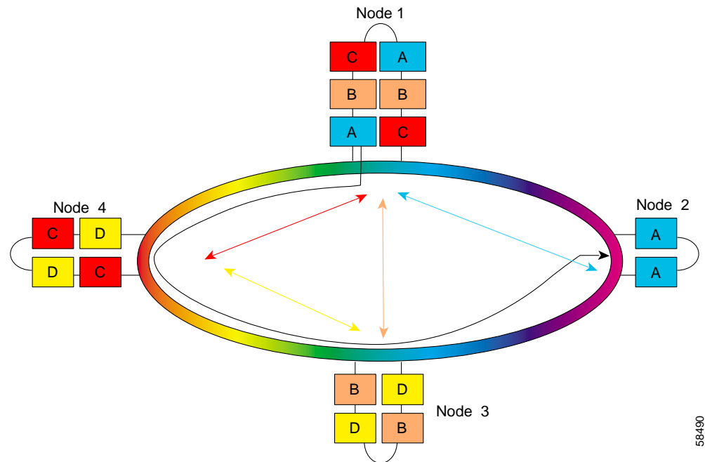
Figure 10-24 Channel Plan for Meshed Ring
