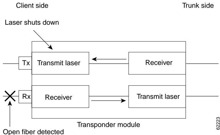
Figure 4-2 OFC Overview
