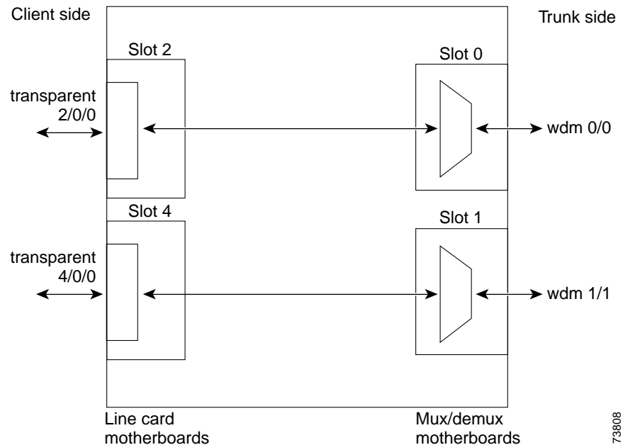
Figure 5-2 Line Card Protection Scheme with 2.5-Gbps Transponder Module
