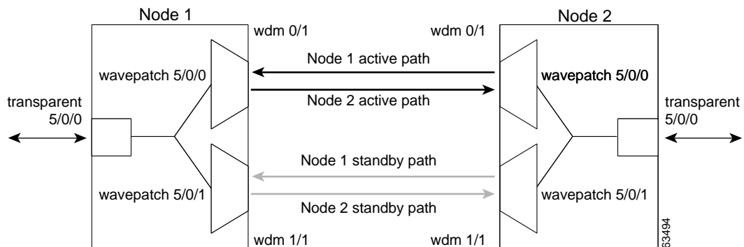
Figure 5-3 Active and Standby Path Configuration Example
