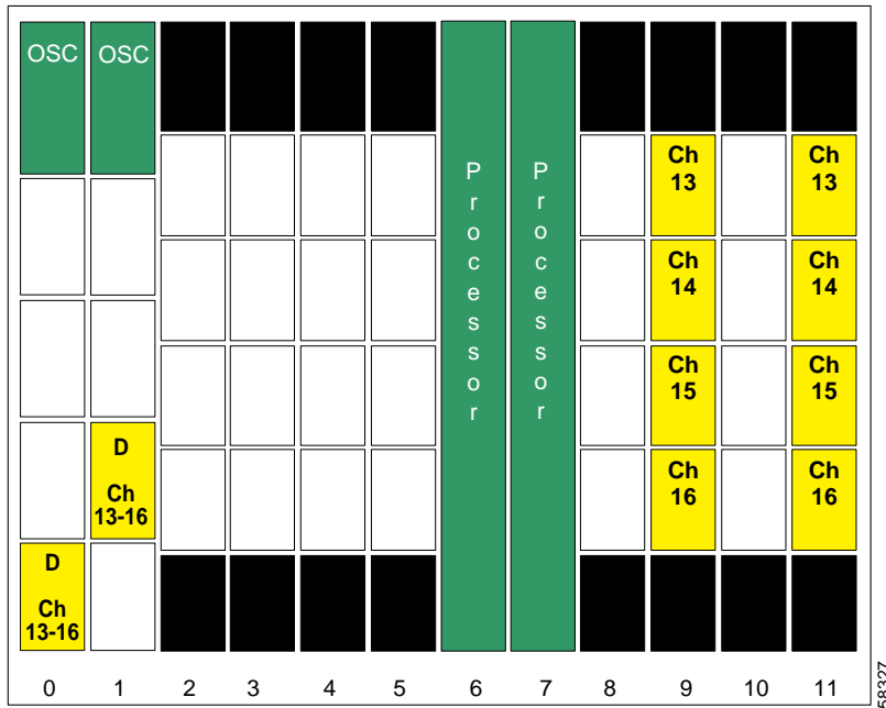
Figure 8-22 Shelf Configuration for Node 5 in Line Card Protected Hubbed Ring
