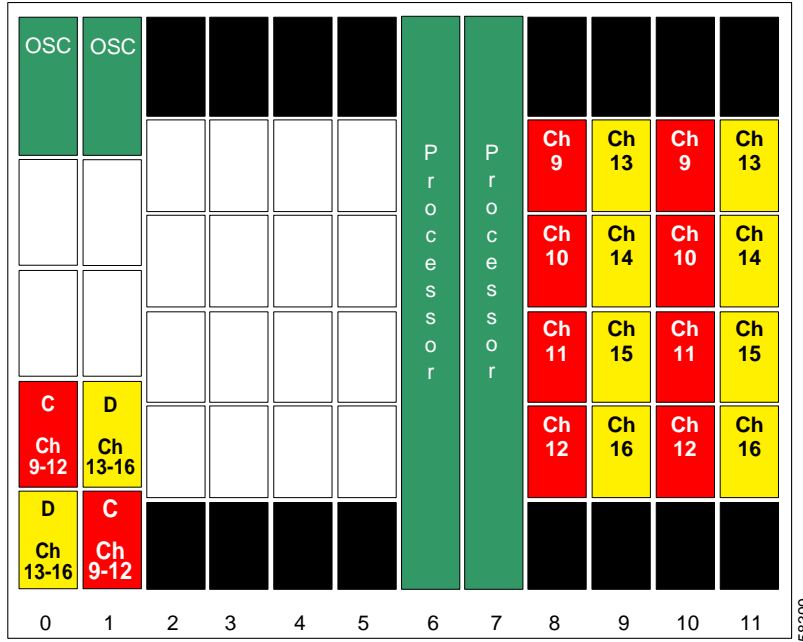
Figure 8-44 Shelf Configuration for Node 4 in Line Card Protected Meshed Ring
