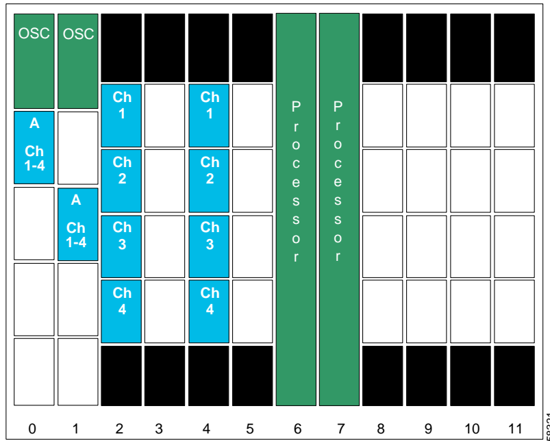
Figure 8-16 Shelf Configuration for Node 2 in Line Card Protected Hubbed Ring
