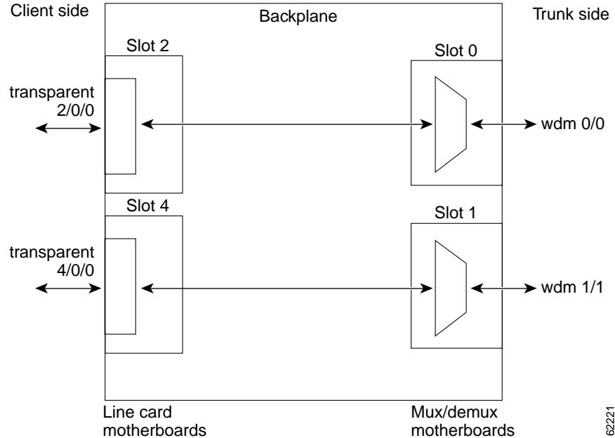
Figure 5-2 Line Card Protection Scheme
