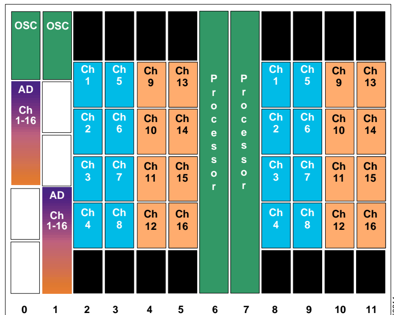
Figure 7-5 Shelf Configuration for Line Card Protected 32-Channel Point-to-Point Topology
