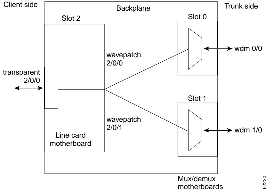
Figure 5-1 Splitter Protection Scheme
