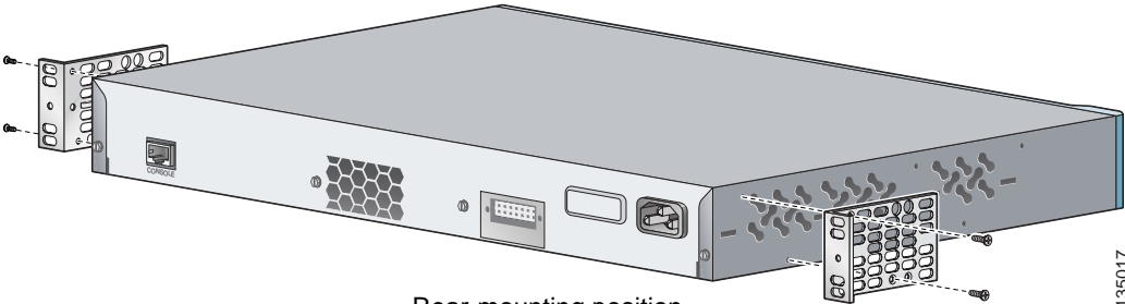
Rear-mounting position
