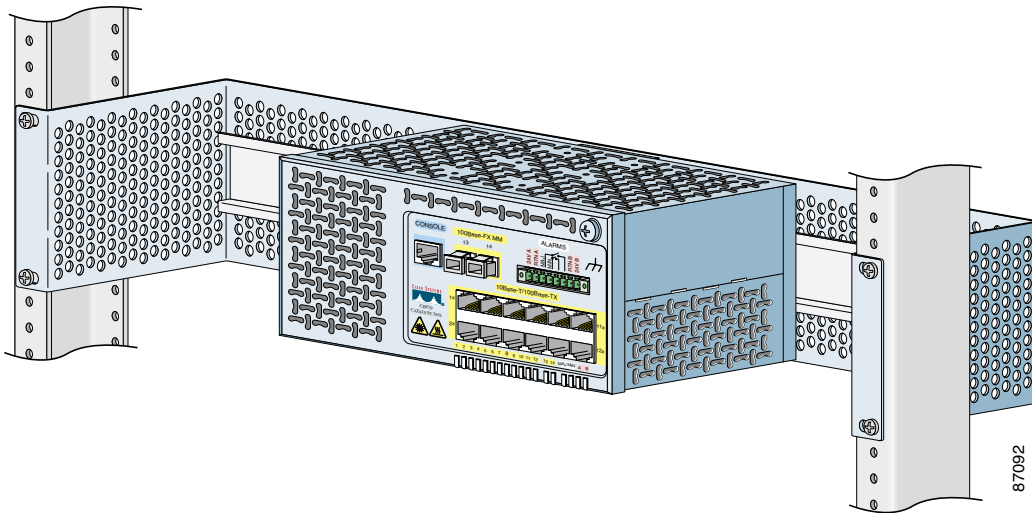
Figure 3-31 Installing the Switch in a Rack
