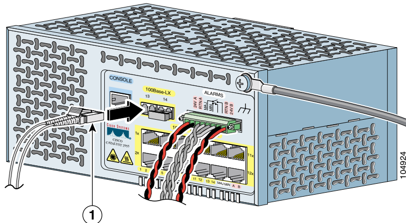
Figure 4-29 Connecting to a 100BASE-LX SM Port
