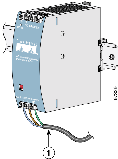
Figure 3-17 Connecting AC Power to the Power Converter
