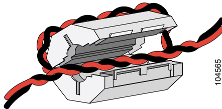
Figure 4-10 Wire Looped Through the Ferrite
