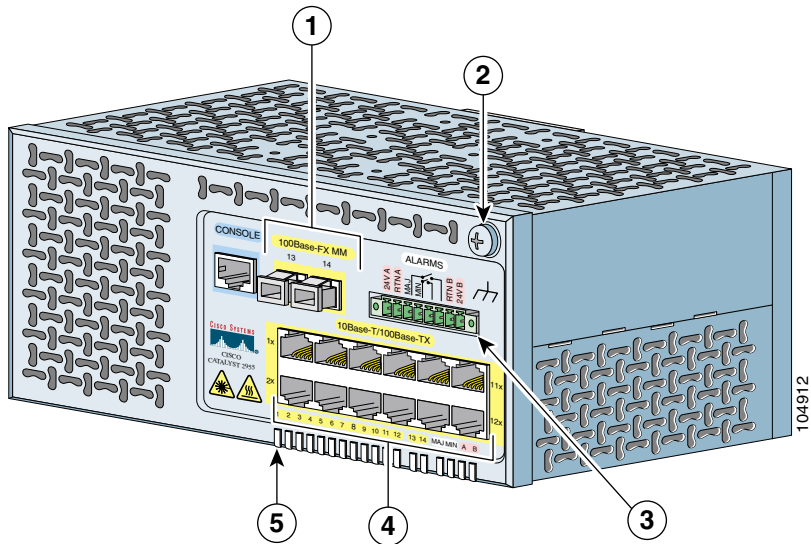
Figure 2-2 Catalyst 2955C-12 Switch
