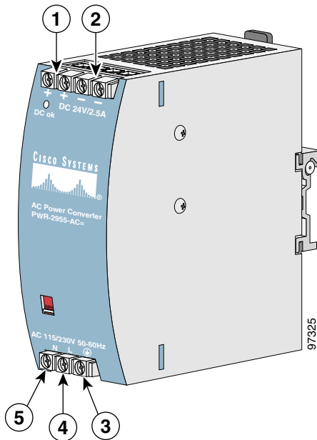
Figure 10 The Catalyst 2955 Switch AC/DC Power Converter
