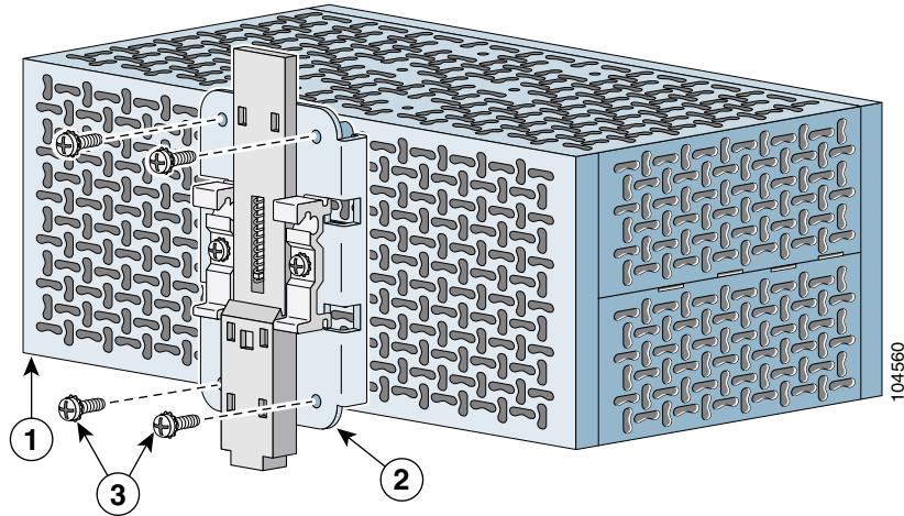
Figure 4-16 Catalyst 2955 Switch Rear Panel Clip Mounting
