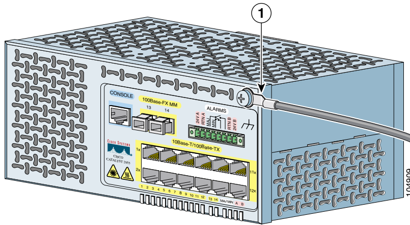
Figure 4-4 Torquing Ground-Lug Screws
