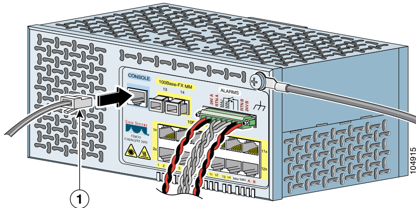
Figure 3-1 Connecting to the Console Port
