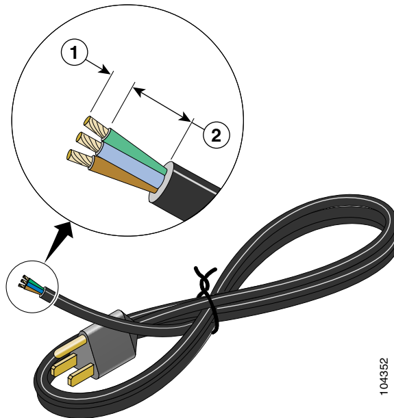
Figure 3-15 Preparing the AC Power Cord
