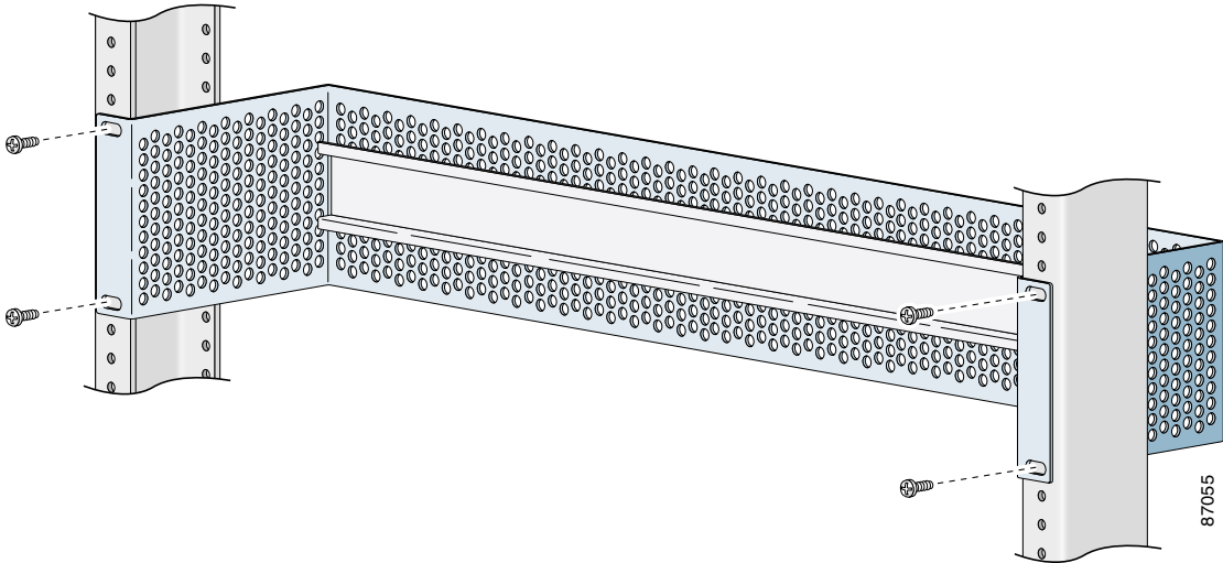
Figure 4-20 Installing the DIN Rail Adapter
