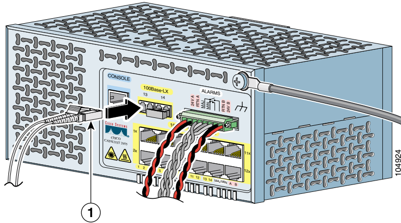
Figure 3-39 Connecting to a 100BASE-LX SM Port
