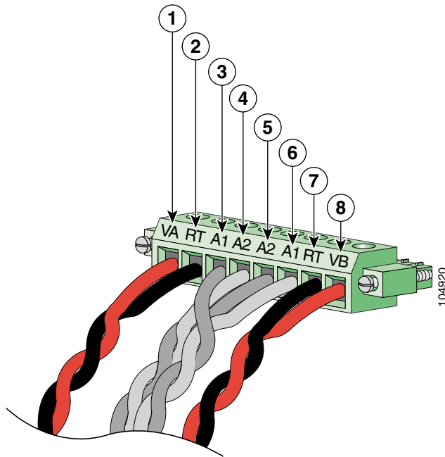
Figure 4-15 Completed Connections for Two External Alarm Devices on the Power and Relay Connector
