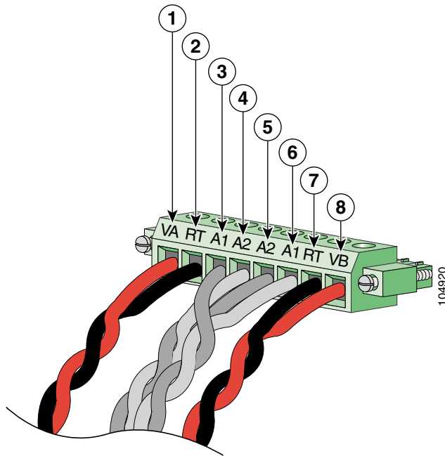
Figure 3-25 Completed Connections for Two External Alarm Devices on the Power and Relay Connector
