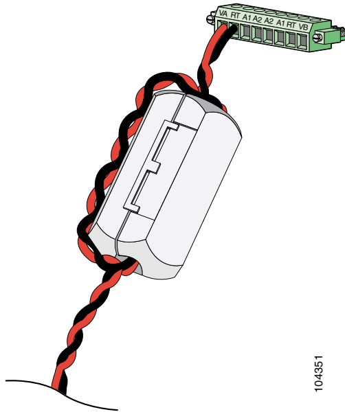
Figure 3-11 Clasping the Ferrite
