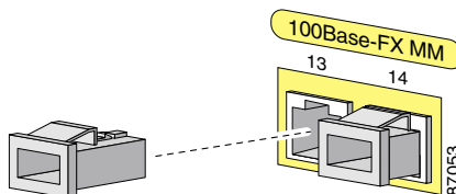
Figure 4-26 Removing Dust Plugs from 100BASE-FX Ports
