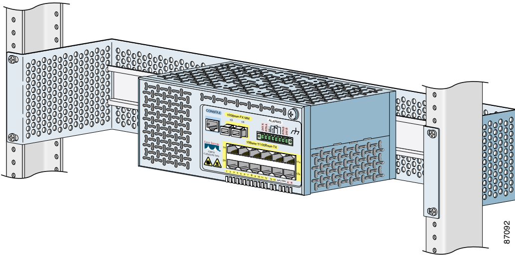
Figure 4-21 Installing the Switch in a Rack
