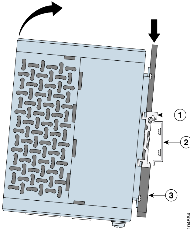
Figure 3-33 Removing the Switch from a Face-Down Mounting Position
