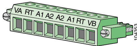
Figure 3-5 Power and Relay Connector
