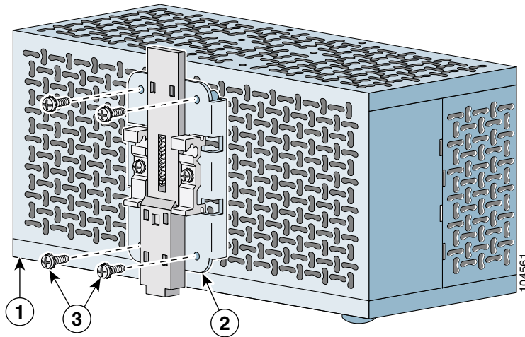
Figure 4-17 Catalyst 2955 Switch Top Panel Clip Mounting
