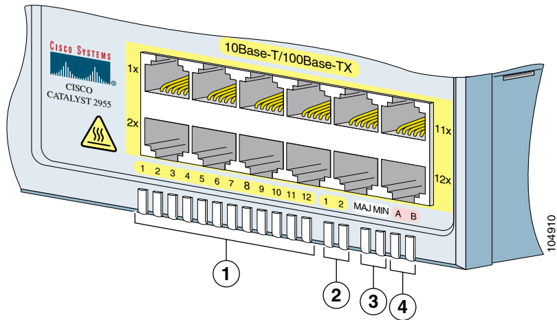
Figure 2-7 LEDs on the Catalyst 2955T-12 Switch
