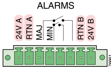
Figure B-5 Power and Relay Connector
