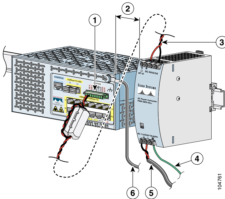
Figure 3-21 The Power Converter Connected to the Catalyst 2955 Switch and a DC Power Source
