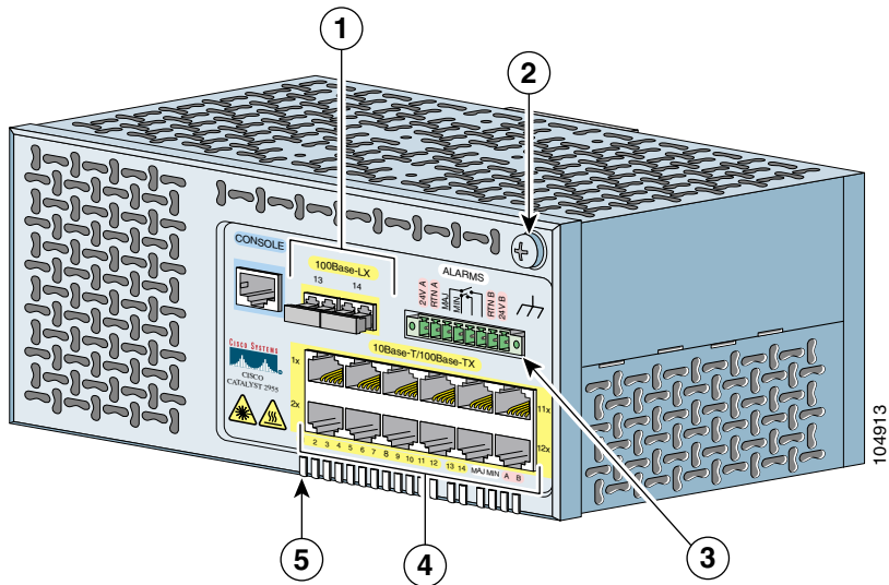
Figure 2-3 Catalyst 2955S-12 Switch
