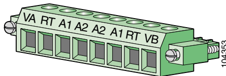
Figure 2-6 Power and Relay Connector
