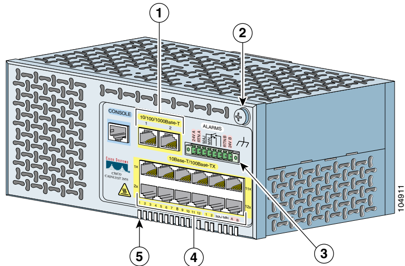
Figure 2-1 Catalyst 2955T-12 Switch
