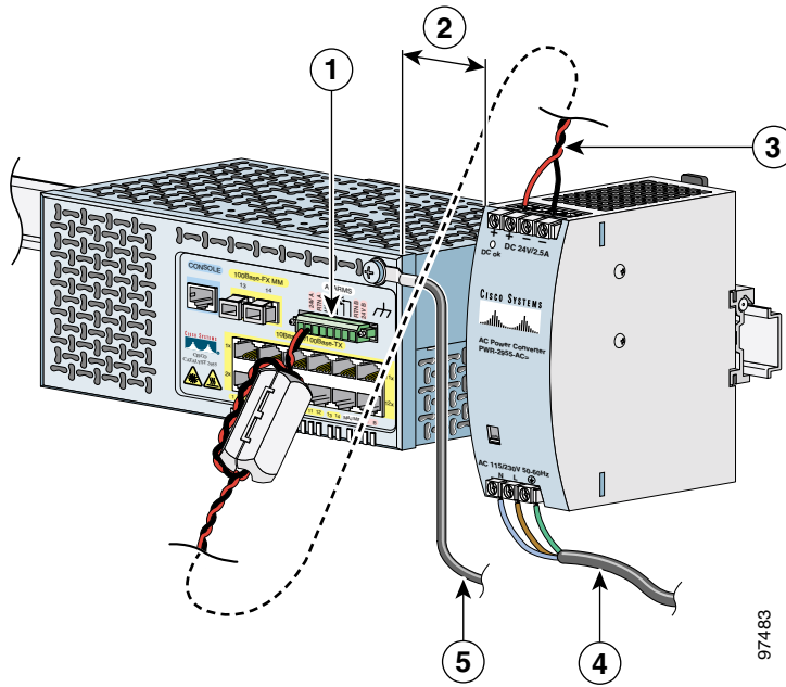
Figure 3-18 The Power Converter Connected to the Catalyst 2955 Switch and an AC Power Source
