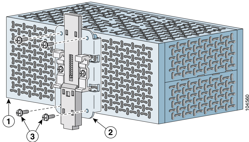
Figure 2-9 Catalyst 2955 Switch Rear Panel
