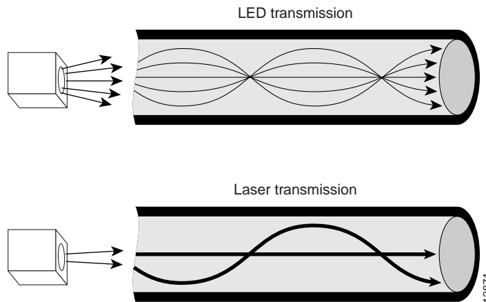
Figure E-1 LED Transmission Compared to Laser Transmission
