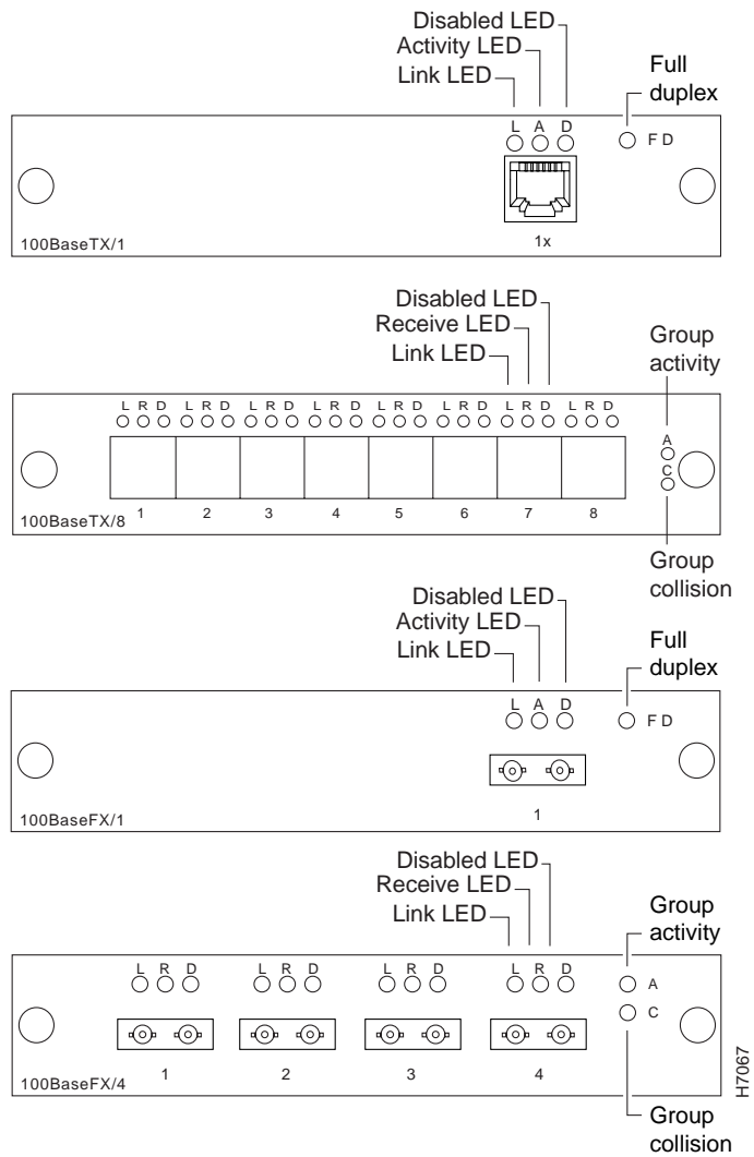
Figure 1-2 100BaseT Modules
