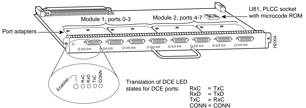
Figure 1 Fast Serial Interface Processor
