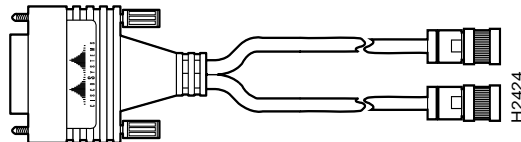
Figure 7 E1-G.703/G.704 Interface Cable for Balanced Connections (with Twinax Connectors and Cables)
