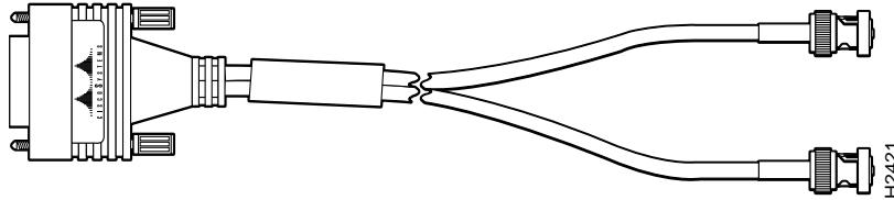
Figure 6 E1-G.703/G.704 Interface Cable for Balanced Connections (with DB-15 Connectors on Both Ends)
