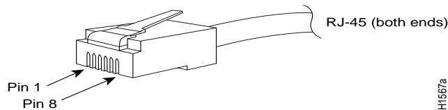
Figure 2-2 CDDI Interface Connector—RJ-45 Type
