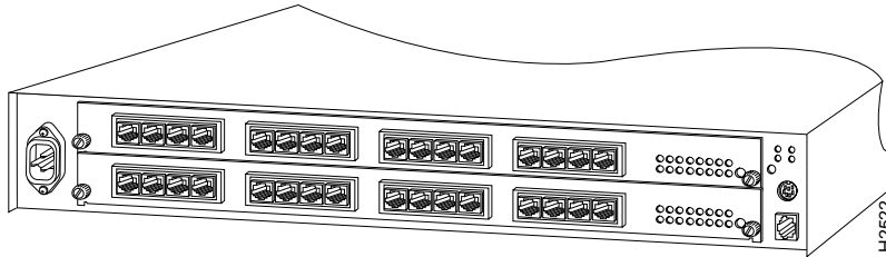
Figure 1-7 Concentrator with CDDI Line Cards Installed—Rear-Panel View
