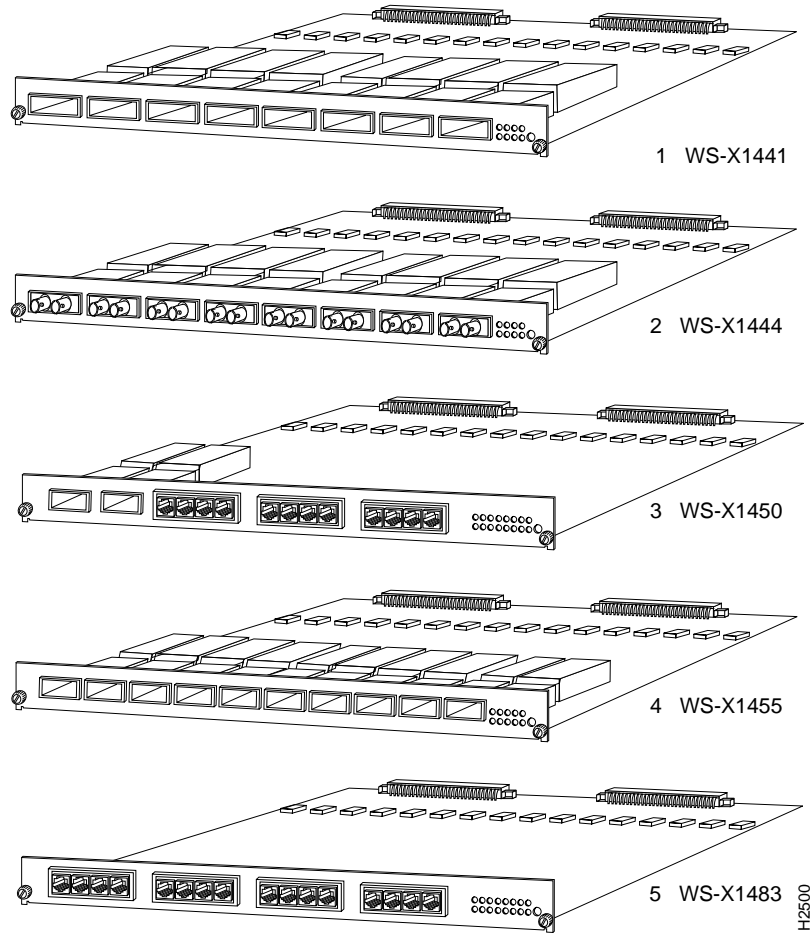
Figure 1-6 CDDI and FDDI Line Cards
