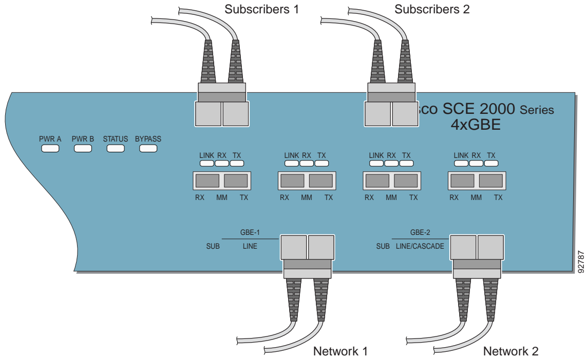
Figure 5-4 Cabling Diagram: Dual Link One SCE Platform Receive-only
