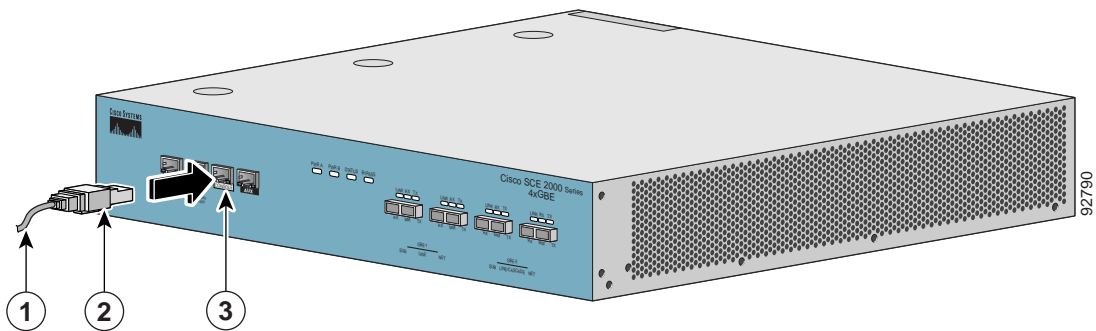
Figure 4-1 Connecting to the Local Console
