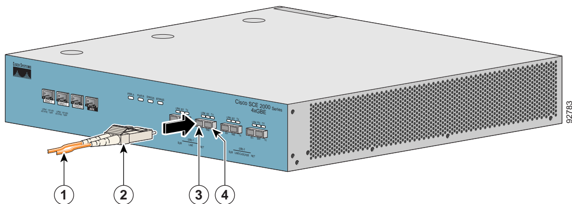
Figure 5-6 Cabling the GBE Interface
