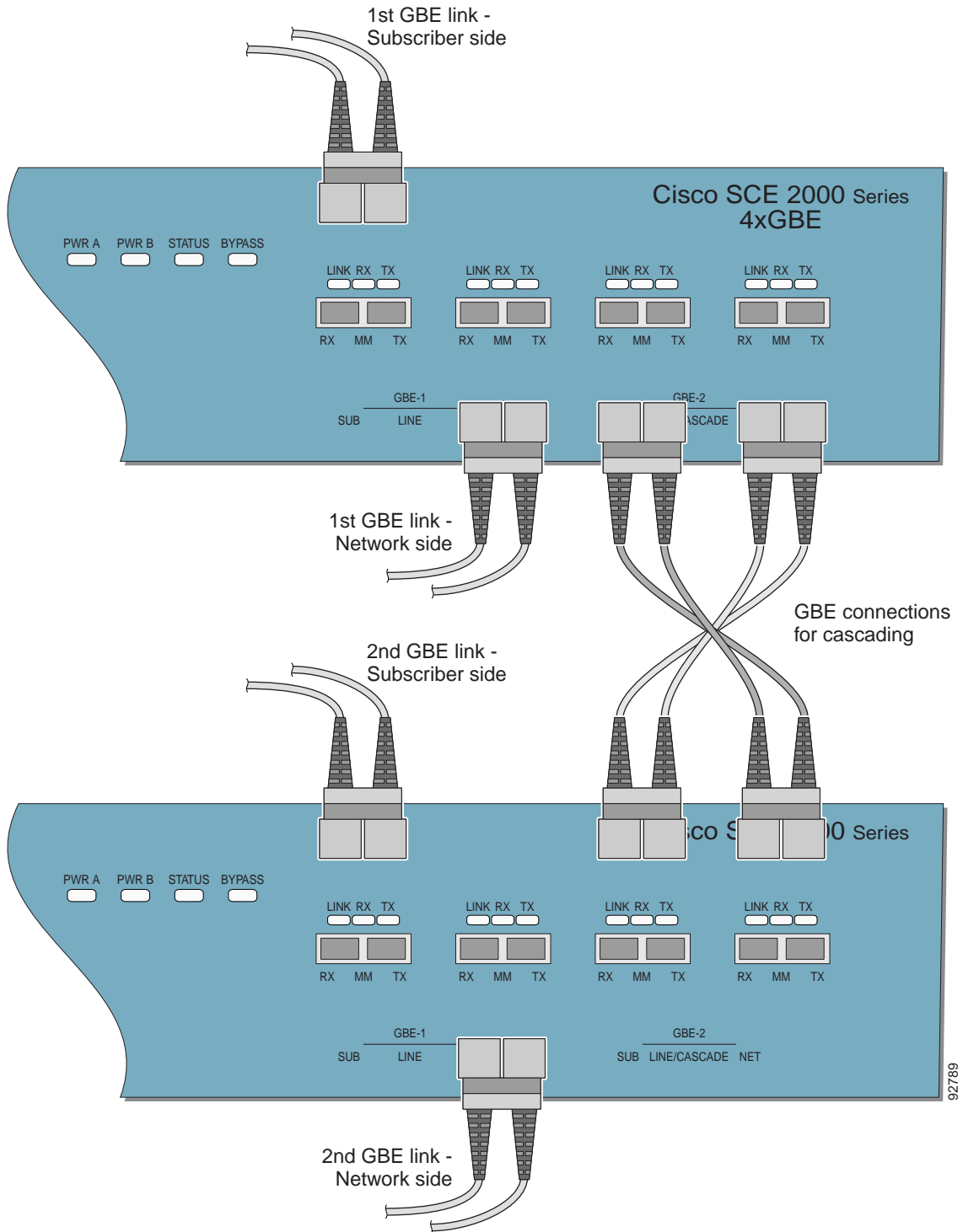
Figure 5-5 Cabling Diagram: Dual Link Inline Topology Two Cascaded SCE Platforms
