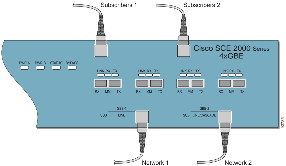
Figure 5-4 Cabling Diagram: Dual Link One SCE Platform Receive-only
