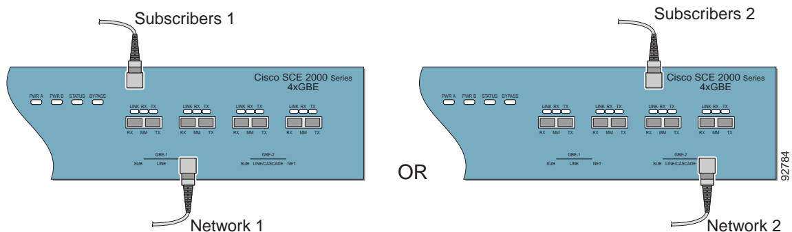
Figure 5-2 Cabling Diagram for Single SCE Platform Single Link Receive-only Topology
