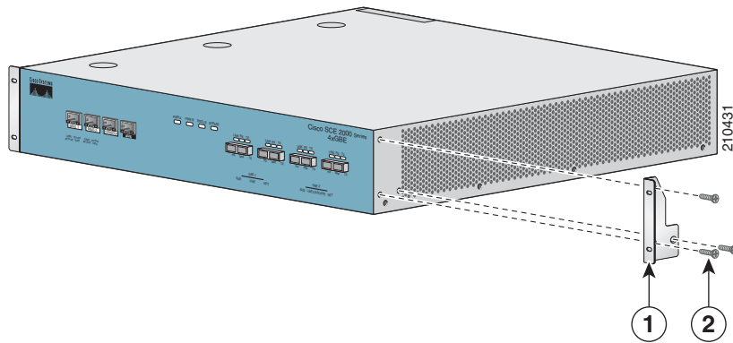
Figure 2-4 Attaching the Mounting Brackets (2-post)
