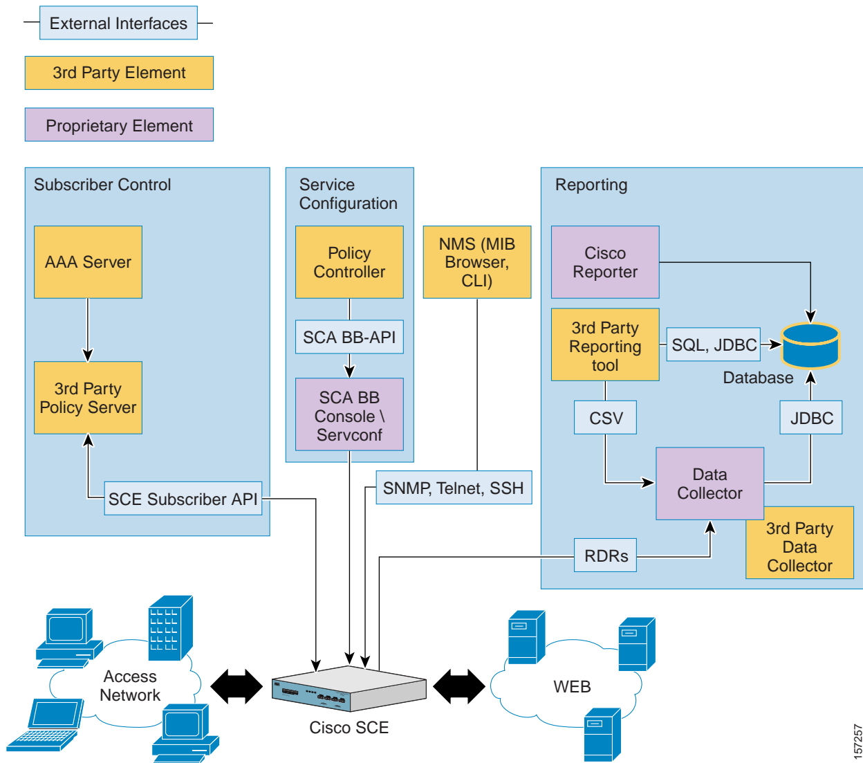
Figure 1-2 Cisco SCA BB Solution Eco System - SM-less integration
