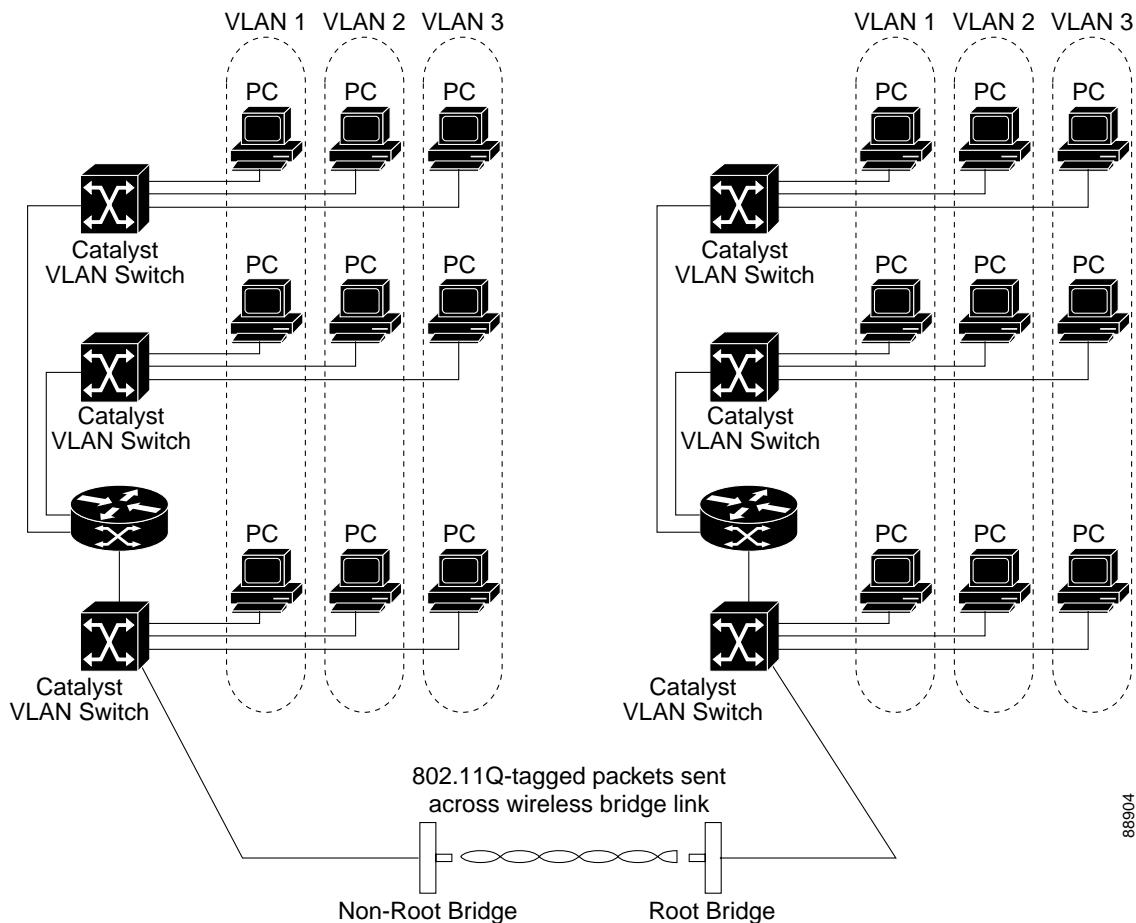
Figure 11-1 Bridges Connecting LAN Segments Using VLANs
