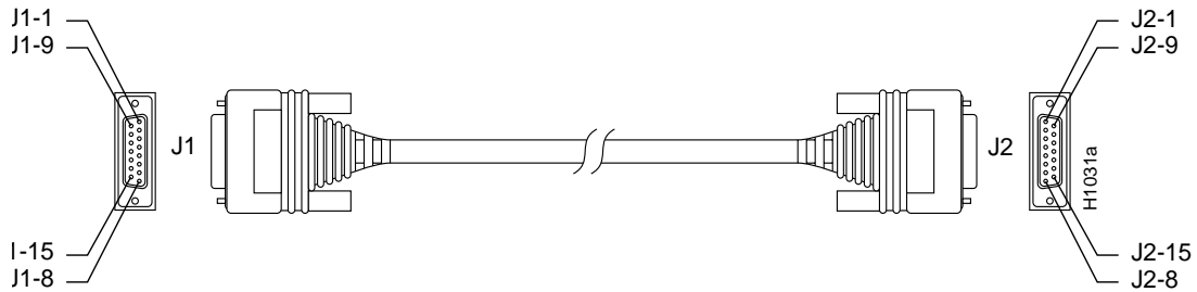
Figure C-6 Ethernet (AUI) Cable Assembly
