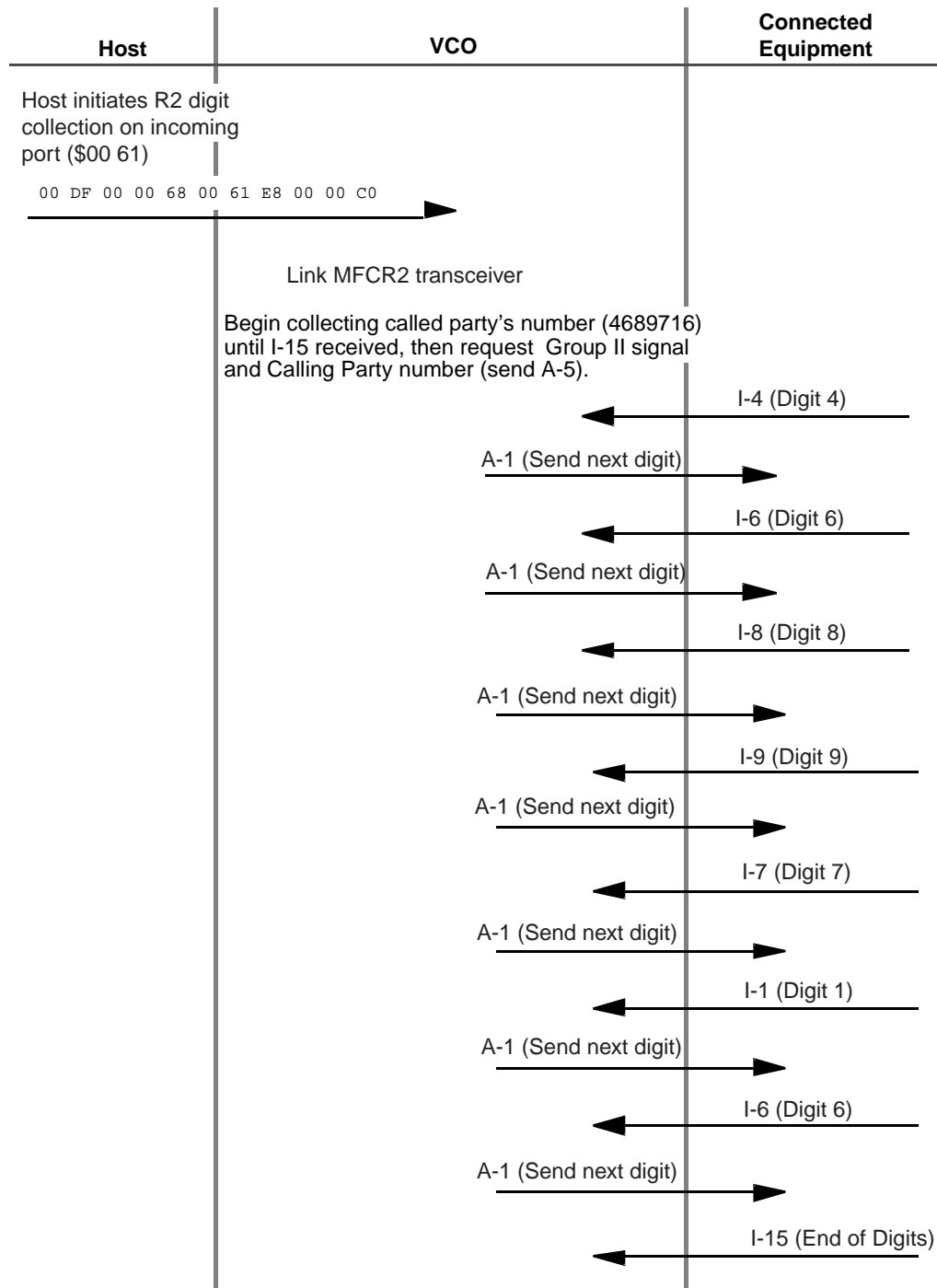
Figure 4-4 Processing Flow for Example #2, Part 1 of 3
