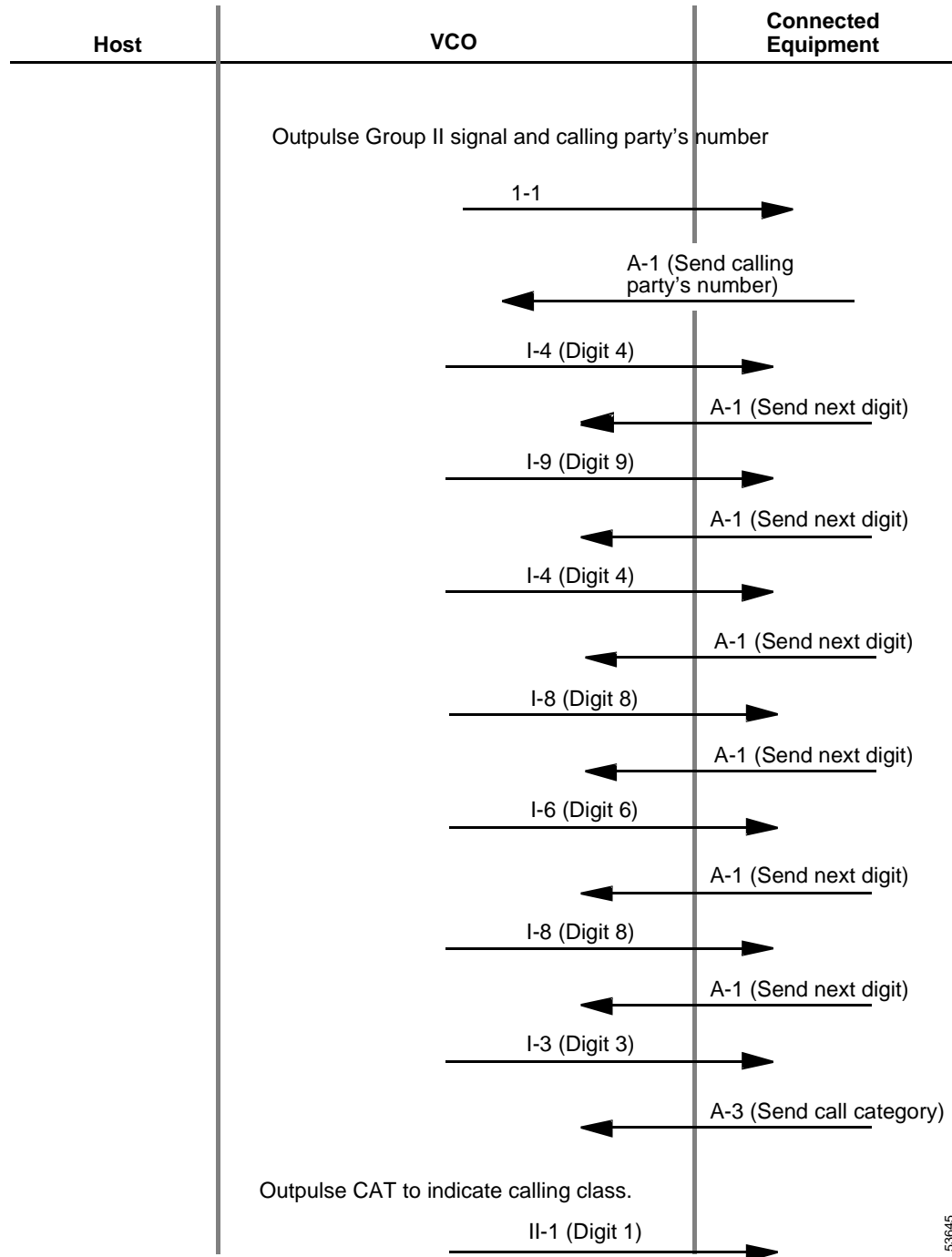
Figure 4-8 Processing Flow for Example #3, Part 2 of 3
