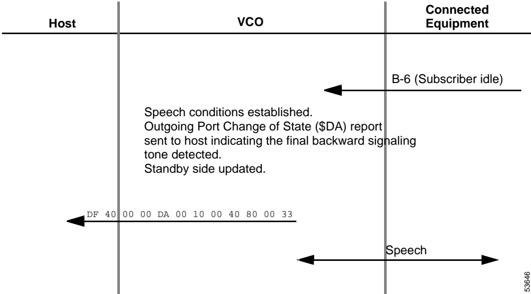
Figure 4-9 Processing Flow for Example #3, Part 3 of 3
