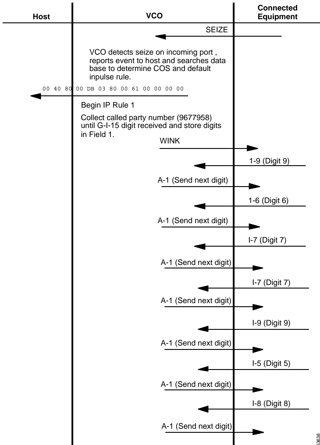
Figure 4-1 Processing Flow for Example #1, Part 1 of 3
