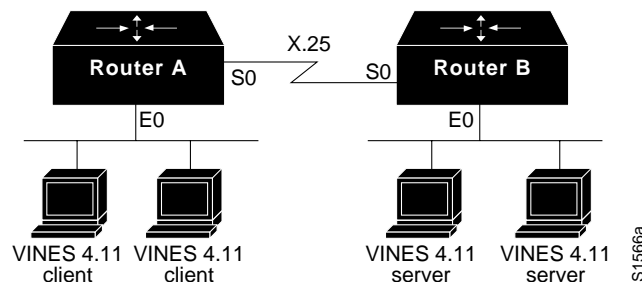
Figure 14-4 VINES Serverless X.25 Configuration
