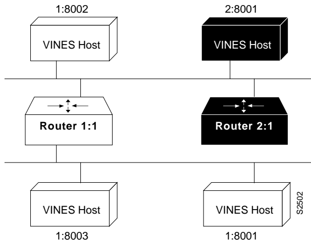
Figure 14-1 VINES Logical Network
