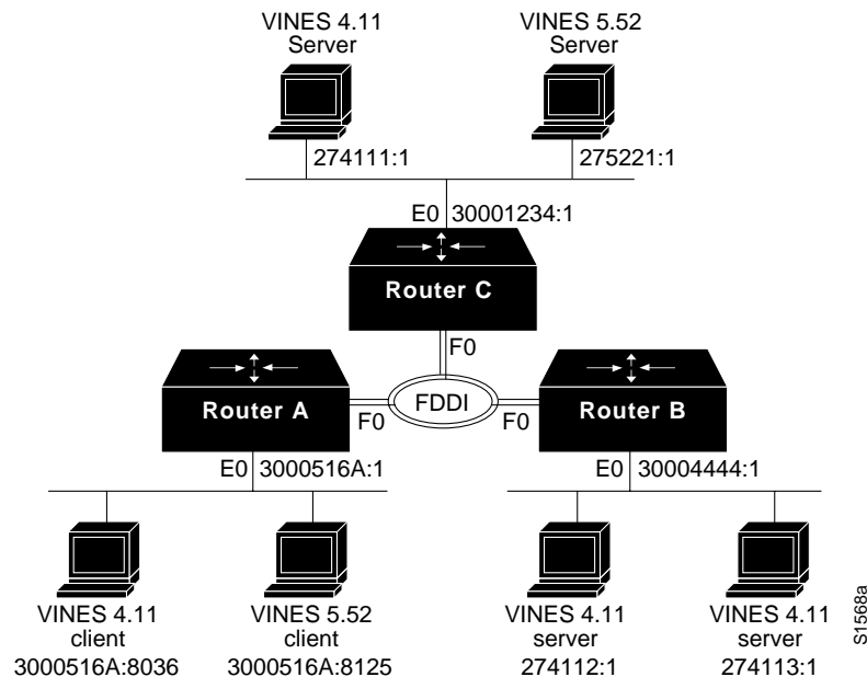
Figure 14-6 VINES Access-List Configuration
