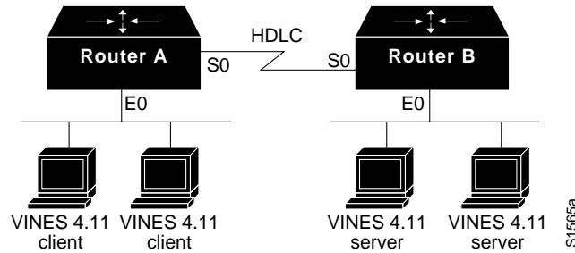
Figure 14-3 VINES Serverless Configuration
