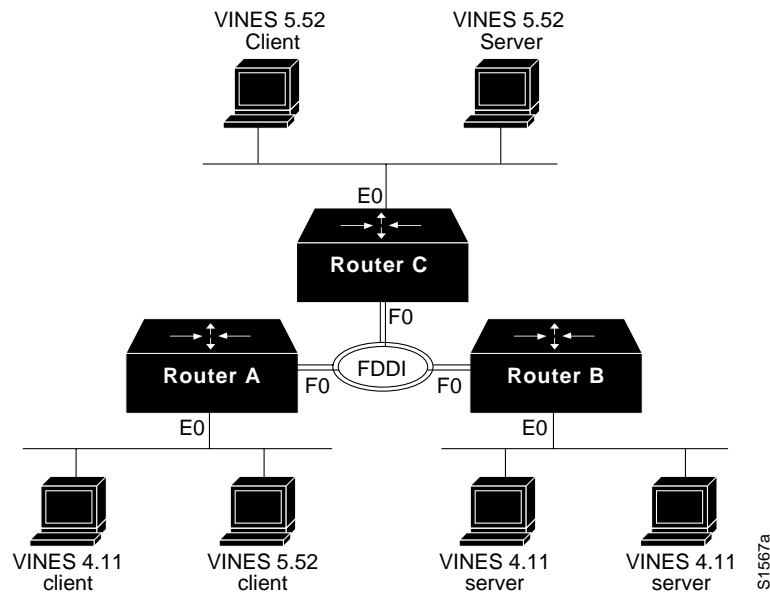
Figure 14-5 VINES Complex Serverless Configuration
