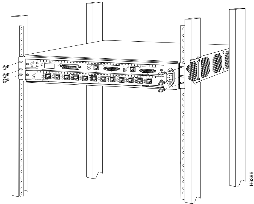
Figure 3-2 Installing the Switch in the Rack
