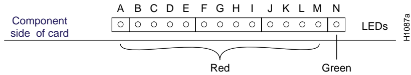
Figure B-12 CSC-R16M LED Indicators—Partial Front-Edge View
