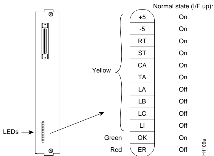
Figure B-15 HSSI Applique (APP-LHS) LED Indicators
