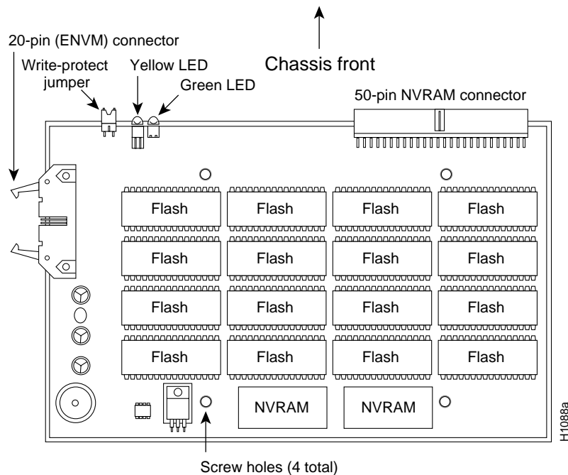
Figure B-10 CSC-MC+ LED Indicators—Component-Side View
