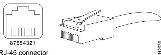
Figure 3 100VG AnyLAN RJ-45 Connections, Receptacle and Plug
