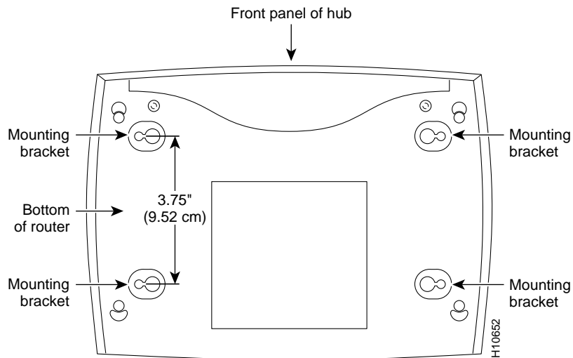
Figure C-1 Wall-Mount Brackets—Bottom of Hub
